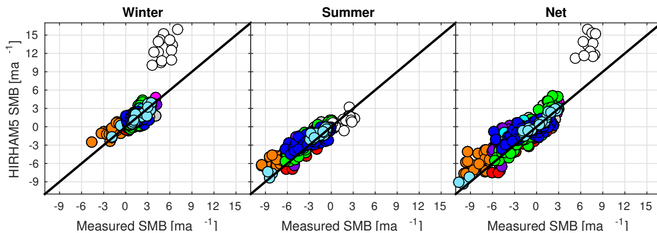
Figure 7. Comparison of SMB measurements from Vatnajökull ice cap from 1995-2014 and HIRHAM5 simulated values. Different colors represent different outlet glaciers, see Fig. 1. The white dots are from a point on Öräfajökull.
