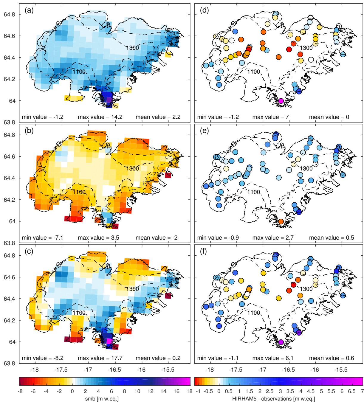
Figure 10. The average (a) winter, (b) summer, and (c) net SMB simulated by HIRHAM5 from the 1980-81 glaciological year to 2013-14. The contour lines marks the approximate placement of the ELA, which generally lies between approximately 1100 and 1300 m elevation. Figures (d)-(f) show the average deviation between model and observations over the observation period for each measurement location for the (d) winter, (e) summer, and (f) whole glaciological year.
