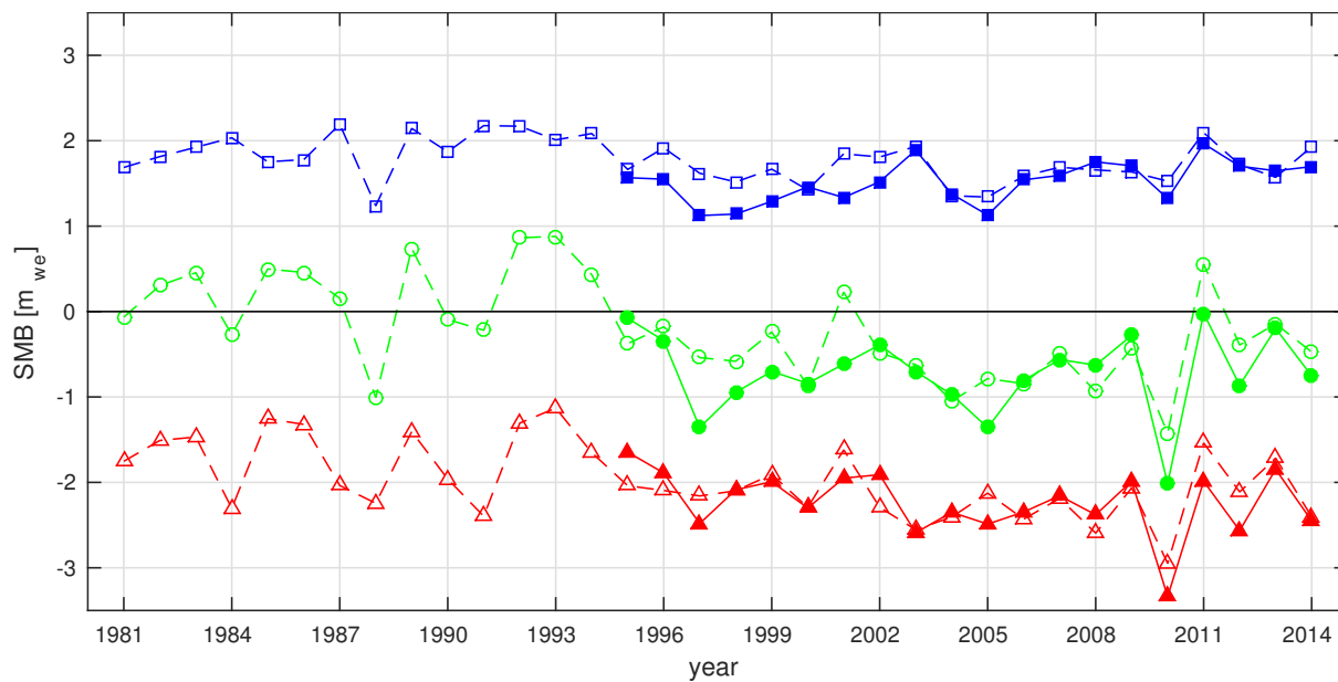
Figure 9. Same as Fig. 8, but corrected at the Öräfajökull area by reducing the HIRHAM5 simulated winter balance with 50%.
