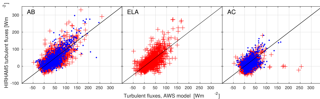
Figure 4. The total turbulent fluxes calculated using the a one-level flux model versus the HIRHAM5 simulated values. Red marks are the data from the Brúarjökull stations, and blue marks are for the Tungnaárjökull stations.
