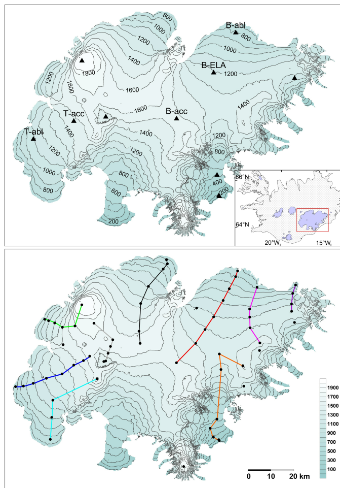
Figure 1. a) the AWS sites and b) mass balance sites from 1995-2014. Not all mass balance sites were measured every year.
