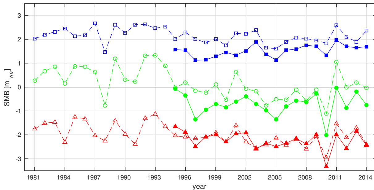
Figure 8. Average summer (red lines), winter (blue lines) and net (green lines) specific surface mass balance for the whole of Vatnajökull. The solid lines are the mass balance of Vatnajökull based on mass balance measurements and manual interpolation, while the dashed lines are the mass balance as simulated by HIRHAM5.
