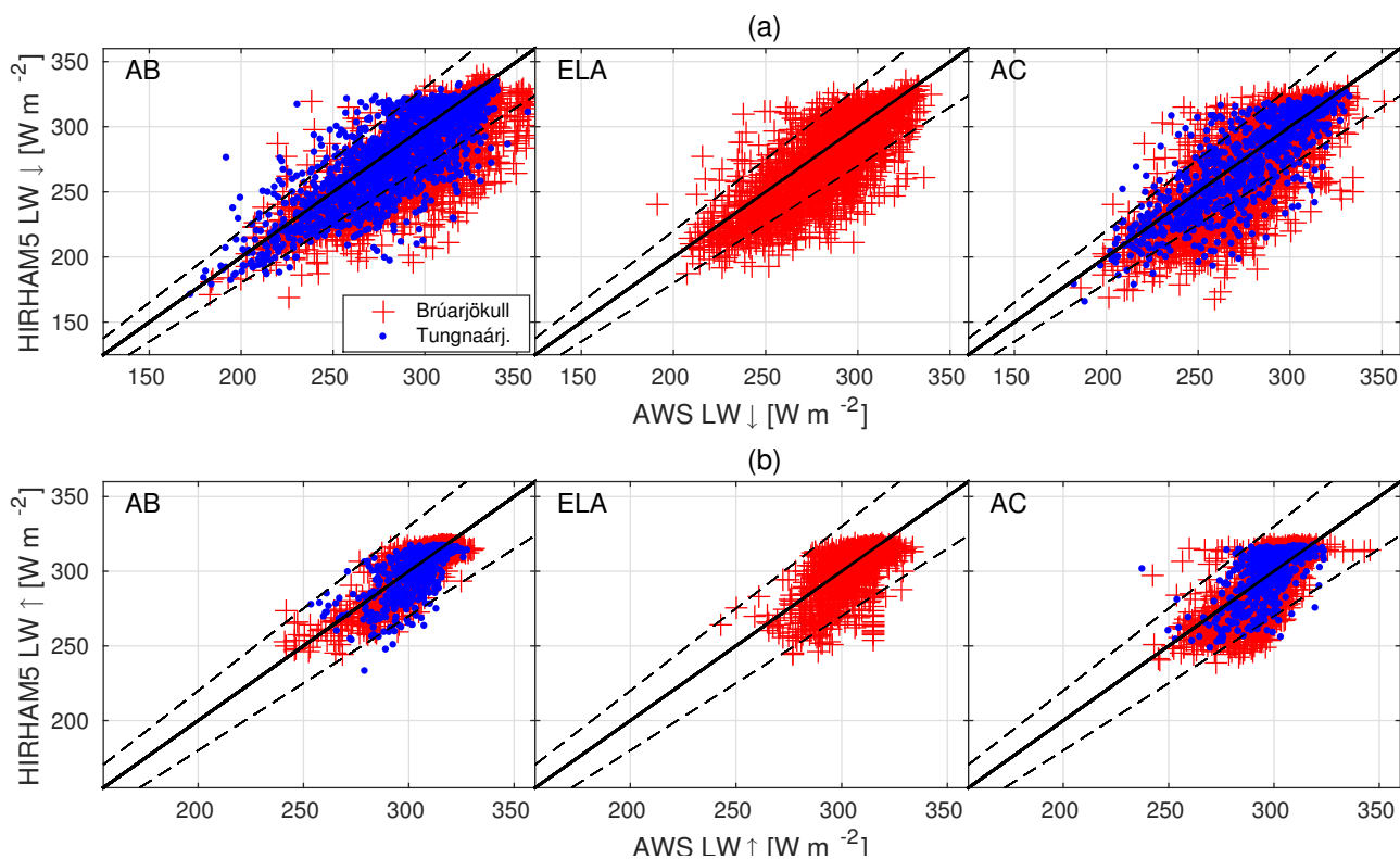
Figure 2. Scatter plots of the measured longwave radiation components, LW_{\downarrow} and LW_{\uparrow} , by stations on Brúarjökull (red) and Tungnaárjökull (blue) versus the LW radiation components simulated by HIRHAM5 at the same locations. The dashed line corresponds to \pm 10\% , i.e. the manufacturer reported uncertainty of the AWS measurements.
