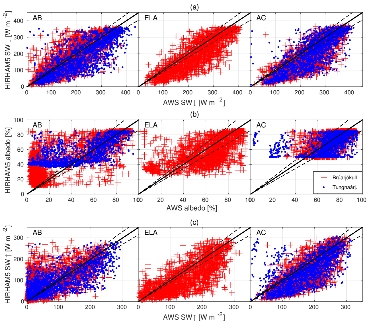
Figure 3. Scatter plots of the measured shortwave radiation components, a) SW ↓ , b) albedo, and c) SW ↑ , by stations on Brúarjökull (red) and Tungnaárjökull (blue) versus the shortwave radiation components simulated by HIRHAM5 at the same locations. The dashed line corresponds to the uncertainty of the measured AWS components.
