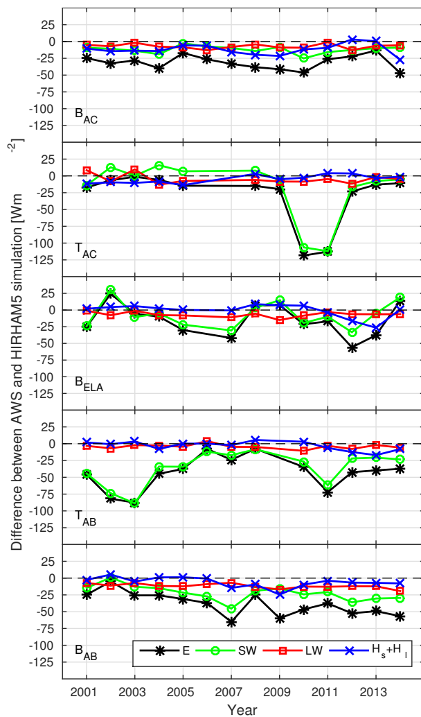
Figure 5. The average summer (Apr-Oct) bias of each energy balance component for the measurement period at each AWS site. The large deviation in the SW radiation at the Tunaárjökull sites in 2010-2011 is due to deposition of ash on the glacier during the 2010 Eyjafjallajökull and 2011 Grímsvötn eruptions.
