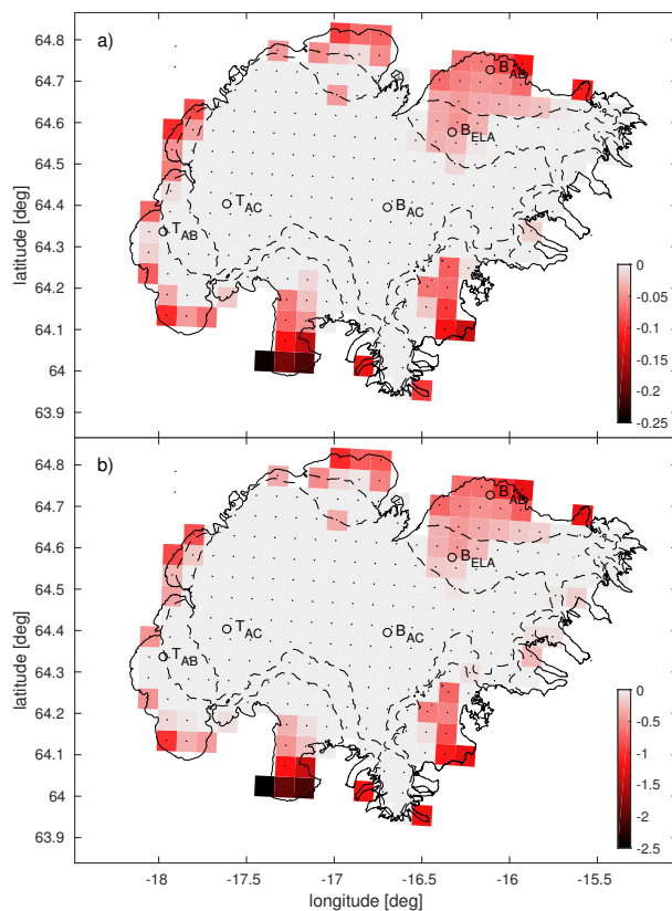
Figure 11. Difference between two runs with HIRHAM5, one using a MODIS bare ice albedo map and the other with a constant ice albedo in a) mean albedo and b) mean annual mass balance in m w.eq. from 2001-2014. The locations of the used AWS are shown with black circles.
