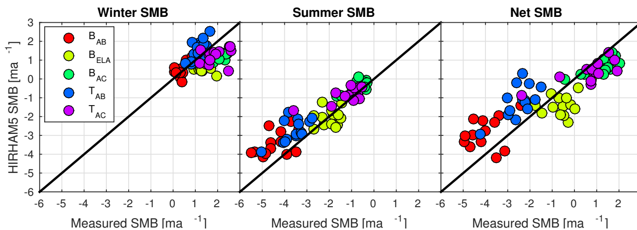
Figure 6. The winter, summer, and net mass balance from 1995-2014 according to mass balance measurements at the five AWS sites and the HIRHAM5 simulation.
