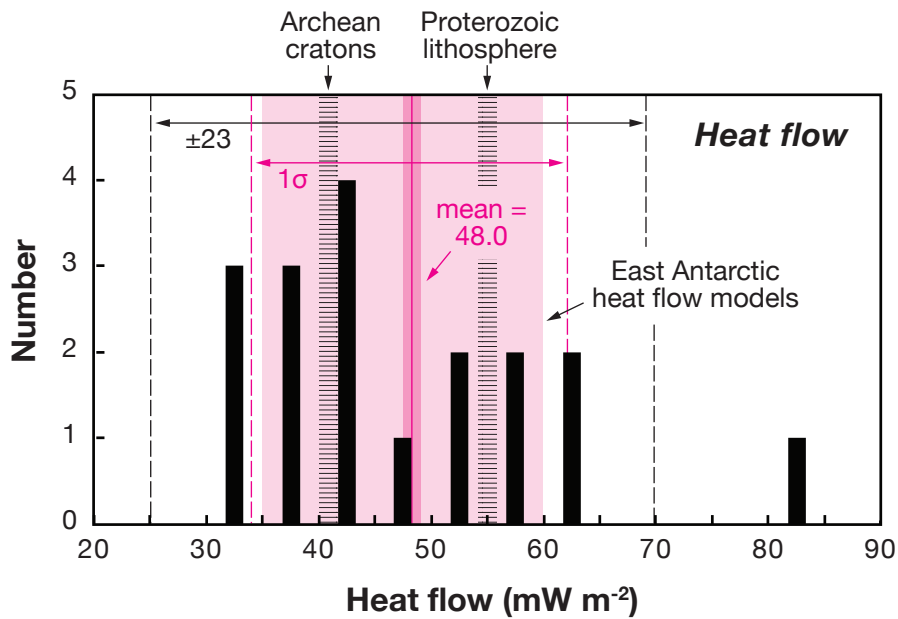
Fig. 5. Figure 5. Histogram of heat flow values estimated from heat production in the glacial clasts.
