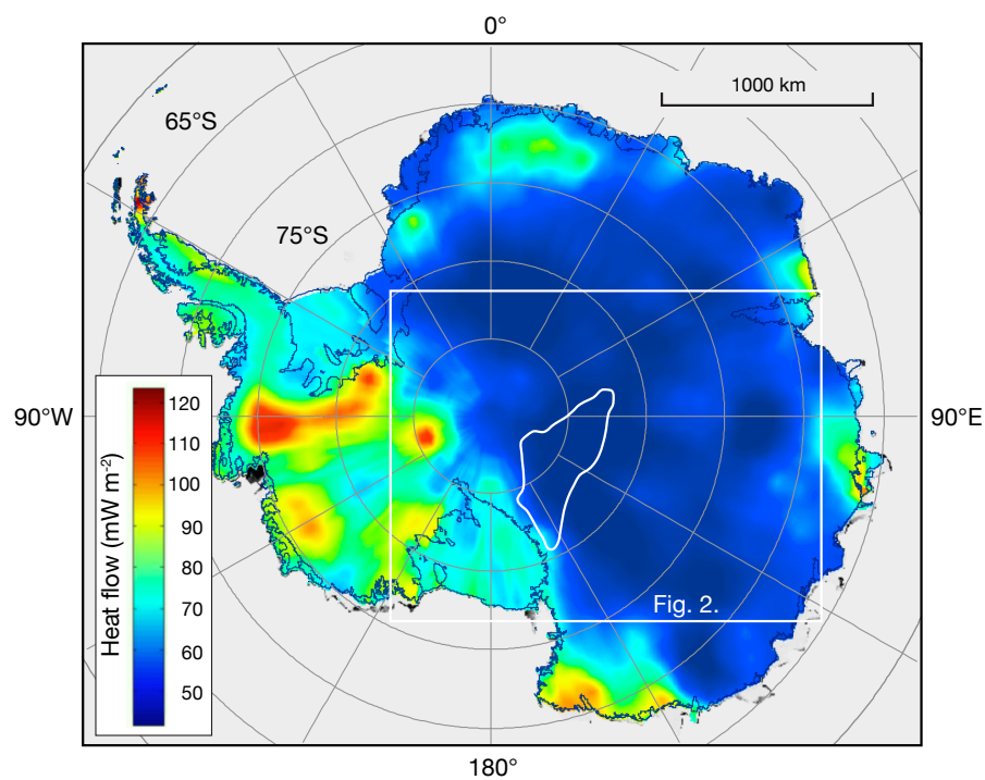
Fig. 1. Figure 1: Terrestrial heat flow in Antarctica.
