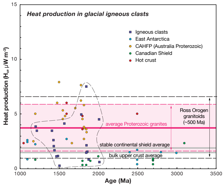
Fig. 4. Figure 4. Plot of surface heat production ( H_0 ) vs. age for igneous glacial clasts.
