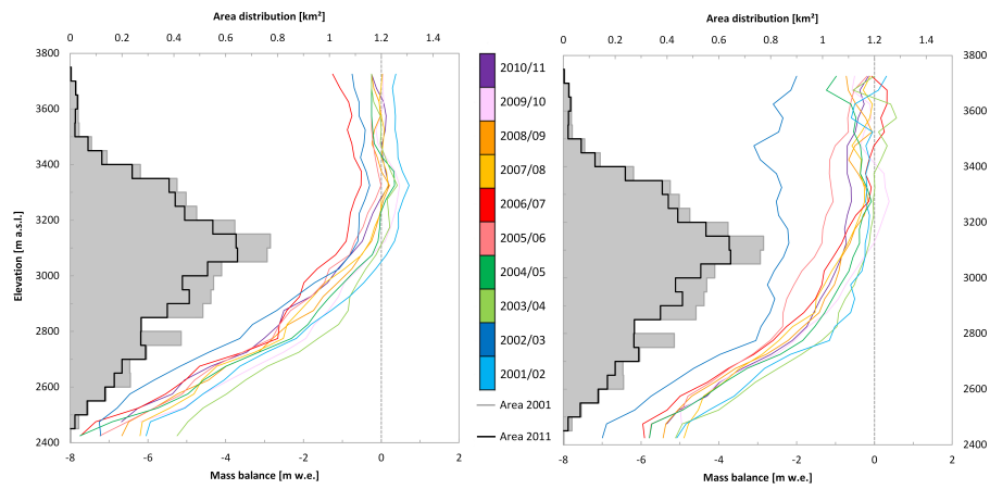
Figure 4. Altitudinal profiles of annual homogenized glaciological (left) and geodetic (right) mass balances over the study period. Note that vertical profiles of the two methods cannot be directly compared due to the effect of glacier dynamics not captured in the glaciological results.
