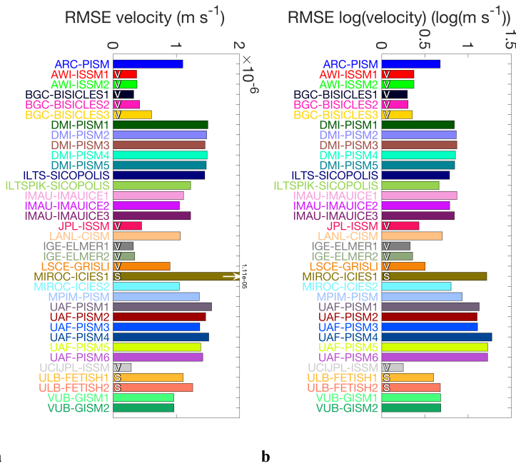
Figure 7 Root mean square error (RMSE) of the horizontal velocity magnitude (a) and the log of the horizontal velocity magnitude (b) compared to observations (Joughin et al., 2016). The diagnostics have been calculated for grid cells subsampled regularly in space to reduce spatial correlation; we show median values for different possible offsets of this sampling.
