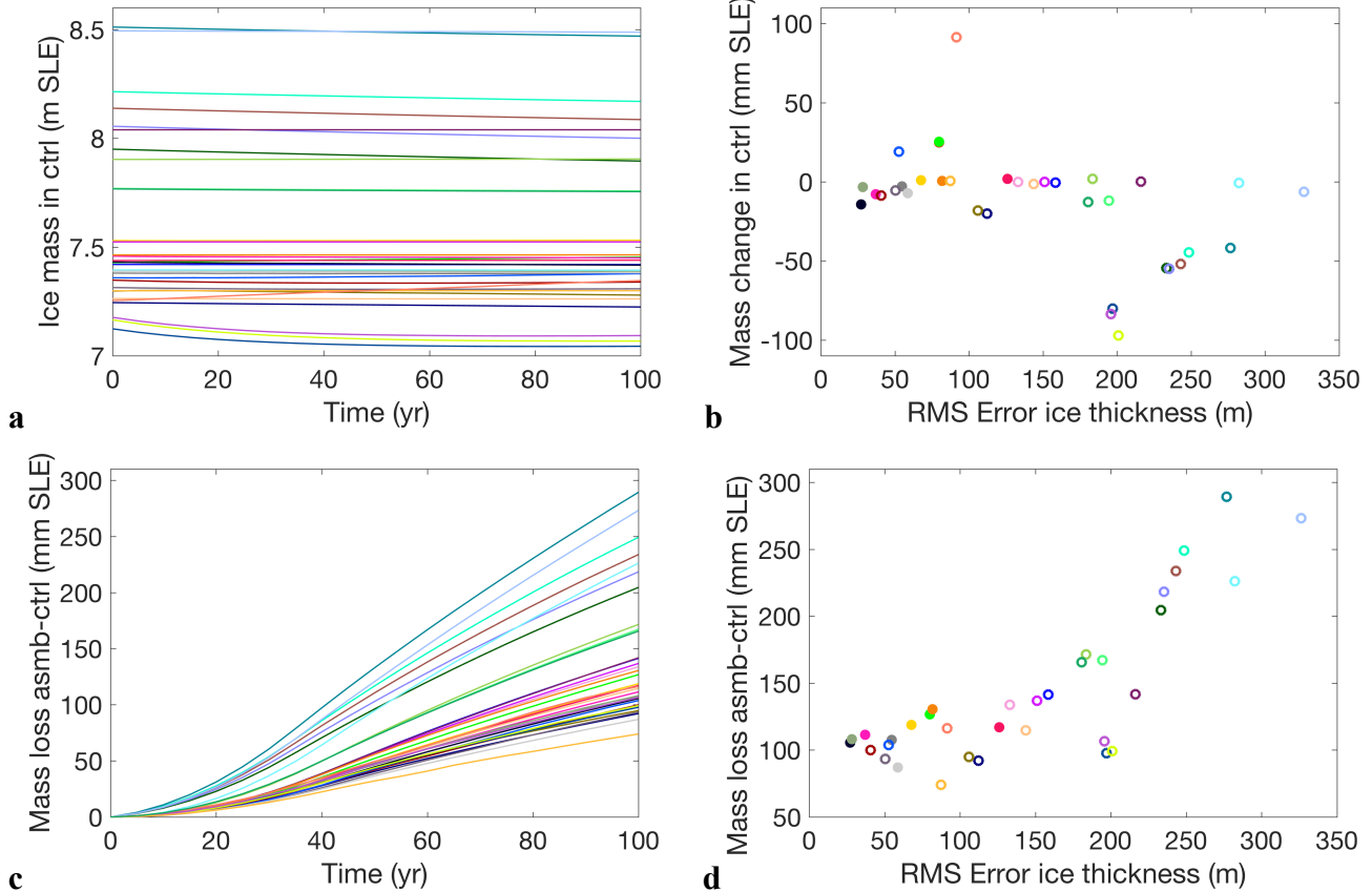
Figure 8 Ice mass evolution in ctrl (a) and ice mass loss from asmb-ctrl (c). Mass change after 100 years in experiment ctrl (b) and from asmb-ctrl (d) related to error in initial ice thickness. Ice volume changes have been converted to sea-level equivalent (SLE) assuming an ocean area of 361.8 \cdot 10^6 \text{ km}^2 and the specific ice density from the individual ice sheet models. Filled symbols in (b) and (d) represent DAV models. Data in (b) and (d) is available in supplementary Table S1.
