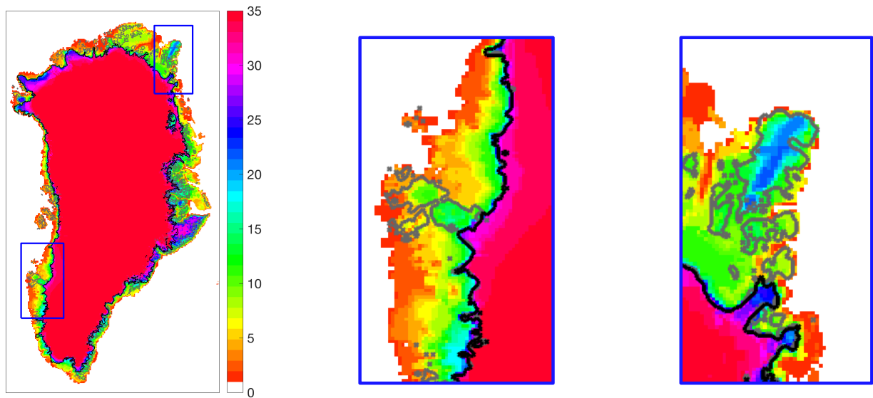
5 Figure 1 Common ice mask of the ensemble of models in the intercomparison. The colour code indicates the number of models (out of 35 in total) that simulate ice at a given location. Outlines of the observed ice sheet proper (Rastner et al., 2012) and all ice-covered regions (i.e. main ice sheet plus small ice caps and glaciers; Morlighem et al. 2014) are given as black and grey contour lines, respectively. A complete set of figures displaying individual model results is given in the supplementary material.
