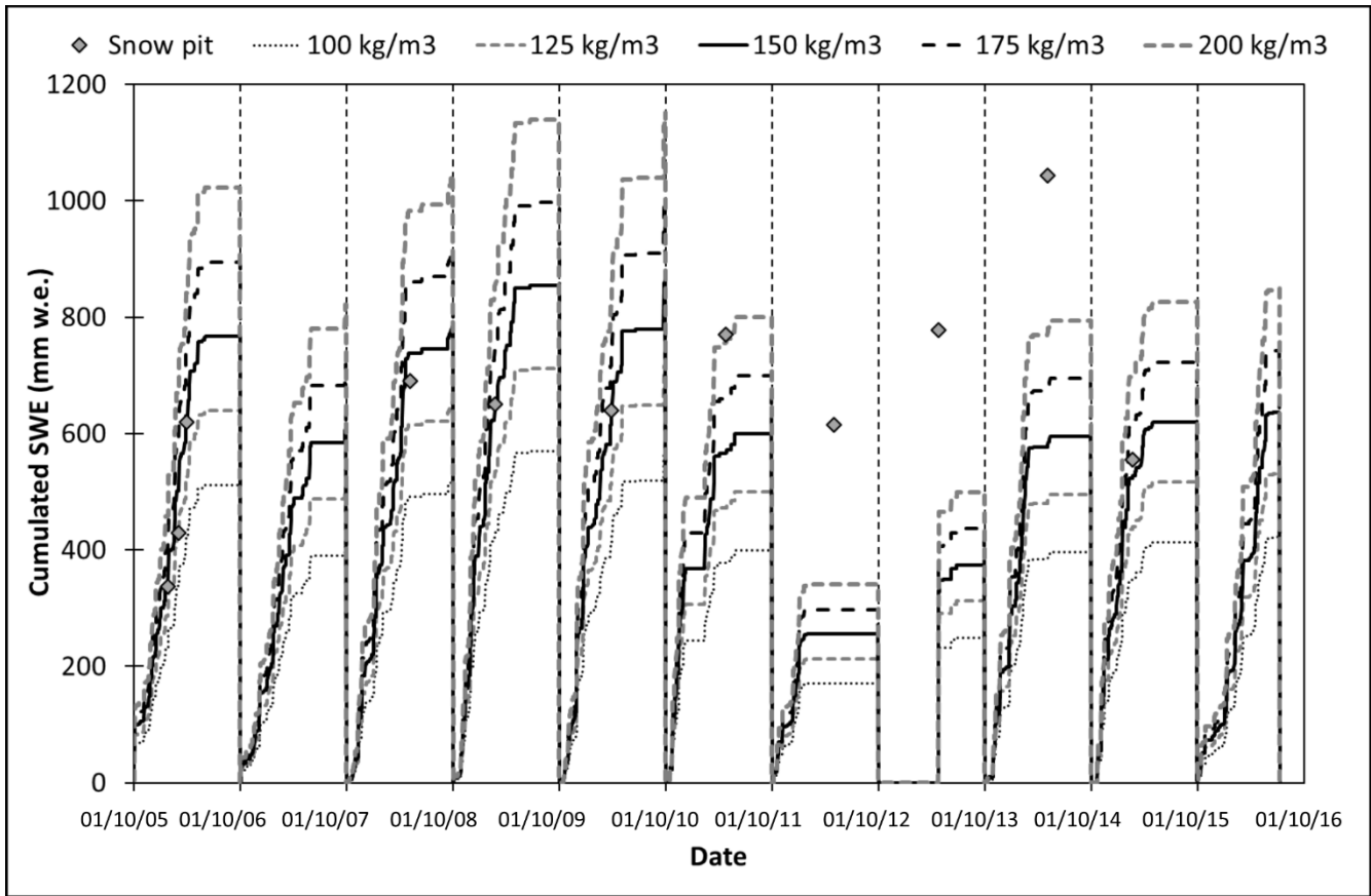
Figure 6: Comparison among daily SWE values derived from snow depth data acquired by SR50 sonic ranger (applying different values of new snow density) and SWE values measured by snow pits from 2005 to 2016. The dates shown are dd/mm/yy.
