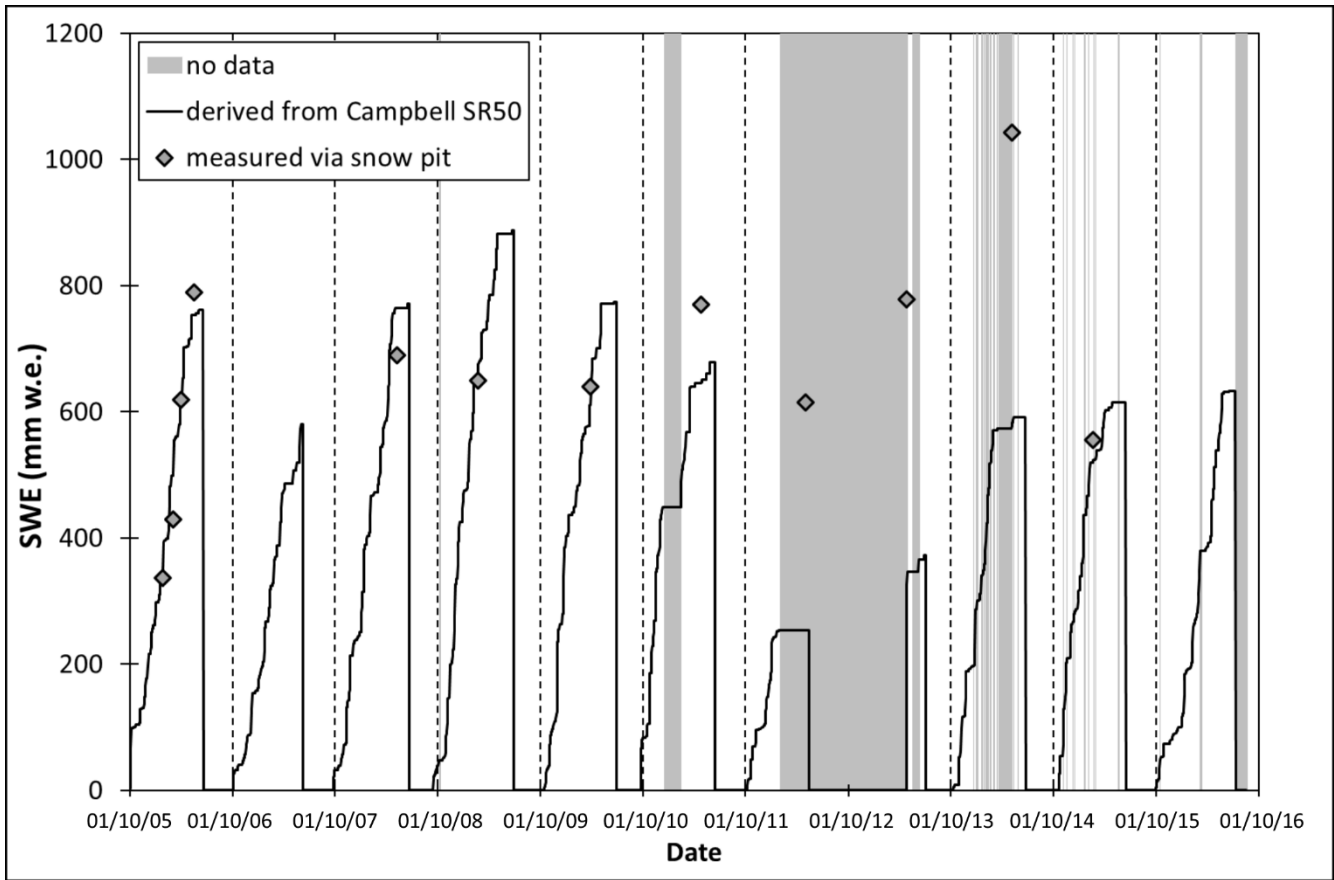
538 Figure 3: Daily SWE data derived from snow depth by the Campbell SR50 (using the new snow density of 149 kg m -3 ) 539 and measured by snow pits from 1 st October 2005 to 30 th September 2016. The periods without data are shown in light 540 grey. The dates shown are dd/mm/yy.
