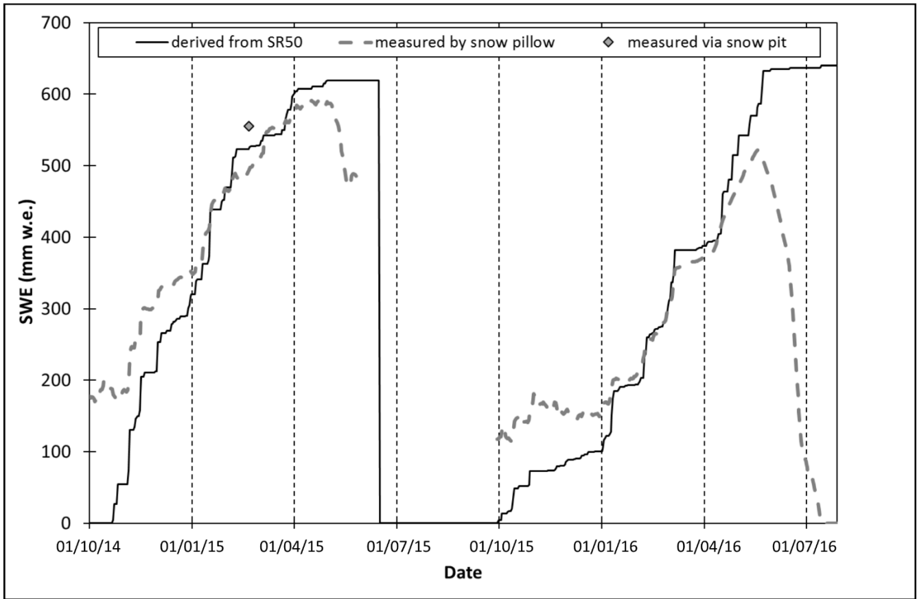
542 543 Figure 4: Daily SWE data derived from snow depth measured by Campbell SR50 (using the new snow density of 149 544 kg m -3 ) and measured by snow pits and snow pillow from October 2014 to July 2016. The dates shown are dd/mm/yy. 545
