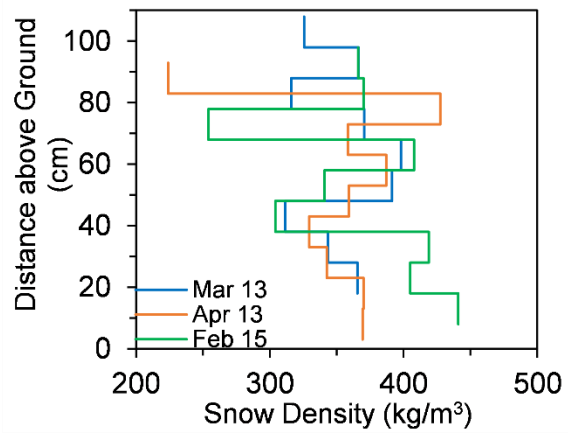
Figure 3: Observations snow density profiles on March 20, 2013; April 7, 2013; and February 20, 2015.
