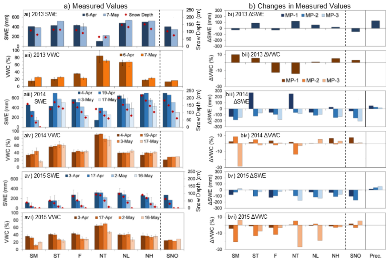
Figure 4: Observations of a) measured values for snow water equivalent (SWE) and near surface soil volumetric water content (VWC) and b) changes in measured values between survey dates for regions of interest: middle of the south aspect hillslope (SM), toe of the south aspect slope (ST), flat aspect (FA), toe of the north aspect slope (NT), low on the north aspect slope (NL), and high on the north aspect slope (NH). Also included are observed values at the SNOTEL site (SNO) that include SWE and precipitation (Precip.). Figure panels display i) 2013 SWE, ii) 2013 VWC, iii) 2014 SWE, iv) 2014 VWC, v) 2015 SWE, and vi) 2015 VWC. Changes are shown for melt period 1 (MP-1) between the first two surveys, melt period 2 (MP-2) between the second and third surveys, and melt period 3 (MP-3) between the third and fourth surveys. Each melt period is 14-15 days with the exception of 2013 that was 28 days. Error bars indicate total range of measurements at locations.
