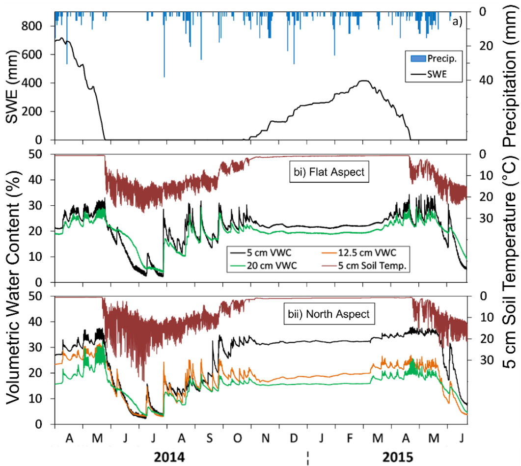
Figure 6: a) Daily snow water equivalent (SWE) and precipitation recorded at the Dry Lake SNOTEL station and b) the hourly soil volumetric water content (VWC) and 5 cm deep temperature at bi) the flat SNOTEL site and bii) the installed sensors on the north aspect slope.
