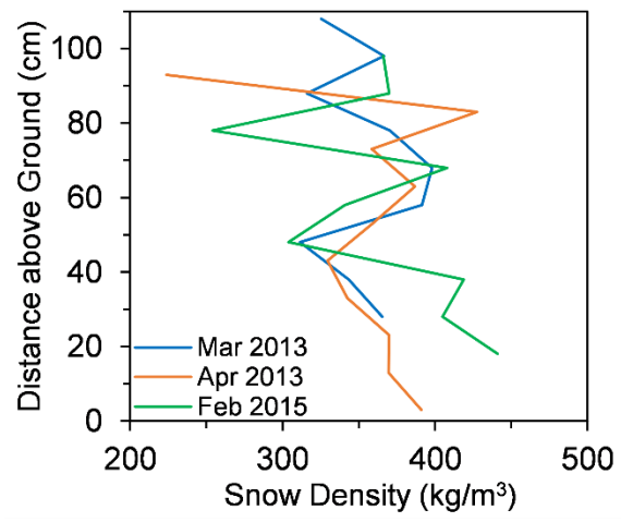
Figure 3: Observations snow density profiles on March 20, 2013; April 7, 2013; and February 20, 2015.
