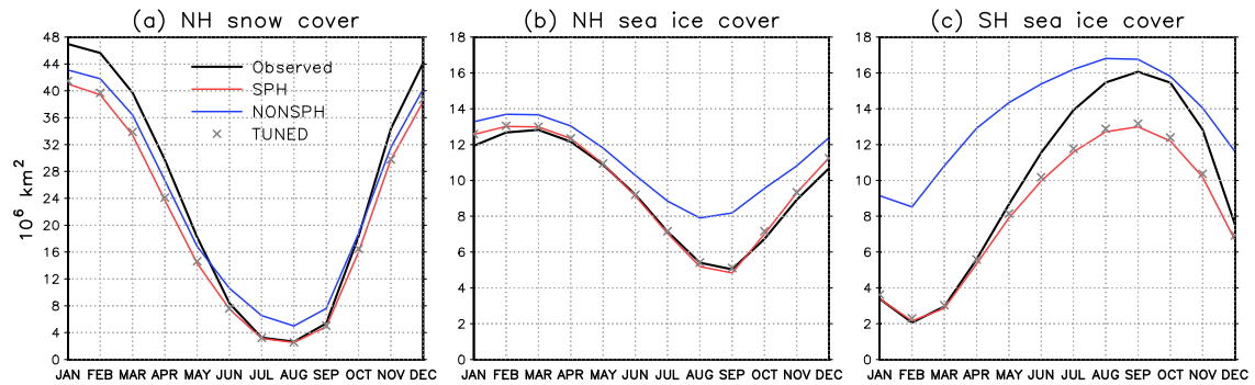
Figure 9. (a) Seasonal cycle of northern hemisphere land snow cover in the NOAA snow cover extent CDR (Robinson et al., 2012; Estilow et al., 2015) (black curve) and in the SPH (red curve), NONSPH (blue curve) and TUNED (crosses) experiments. (b) Northern hemisphere and (c) southern hemisphere sea ice cover in the NSIDC passive microwave sea ice concentration CDR (Meier et al., 2013; Peng et al., 2013) and in the NorESM experiments. For both snow cover and sea ice, the observations are averaged over the years 1990–2014. To account for missing sea ice data in the NSIDC product around the North pole, 0.33 \times 10^6 \text{ km}^2 has been added to the observed values in (b).
