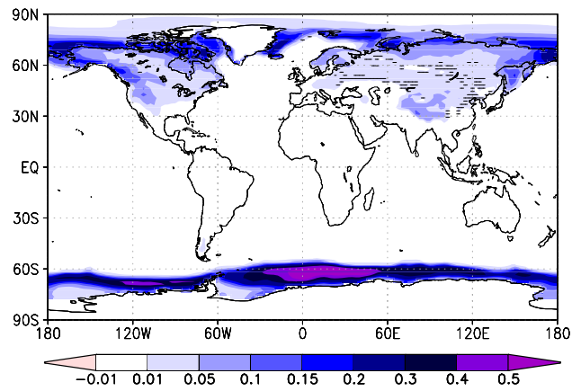
Figure 6. Differences between the NONSPH and SPH experiments in annual-mean snow fraction on land and in sea ice cover. Hatching indicates differences that exceed the limit threshold for colour shading (0.01) but are not significant at the 5% level.
