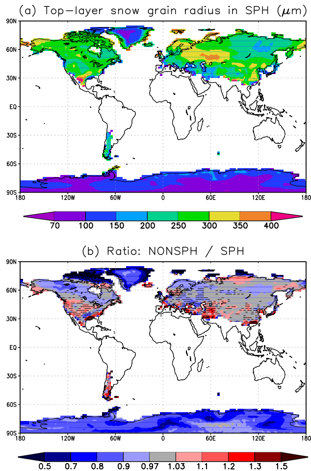
Figure 7. (a) Mean value of snow grain effective radius r_e in the uppermost snow layer on land in the SPH experiment ( \mu\text{m} ) (weighted by snow cover fraction) and (b) The corresponding relative difference (in %) between the ratio of r_e in NONSPH and to that in SPH experiments. Hatching indicates differences ratios that exceed the limit threshold for colour shading (3% i.e., differ from 1 by more than 0.03) but are not significant at the 5% level.
