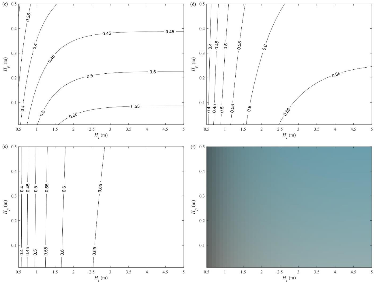
Figure 4: Variations of melt-pond optics and color with pond depth and underlying ice thickness: (a) integrated pond albedo \alpha_B , (b) mean wavelength determined by Eq. (1), (c–e) intensities of red, green, and blue components scaled in the range of 0–1, (f) simulated color of the melt pond in the RGB color space according to the colorimetric method defined by Eqs. (2-6). The sky condition is overcast.
