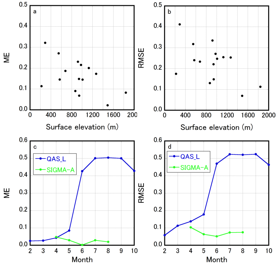
1035 Figure 5: Evaluation of the hourly snow/firn/ice albedo simulated at each AWS (Fig. 1 and Table S7). (a) Mean error (ME) and (b) root mean square error (RMSE) as a function of surface elevation. (c) Monthly changes in ME and (d) monthly changes in RMSE for simulated snow/firn/ice albedo at QAS_L (blue line) and SIGMA-A (green line) during months when the sun appears at each site.
