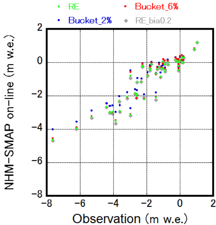
1050 Figure 8: Scatterplot of observed and simulated SMBs during the study period. Observation data 1055 are from stake measurements compiled by PROMICE and ice core measurements from SIGMA- D and SE-Dome. RE indicates the default setting for vertical water movement in snow and firn based on the Richards equation; Bucket_6% and Bucket_2% are alternative settings based on simple bucket schemes with irreducible water contents of 6 % and 2 % of the pore volume; RE_bia0.2 is another alternative setting, where bare ice albedo is set to 0.2, while other configuration is as same as RE.
