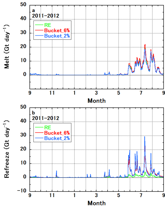
1060 Figure 9: Sensitivity to the choice of vertical water movement scheme of the simulated top 30m integrated (a) melt and (b) refreeze rates for the GrIS during the 2011-2012 mass balance year. RE indicates the default setting for vertical water movement in snow and firn based on the Richards equation; Bucket_6% and Bucket_2% are alternative settings based on simple bucket schemes with irreducible water contents of 6 % and 2 % of the pore volume.
