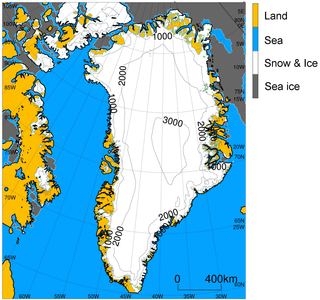
1005 Figure 1: Model domain of NHM-SMAP used in this study showing surface types (colours). The sea ice pattern is depicted for 1 July 2012, and it changes from day to day. Contours on ice sheets and ice caps indicate surface elevation (contour interval 1000 m).
