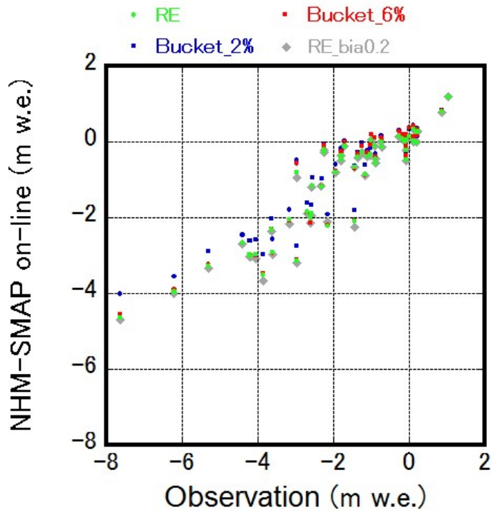
1050 Figure 8: Scatterplot of observed and simulated SMBs during the study period. Observation data 1055 are from stake measurements compiled by PROMICE and ice core measurements from SIGMA-D and SE-Dome. RE indicates the default setting for vertical water movement in snow and firn based on the Richards equation; Bucket_6% and Bucket_2% are alternative settings based on simple bucket schemes with irreducible water contents of 6 % and 2 % of the pore volume; RE_bia0.2 is another alternative setting, where bare ice albedo is set to 0.2, while other configuration is as same as RE.
