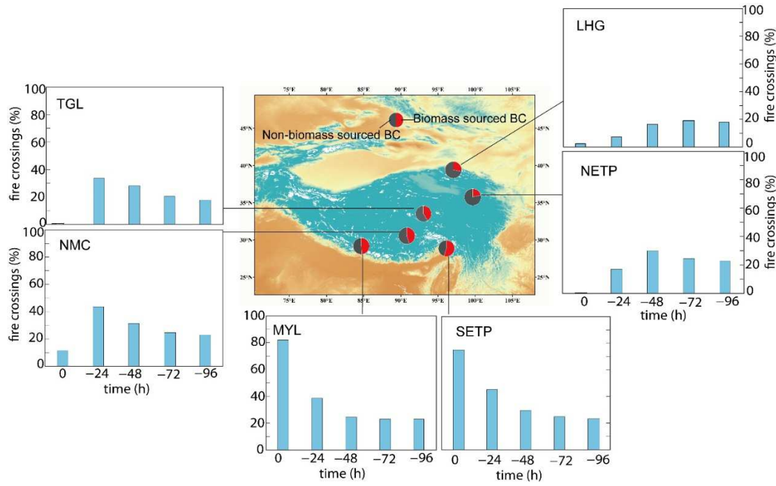
46 Figure 5: Different source contributions to BC deposition on the snow cover of the Tibetan Plateau.
