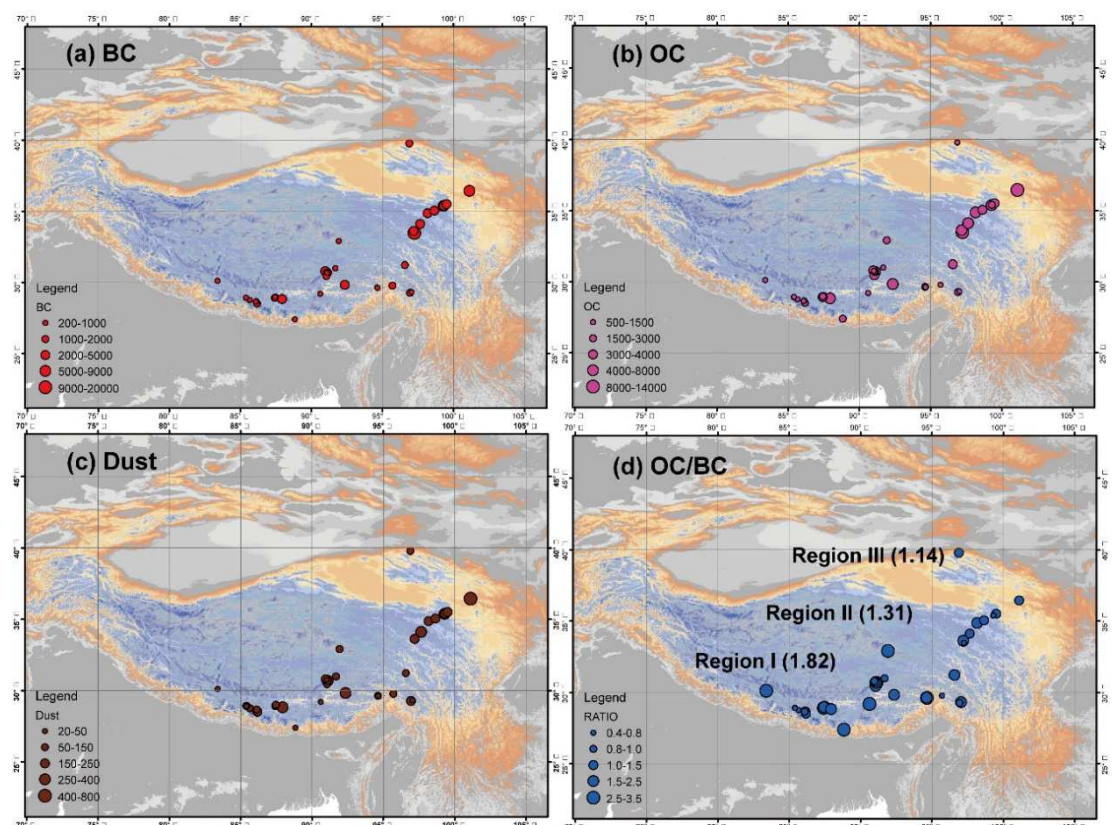
27 28 Figure 2: Spatial distributions of light-absorbing impurities in snow cover for each sampling site over the 29 Tibetan Plateau. (a) BC, (b) OC, (c) Dust, and (d) ratio of OC to BC (OC/BC).
