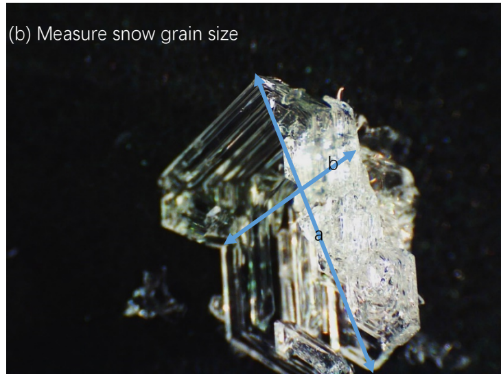
Figure R2. Snow grain size observation in the field (a) and measurement in the lab (b).
