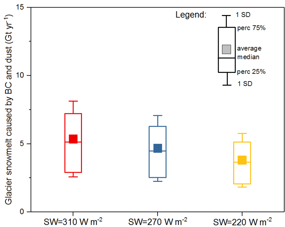
70 71 Figure 9: Estimates of total glacial snowmelt based on daily snowmelt caused by BC and dust for shortwave 72 radiation at 220, 270, and 310 W m -2 , respectively. The days of daily temperature above 0 ° C value is 100 73 (±25 %).
