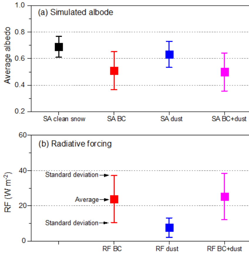
53 54 Figure 7: (a) Average albedo (solid rectangles) of snow cover due to aging only and impurities relative to the 55 clean snow and (b) resulting clear sky instantaneous radiative forcing (solid rectangle means the average). 56 (Note: SA means simulated albedo, SA BC means albedo only with BC in snow, SA dust means albedo only 57 with dust in snow, and SA BC+dust means albedo with BC and dust in snow. RF means radiative forcing, 58 RF BC means the RF caused by BC in snow, RF dust means the RF caused by dust in snow, and RF 59 BC+dust means the RF caused by BC and dust in snow. The solid rectangles are the central average estimate 60 whereas the bars show the standard deviation range of albedo and RF)
