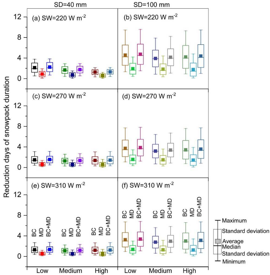
62 63 Figure 8: Reduction in days of snow cover duration by BC and dust for low, medium and high scenarios due 64 to albedo reduction at different snow depth (SD=40 and 100 mm, respectively). a and b were simulated 65 based on the daily shortwave at 220 W m -2 . c and d were simulated based on the daily shortwave at 270 W 66 m -2 , e and f were simulated based on the daily shortwave at 310 W m -2 . (Solid rectangles are average 67 values; solid line in the box means the median; outliers of boxes are the one standard deviations of the 68 average; and the bars are maximum and minimum values.)
