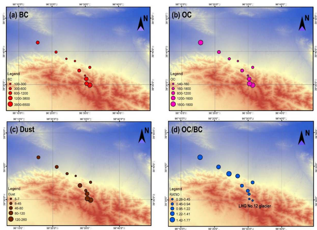
32 Figure 3. Spatial distributions of light-absorbing impurities in snow at the Laohugou region. (a) BC, (b) OC, 33 (c) Dust, and (d) ratio of OC to BC (OC/BC).
