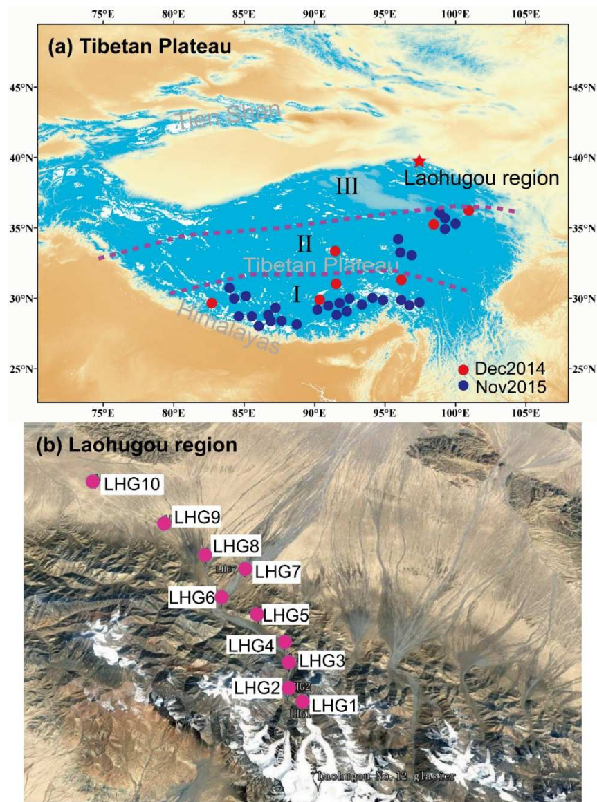
25 Figure 1: Snow sampling sites over (a) the Tibetan Plateau and (b) the Laohugou region.
