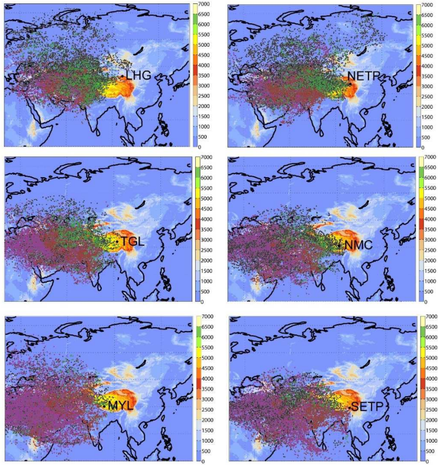
36 Figure 4: Footprint analyses for six selected sites over the Tibetan Plateau during the winter season (Nov 37 2015-Feb 2016). LHG and NETP in the northern Tibetan Plateau (Region III), TGL and NMC in the 38 central Tibetan Plateau (Region II), and MYL and SETP in the southern Tibetan Plateau (Region I). (The 39 right color bar means the height (m a.s.l.). The trajectories starting below 500 hPa were taken into account. 40 Black dots: the air parcel did not pass near a fire during the 96 h prior to arrival at the studied site; Green 41 dots: the air parcel did pass by a fire between -96 h and -48 h, but not afterwards, i.e., the 'contact' to a fire 42 lies back at least 48 h before the air parcel arrived at Renlongba glacier; Magenta dots: contact with fires 43 occurred between -48 h and 0 h before arriving at site; Red dots: contact with a fire before and after -48 h.)
