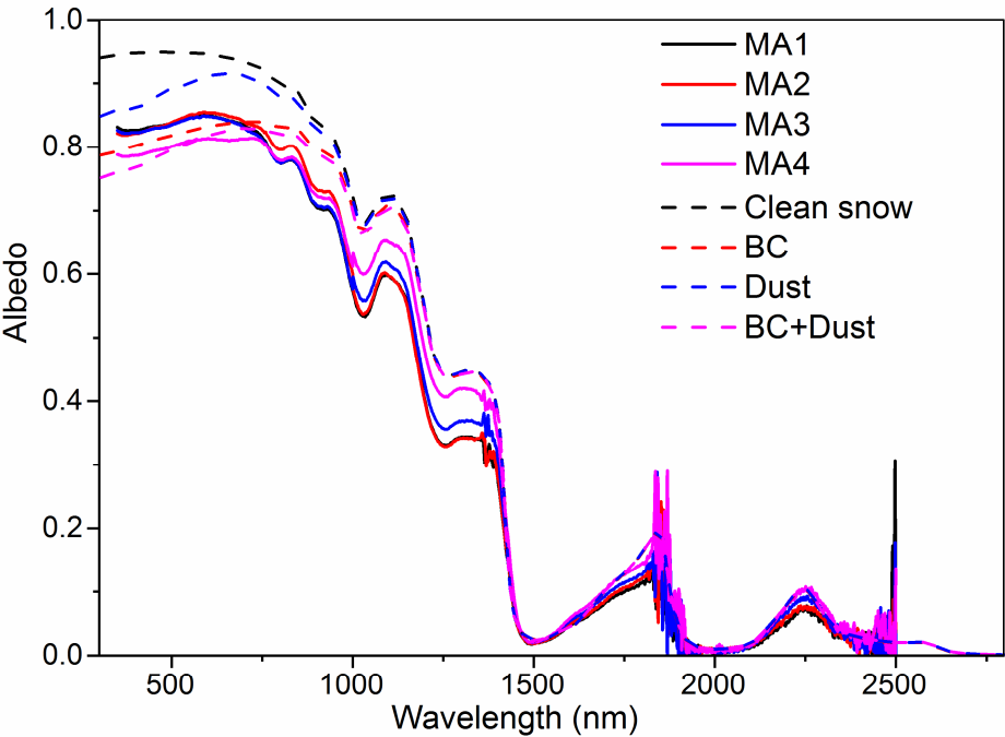
48 49 Figure 6: Measured albedo by ASD (solid lines, MA1-4) and simulated effects of BC and dust on albedo 50 (dashed lines) at the selected snow site on the Tibetan Plateau.
