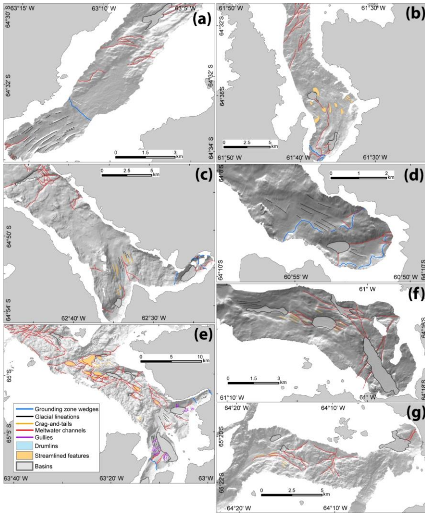
Figure 13. Interpretation of geomorphic features with hillshade as background in western Antarctic Peninsula bays: (a) Fournier Bay, (b) Charlotte Bay, (c) Andvord Bay, (d) Cierva Cove, (e) Flandres Bay, (f) Brialmont Cove, and (g) Collins Bay. Multibeam data shown in figures 2-7.
