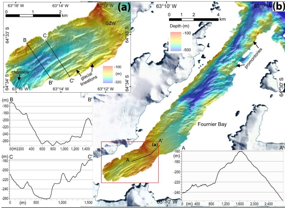
Figure 15. Multibeam bathymetry map of Fournier Bay. Vertical exaggeration is 5x in (a) and 3x in (b).
