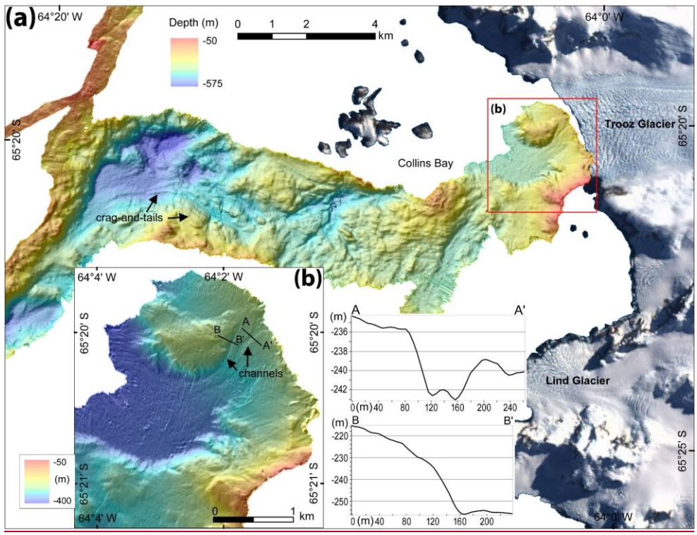
Figure 19. Multibeam bathymetry map of Collins Bay. Vertical exaggeration is 3x in (a) and 2x in (b).
