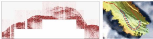
Figure 7. CHIRP facies showing seafloor lithology. Five facies were identified throughout the bay, in addition, two localized examples of features are shown: (a) drumlin and (b) glacial lineations near the modern ice front. The blue rectangle in multibeam example shows the location of the chirp example shown
