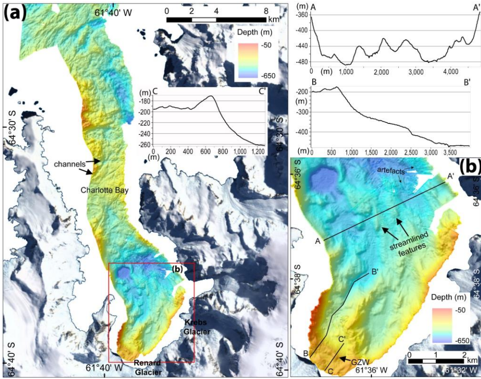
Figure 16. Multibeam bathymetry map of Charlotte Bay. Vertical exaggeration is 5x in (a) and (b).
