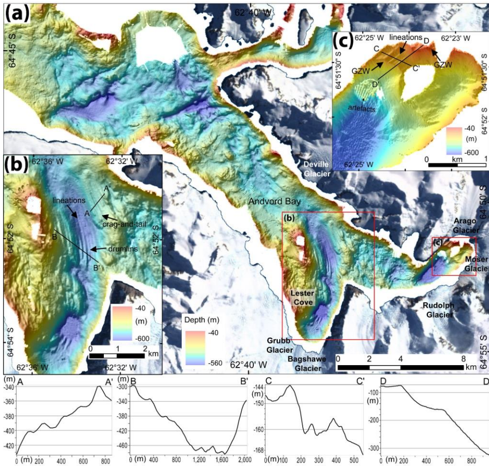
Figure 17. Multibeam bathymetry map of (a) Andvord Bay, (b) Lester Cove, and (c) Moser Glacier Cove. Vertical exaggeration is 5x in all images.
