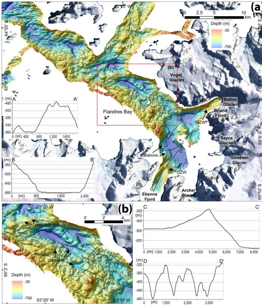
Figure 18. Multibeam bathymetry map of Flandres Bay, Briand Fjord, and Etienne Fjord. Vertical exaggeration is 5x in (a) and (b).
