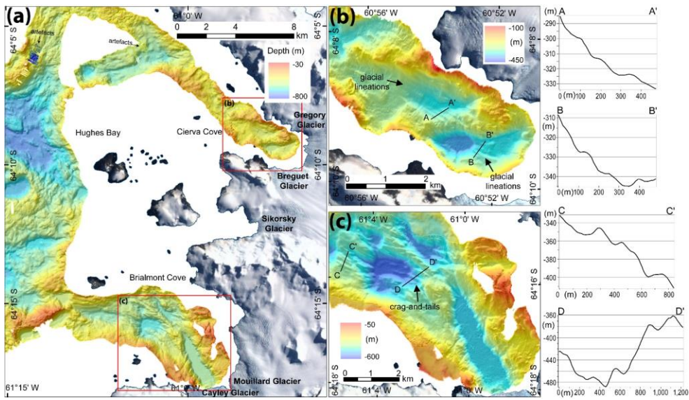
Figure 14. Multibeam bathymetry map of Hughes Bay, (b) Cierva Cove, and (c) Brialmont Cove. Vertical exaggeration is 3x in (a), and 5x in (b) and (c).
