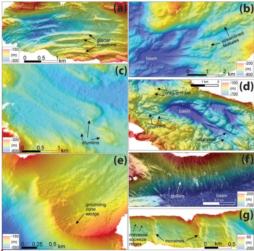
5 Figure 6. Seafloor landforms found in the bays of the western Antarctic Peninsula: (a) glacial lineations, (b) streamlined features and basin, (c) drumlins, (d) crag-and-tails, meltwater channels, and basin, (e) grounding zone wedge, (f) gullies and basin, (g) moraines and crevasse squeeze ridges.
