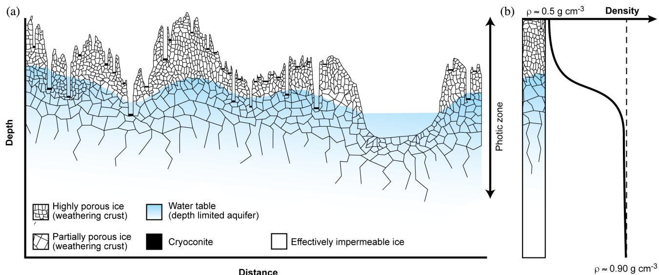
Fig. 1. (a) Conceptual diagram of weathering crust structure, highlighting the porous ice layers, cryoconite holes, and saturated water table (adapted from Irvine-Fynn and Edwards, 2014 and Müller and Keeler, 1969). (b) Theoretical sub-surface depth-density profile showing the non-linear increase in ice density from the highly porous, low density near-surface ice to higher-density, unweathered glacier ice (adapted from LaChapelle, 1959).
