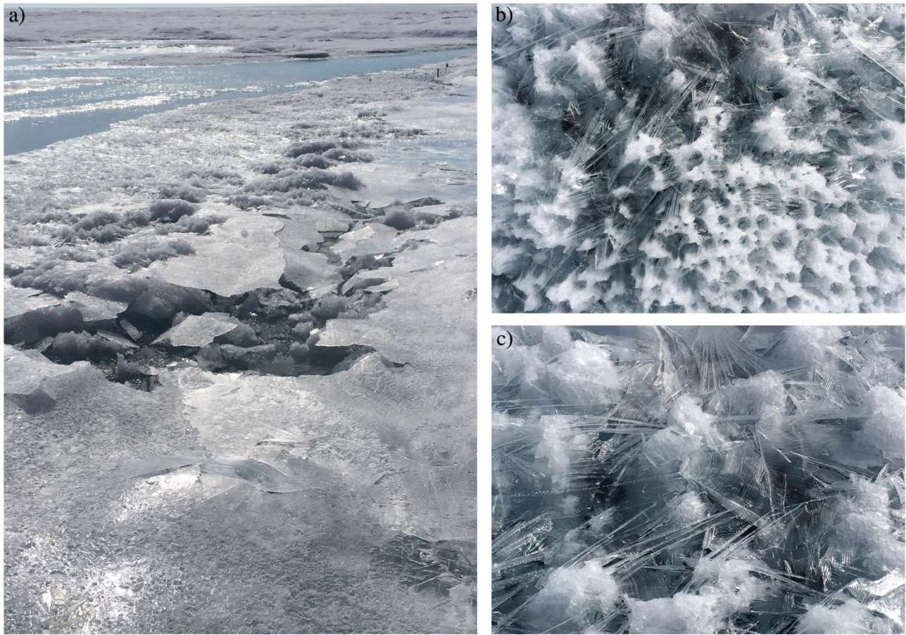
Fig. 9. Night-time refreezing of meltwater at the surface of a) water tracks (~10 m length scale), and b) cryoconite holes (~0.1 – 1 m length scale) was frequently observed during the field study. Photos were collected by the first author during the 6 July – 12 July 2016 field campaign between 04:00 and 07:00 local time.
