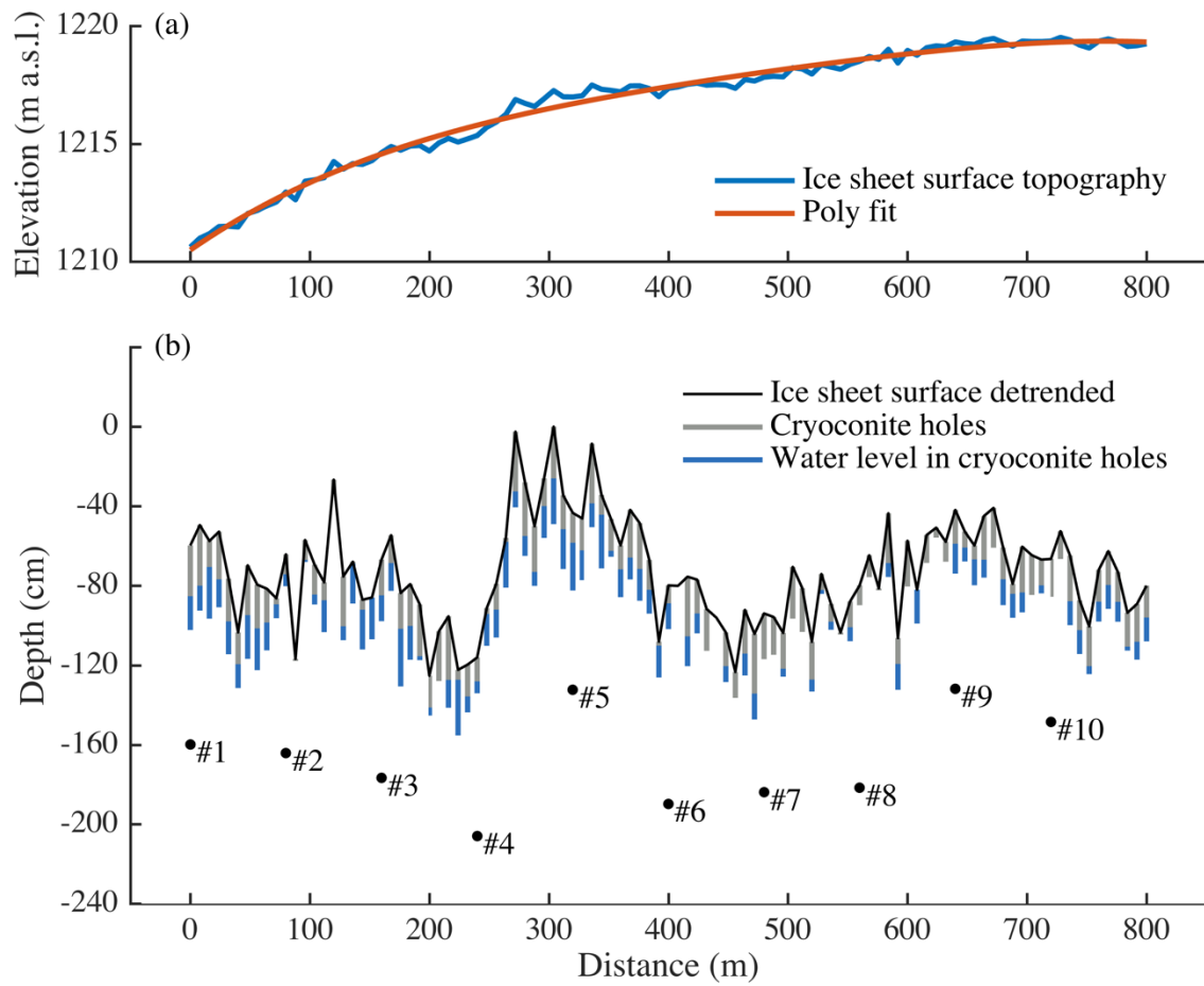
Fig. 7. (a) Ice sheet surface topography along the 800 m study transect extracted from a 6 cm resolution stereo-photogrammetric digital elevation model derived from RGB imagery collected 10 July 2016 from a quad-copter drone and the 2 nd -order polynomial best fit. (b) Ice sheet surface topography detrended with the polynomial best fit, cryoconite hole depths (vertical grey bars), and cryoconite hole water levels (vertical blue bars) sampled along the 800 m study transect, adjusted to a common vertical reference. Locations of the 10 shallow boreholes and their depth relative to the detrended surface are labelled #1-10.
