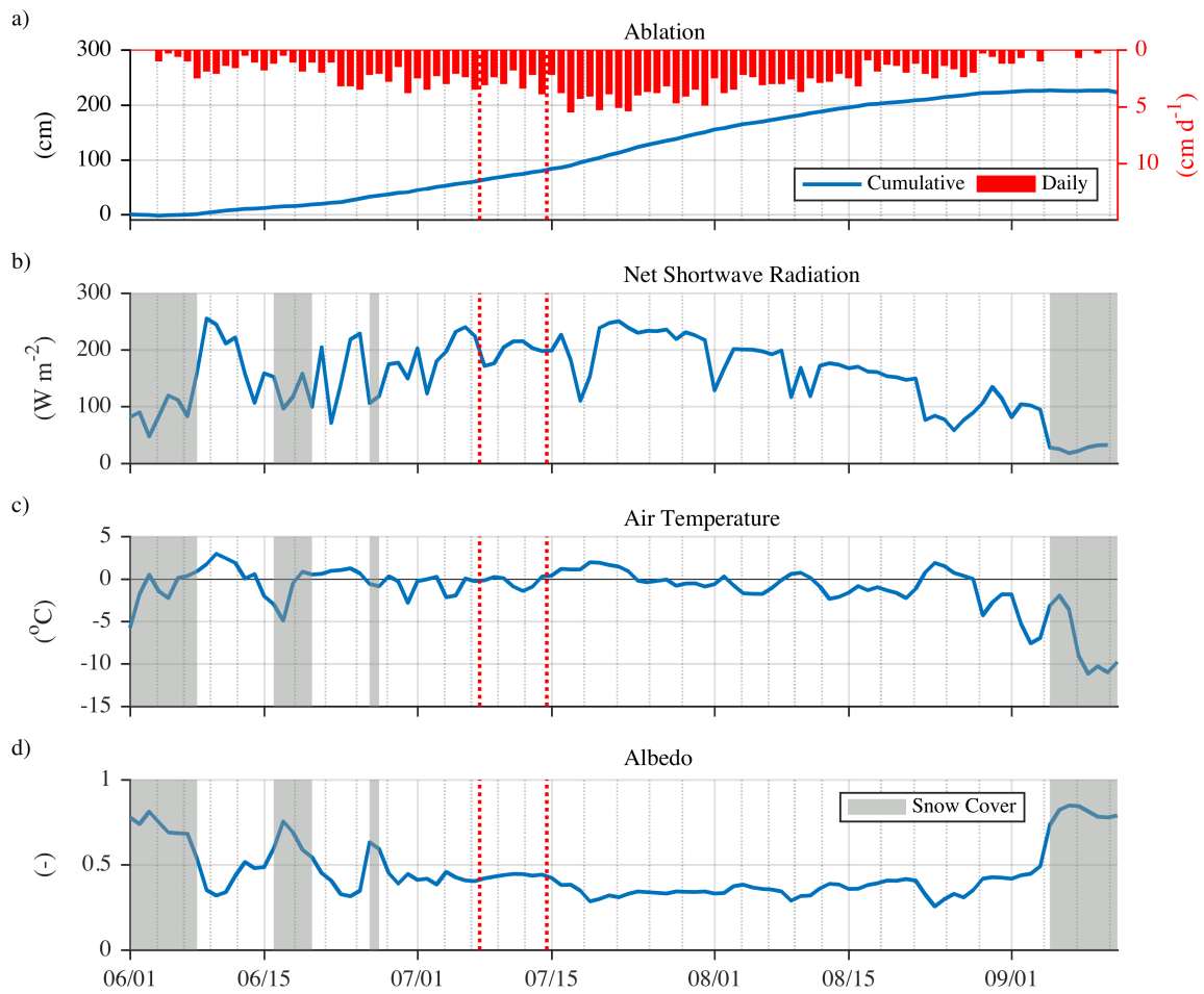
Fig. 8. Meteorological records of a) daily and cumulative ice surface ablation, b) net shortwave radiation, c) 2 m air temperature, and d) albedo, for the period 01 June 2016 – 15 September 2016. Data were collected by the PROMICE/GAP KAN-M automatic weather station (for location see Fig. 2). Vertical grey shaded bars indicate time periods when albedo was greater than >0.5, indicating snow cover was likely present. Albedo is calculated from the ratio of outgoing solar radiation to incoming solar radiation measured ~2 m above the ice sheet surface at the KAN-M station ( www.promice.org ).
