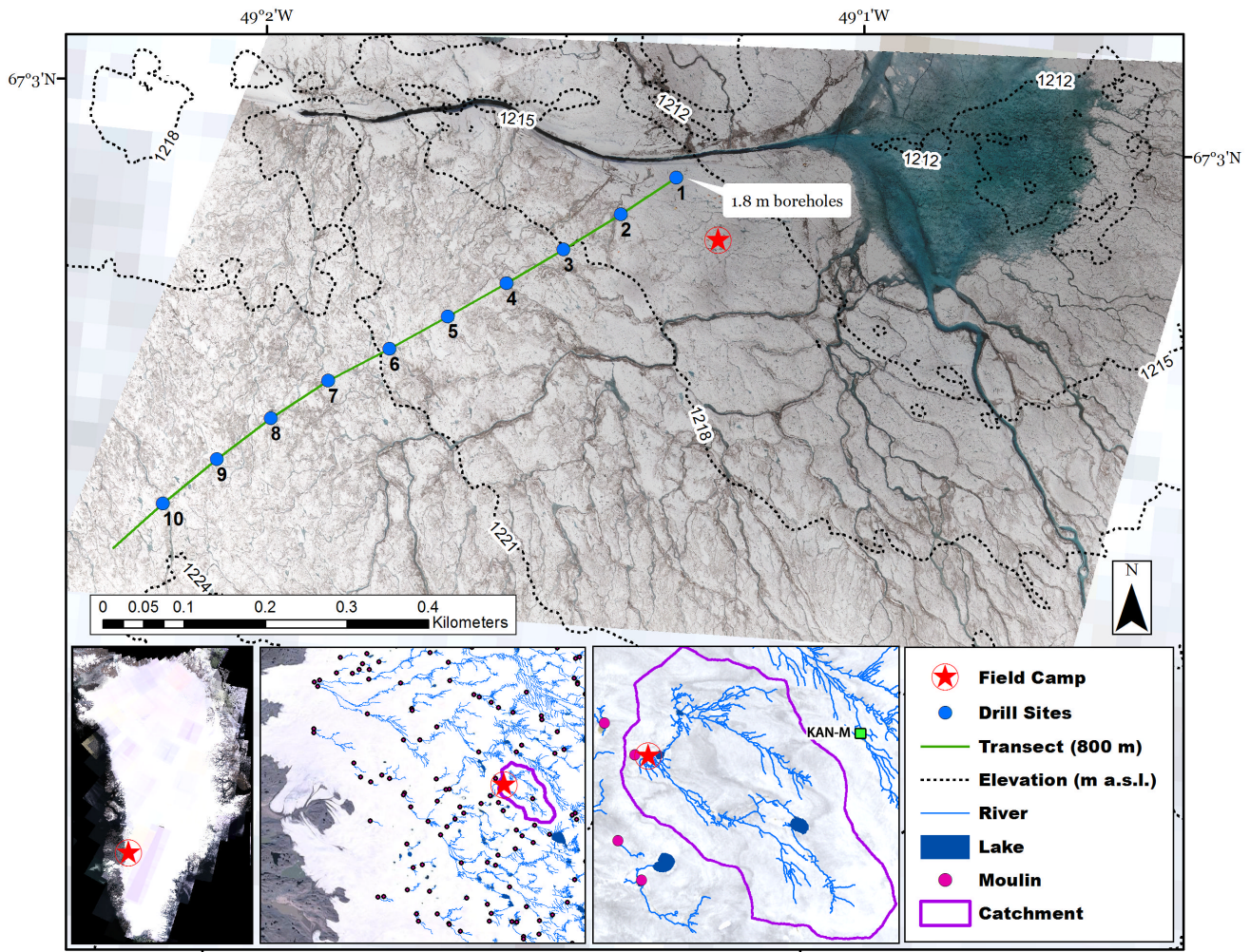
Fig. 2. Ortho-rectified image mosaic of the study area at 6 cm ground resolution from RGB camera imagery collected 10 July 2016 on board a quad-copter drone. Background 30 m Landsat image collected same day. Shallow ice cores extracted at 80 m intervals (blue circles) along the 800 m transect provide ice density measurements to depths of 1.1 m, with two additional shallow ice cores extracted to 1.8 m depth at interval 1. Insets (below) show the 63.1 km 2 supraglacial catchment extent (magenta outline), as delineated from WorldView satellite stereo-photogrammetric digital elevation model topography, and supraglacial river and moulin locations derived from Landsat 8 imagery (Yang and Smith, 2016).
