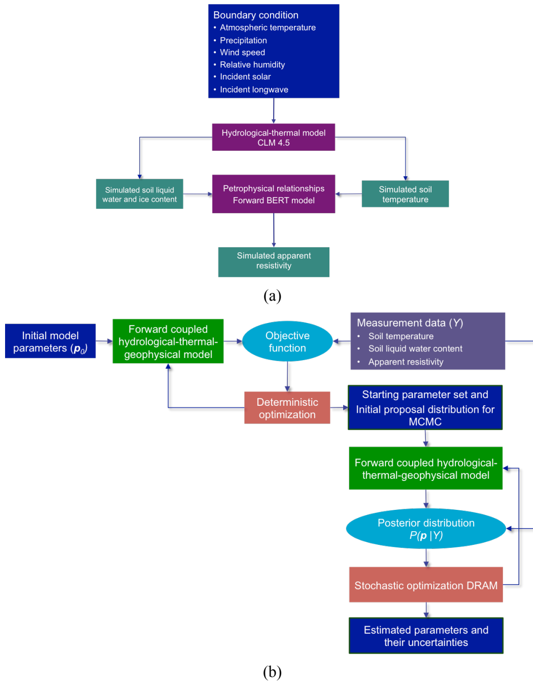
5 Figure 1: (a) Forward coupled hydrological-thermal-geophysical model that considers soil liquid/ice water content, temperature and apparent resistivity. (b) The two-stage inversion scheme combines deterministic and stochastic optimization algorithms to estimate the pdfs of desired model parameters ( p ), which include the OC content (scenarios from 1 to 9), sand content (scenarios 8-9) and petrophysical parameters (scenarios 8-9) (see Table 2). The scheme permits to flexibly use single or multiple types of data for inversion. The forward coupled hydrological-thermal-geophysical model (a) is iteratively executed in both deterministic and stochastic inversion stages.
