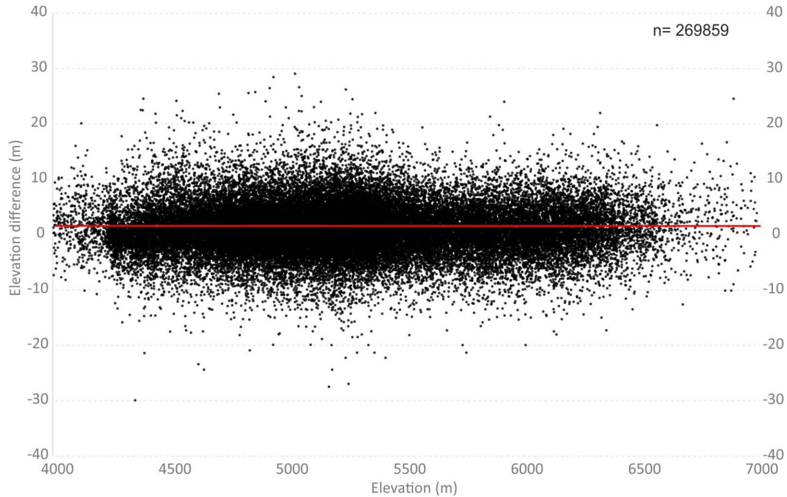
Supplementary figure 1. Stable ground elevation difference versus elevation across the study area. The difference grid was resampled to 100 m pixel size.
