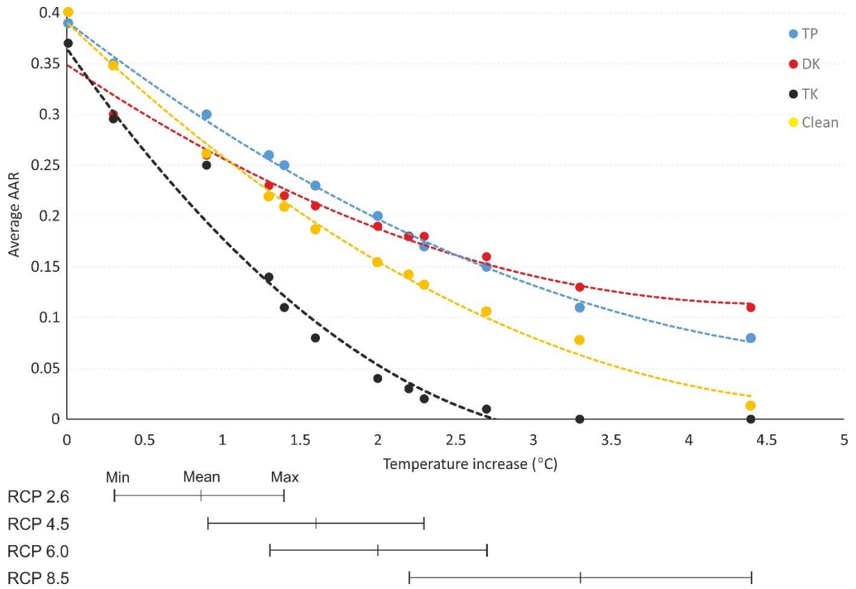
5 Figure 7. Projected AARs (averaged across each catchment) based on different scenarios of temperature increase relative to the present day and accompanying ELA rise. Temperature rise scenarios have been used from the IPCC AR5 Working Group report. TP- Tibetan Plateau; DK- Dudh Koshi; TK- Tama Koshi; Clean- Clean ice glaciers. Each point represents a projected AAR given minimum, mean or maximum temperature rise under each RCP scenario.
