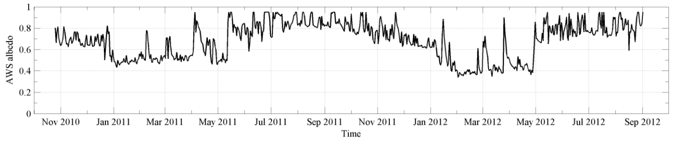
Figure 3. Daily accumulated albedo record (i.e., the ratio of accumulated SW\uparrow and SW\downarrow over a day) of Brewster Glacier, October 25, 2010 to September 1, 2012 (Cullen & Conway, 2015). Note that an upper threshold of 0.95 was applied when SW\downarrow was compromised by snow covering the upper radiation sensors during heavy snowfall (35 occurrences out of 678 days).
