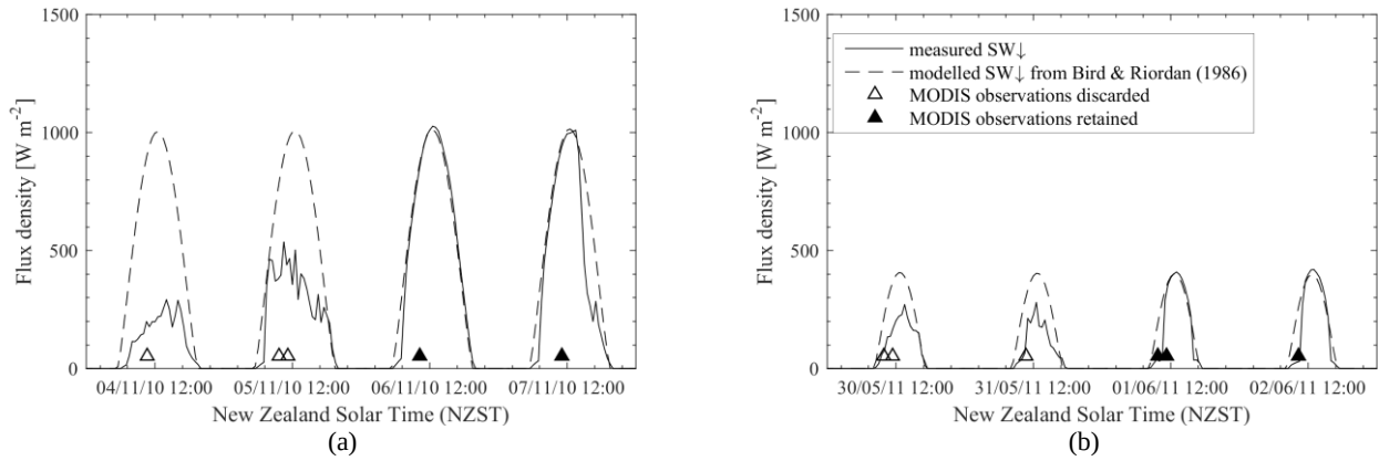
Figure 6. Measured \text{SW}_{\downarrow} compared to that predicted by integrating the SPCTRAL2 clear sky solar spectral model of Bird & Riordan (1986) over the range of wavelengths captured by the pyranometer i.e., (300-2800 nm) over four days in summer (a) and winter (b). Solid triangles correspond to MODIS observations retained in the strict subset of images with guaranteed clear sky conditions.
