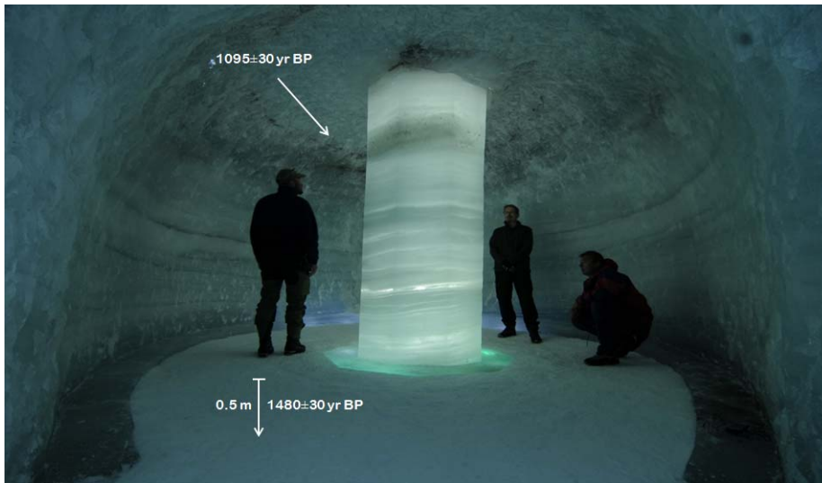
1 2 3 Figure 15. Photo from the old ice tunnel excavated in 2010 showing the layering in the ice 4 and position of two samples for radiocarbon dating. Photo: Klimapark2469 AS. 5
