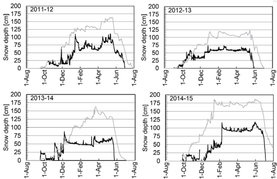
Figure 12. Hourly snow depth measurements (black lines) from the station 95 m from the front of Juvfonne (see Figure 3a for position). Grey lines show modelled daily snow depth from seNorge (Engeset et al. 2004).
