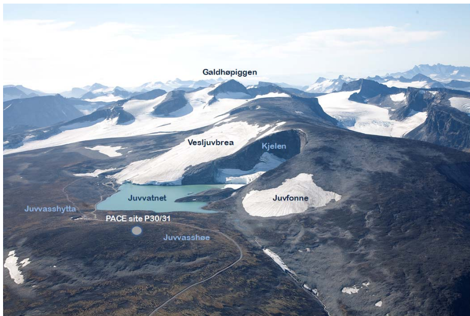
1 2 Figure 2. Overview picture from September 2008 towards SSW showing Juvfonne and the 3 Juvflye area including Kjelen, Juvvatnet, Juvvasshytta, Vesljuvbrea and the P30/31 4 Permafrost and Climate in Europe (PACE) boreholes at Juvvasshøe. Also visible is the 5 highest mountain of Norway, Galdhøpiggen (2469 m a.s.l.). Photo: Helge J. Standal. 6
