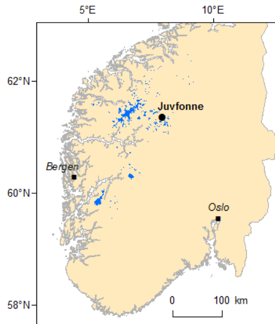
1 2 3 Figure 1. The field site Juvfonne in central southern Norway. Dark blue areas are glaciers. 4
