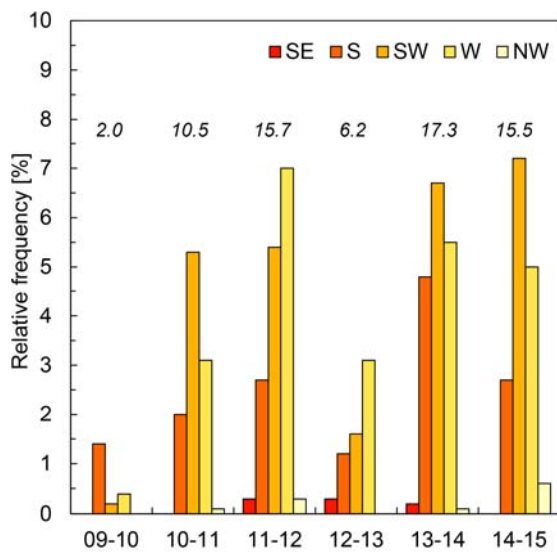
Figure 11. Relative frequency (as percentage of all hourly observations) of strong gale or more ( \geq 20.8 ms ^{-1} ) at Juvvasshøe during winter (Oct-Apr) 2009-2015 for the wind sectors SE to NW. The values inserted show the total frequency of strong gale or more.
