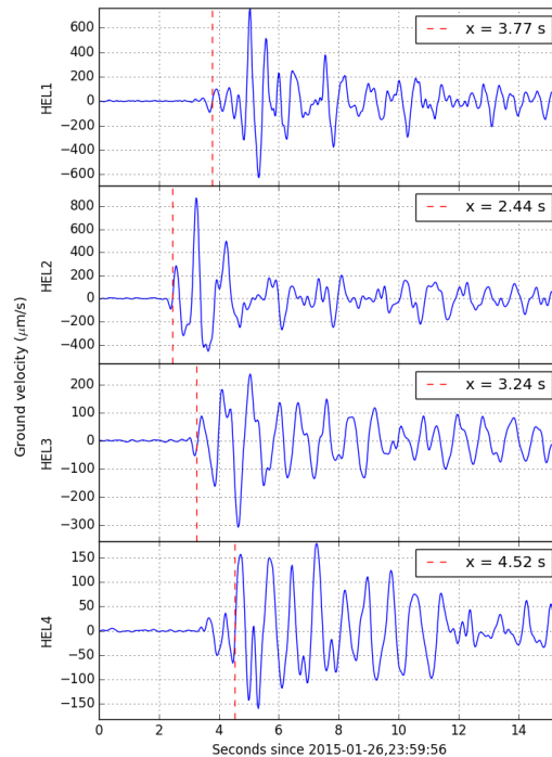
Figure 4. Seismic signals for a calving event at Helheim Glacier on January 26 2015. The signal onset times are determined using an automated script that searches for the first instance of a gradient exceeding a particular threshold as defined in Section 3.2. The differences in the wave onset times are then used to generate a characteristic path difference for each hyperbola.
