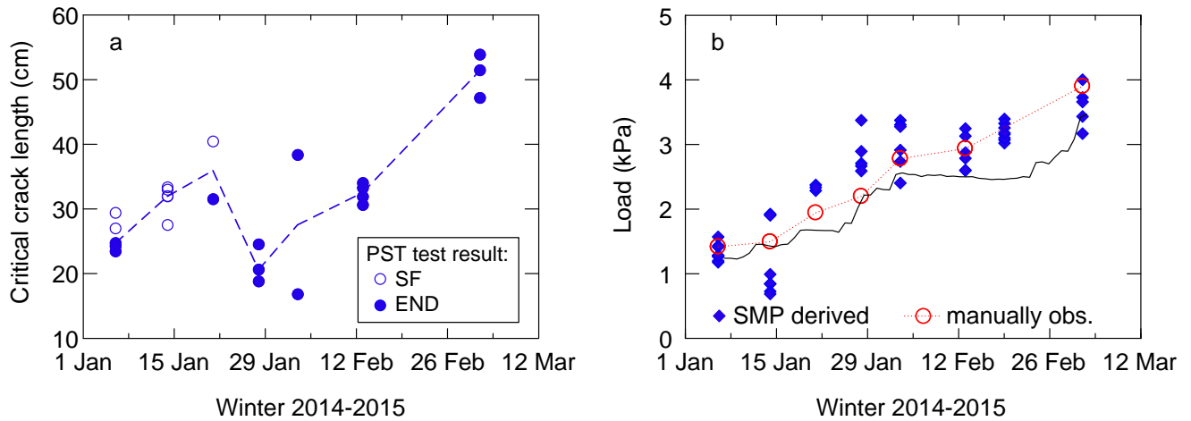
5 Figure 2: (a) Critical cut length as observed in propagation saw tests (Number of cases: N = 23 ). Full circles indicate crack propagation to the very end of the column (END), open circles indicate partial propagation resulting in a fracture across the slab (SF); dashed line connects the median values per day. (b) Load on the weak layer: red open circles (connected by dotted line) show the load as calculated from the manually observed density and layer thickness; blue diamonds are corresponding SMP-derived values ( N = 50 ). The black solid line indicates the load as provided by SNOWPACK.
