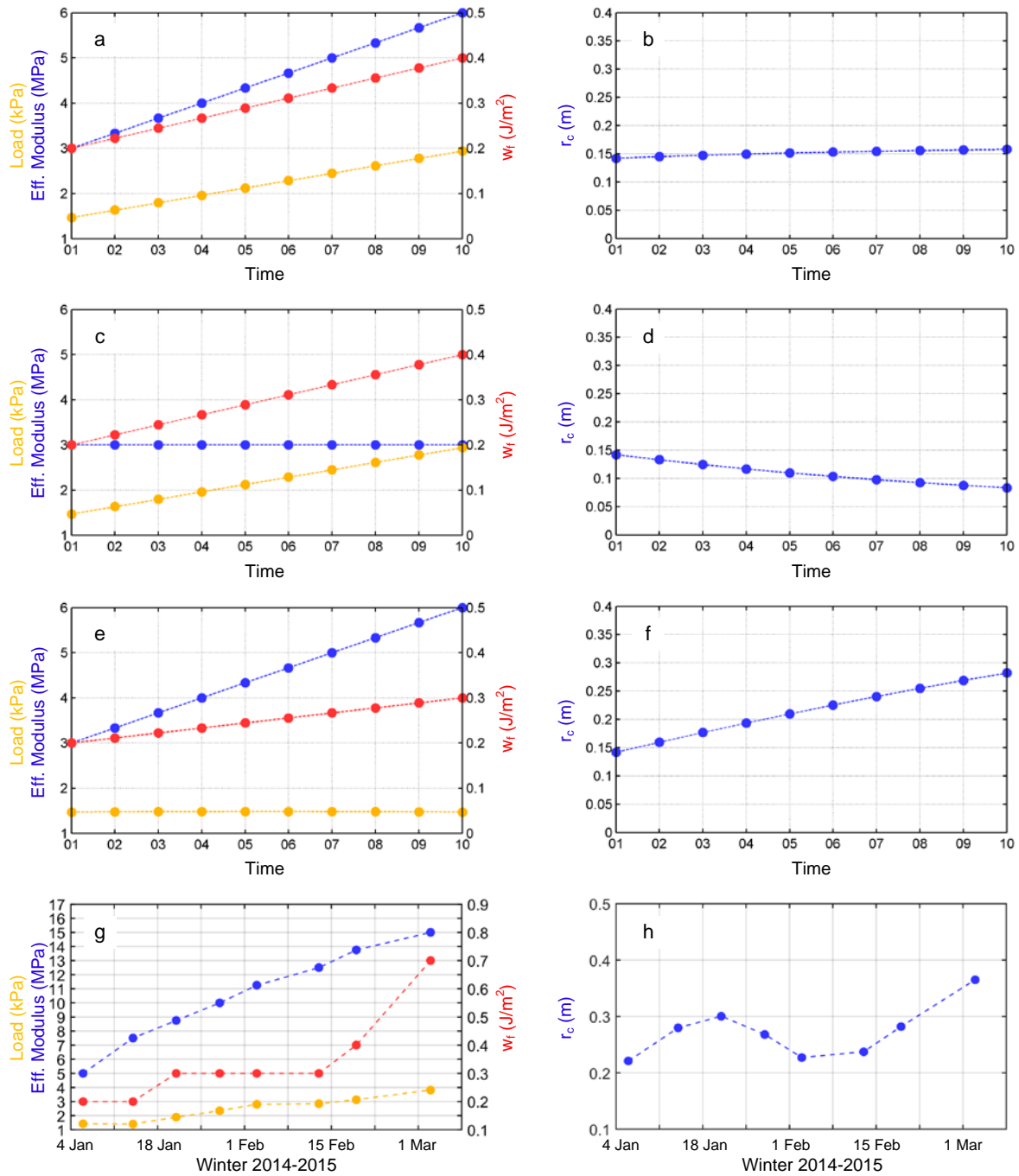
Figure 7: Sensitivity study on how the critical cut length r_c varies as a function of the load and the effective modulus of the slab, and the specific fracture energy of the weak layer w_r . Arbitrary units of time for the three simplified scenarios shown in panels (a) to (f). In the last scenario (g,h), the situation during the sampling period is supposed to be roughly mimicked.
