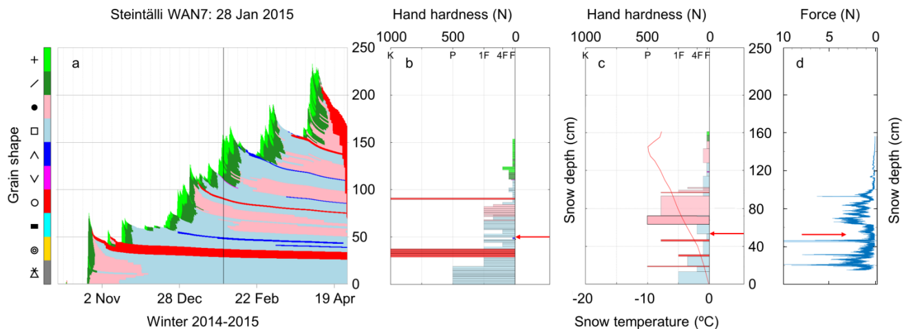
5 Figure 1: (a) SNOWPACK simulation for the location of the automatic weather station (AWS) WAN7 for winter 2014-2015 showing the evolution of grain shape, black vertical line indicates date of snow profile (28 Jan 2015), (b) simulated snow profile for 28 Jan 2015, (c) manually observed snow profile at the location of the AWS on 28 Jan 2015, (d) corresponding SMP penetration force signal measured at the location of the manual profile. Red arrows point to the weak layer.
