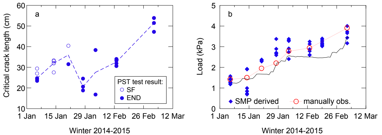
Figure 2: (a) Critical cut length as observed in propagation saw tests (ASTM C1313). Full circles indicate crack propagation to the very end of the column (END), open circles indicate partial propagation resulting in a fracture across the slab (SF); dashed line connects the median values per day. (b) Load on the weak layer: red open circles (connected by dotted line) show the load as calculated from the manually observed density and layer thickness; blue diamonds are corresponding SMP-derived values ( N = 50 ). The black solid line indicates the load as provided by SNOWPACK.
