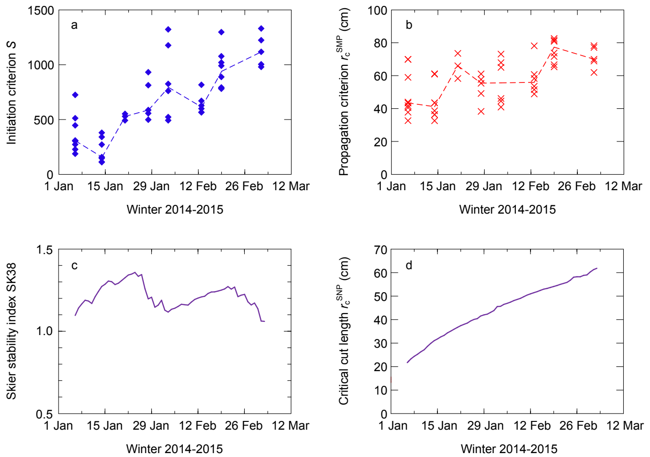
Figure 5: Instability criteria: (a) SMP-derived failure initiation criterion S , and (b) SMP-derived crack propagation criterion r_c^{SMP} ; dashed lines connect median values per day ( N=50 ). Output of the numerical snow cover model SNOWPACK: (c) Skier stability index SK38, and (d) modelled critical cut length r_c^{SNP} .
