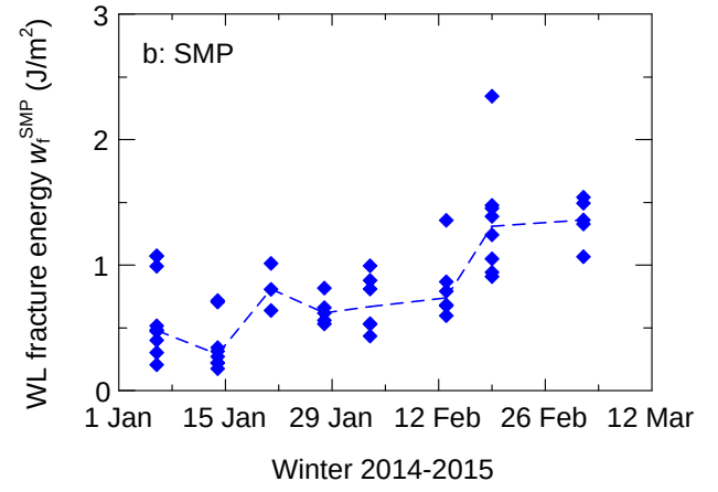
Figure 4: Weak layer specific fracture energy derived from (a) the bending of the slab via PTV analysis ( N = 24 ) with vertical lines denoting measurement uncertainty, and (b) from the SMP signal analysis ( N = 50 ). Dashed lines connect the median values per day.
