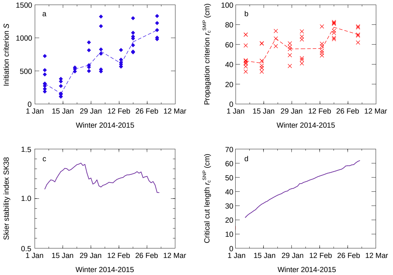
Figure 5: Instability criteria: (a) SMP-derived failure initiation criterion S , and (b) SMP-derived crack propagation criterion r_c^{SMP} ; dashed lines connect median values per day ( N = 50 ). Output of the numerical snow cover model SNOWPACK: (c) Skier stability index SK38, and (d) modelled critical cut length r_c^{SNP} .
