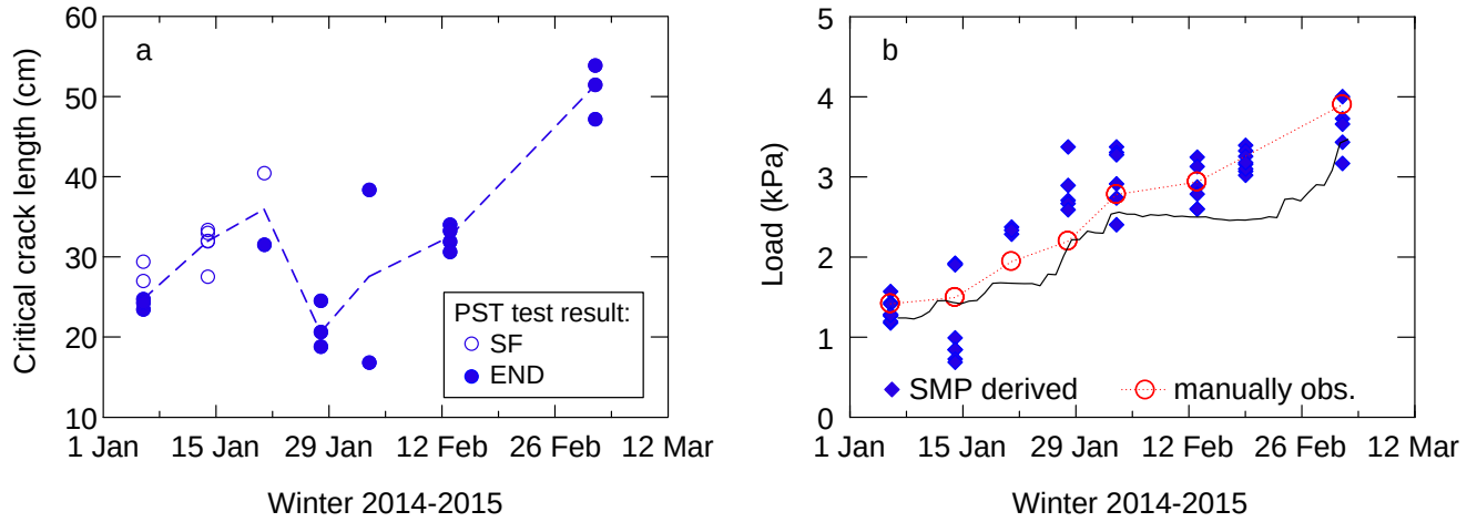
Figure 2: (a) Critical cut length as observed in propagation saw tests (Number of cases: N = 23 ). Full circles indicate crack propagation to the very end of the column (END), open circles indicate partial propagation resulting in a fracture across the slab (SF); dashed line connects the median values per day. (b) Load on the weak layer: red open circles (connected by dotted line) show the load as calculated from the manually observed density and layer thickness; blue diamonds are corresponding SMP-derived values ( N = 50 ). The black solid line indicates the load as provided by SNOWPACK.
