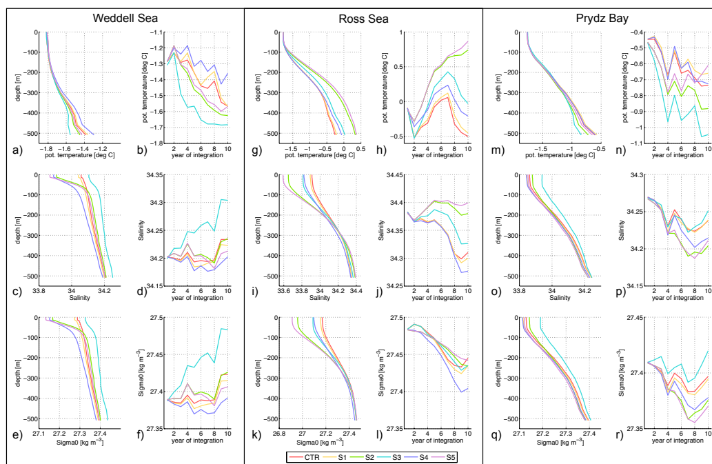
Figure 4. Mean vertical profile \leq 550 m depth (left) and annual mean values at the 550m isobath (right) of potential temperature, salinity and sigma0 in April-September in the a-f) Weddell Sea, g-l) Ross Sea and m-r) Prydz Bay.
