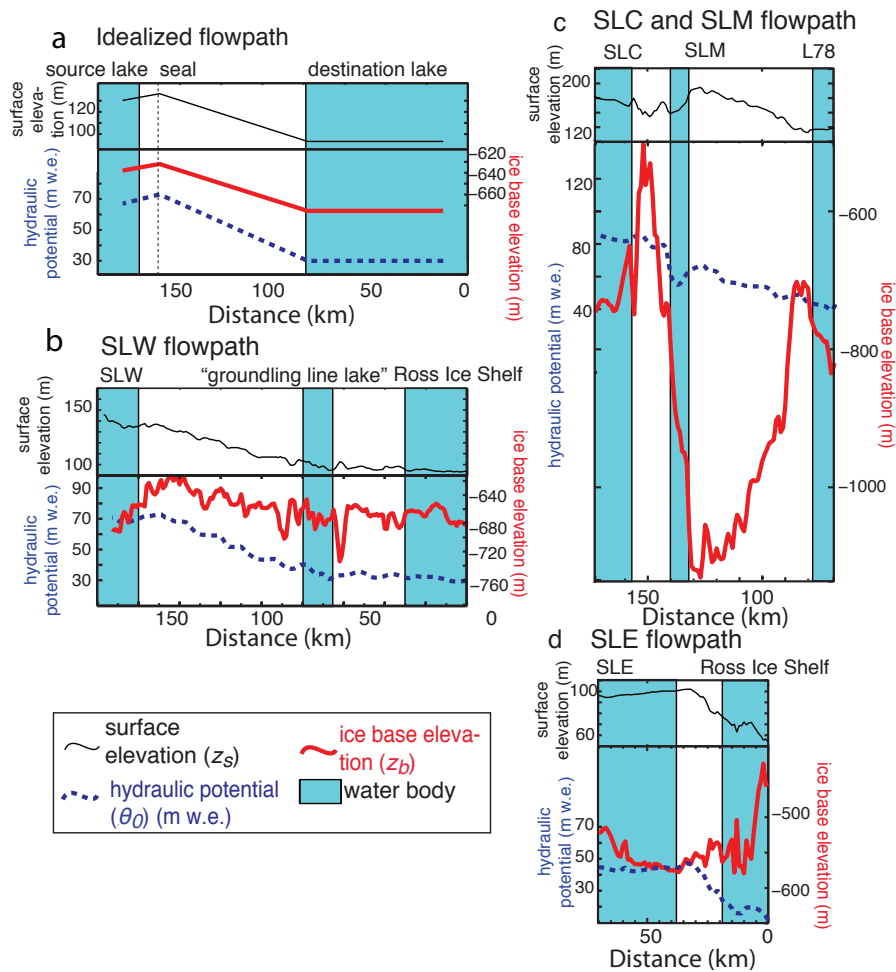
Figure 4. Ice surface elevation, hydropotential, and ice base elevation along the following flow paths (See Figure 1b for location of flow paths): (a) an idealized lake flow path based on SLW, (b) the flow path draining SLW (from Carter and Fricker, 2012), (c) the flow path draining SLC and SLM; and (d) the flow path draining SLE.
