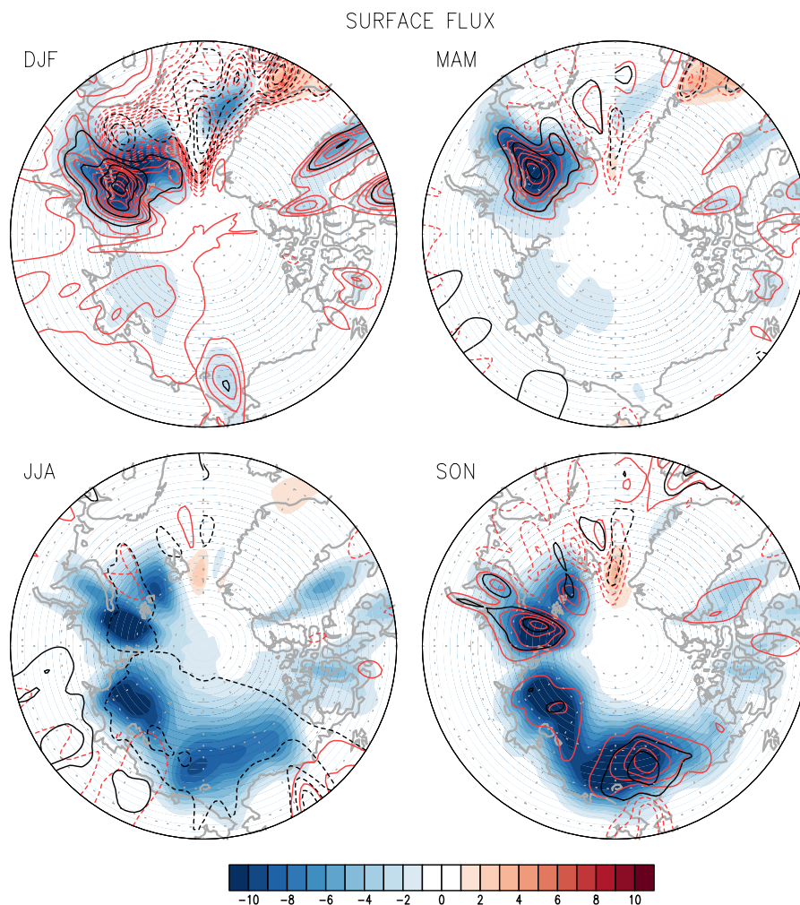
Figure 4. The regressed seasonal patterns of sea ice concentration (shading; 1 %), sensible heat flux (red contours; 1 \text{ W m}^{-2} ), and latent heat flux (black contours; 0.2 \text{ W m}^{-2} ) in the Arctic region ( 64.5^\circ\text{-}90^\circ \text{ N} ). Net upward heat flux is defined as positive.
