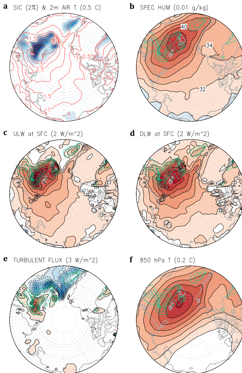
Figure 10. The regressed DJF patterns of (a) sea ice (shading) and 2 m air temperature (contour), (b) 900 hPa specific humidity, (c) upward longwave radiation at surface, (d) downward longwave radiation at surface, (e) turbulent (sensible + latent) heat flux, and (f) 850 hPa air temperature. The green contours in (b)-(f) represent sea ice concentration in (a).
