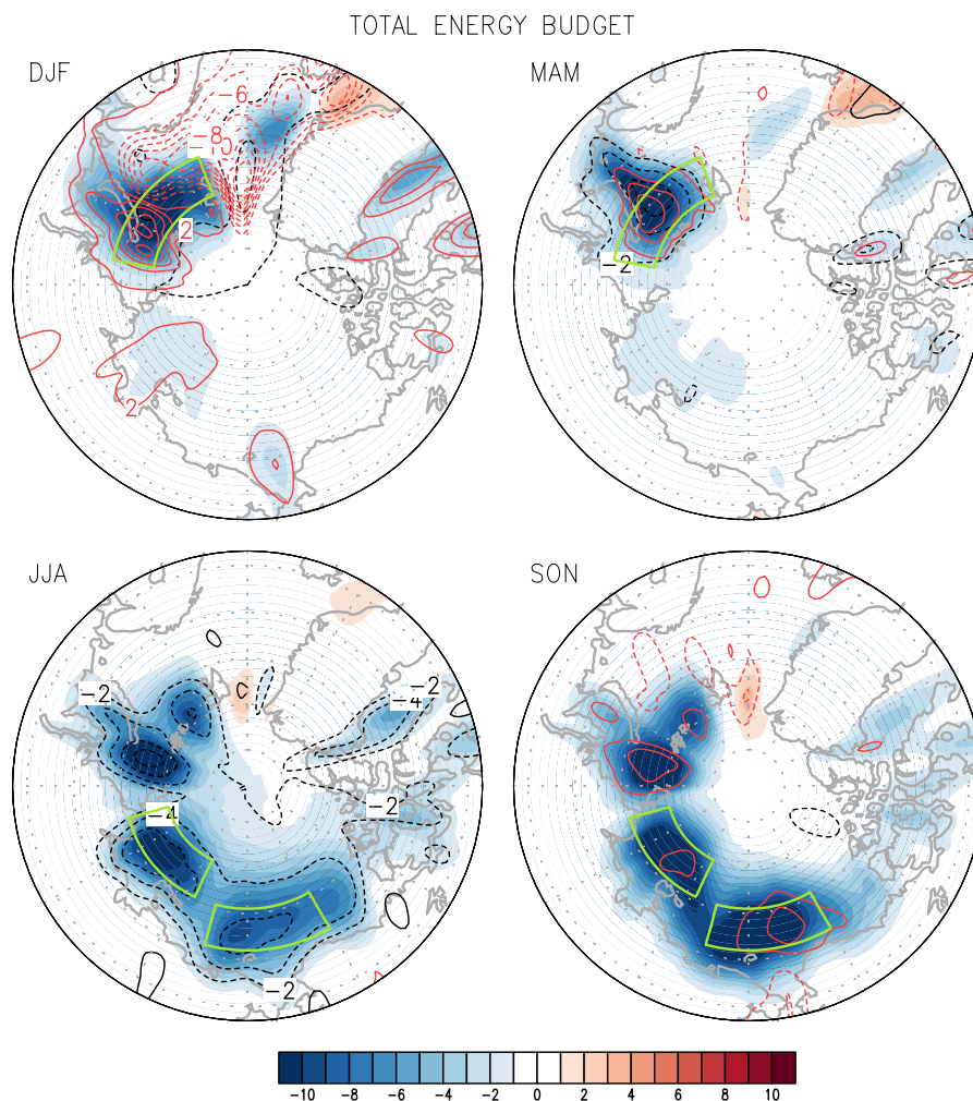
Figure 5. The regressed seasonal patterns of sea ice concentration (shading; 1 %) and net surface radiation (black contours; 2 W m^{-2} ), and turbulent heat flux (red contours; 2 W m^{-2} ) in the Arctic region ( 64.5^{\circ} - 90^{\circ} N). Positive values represent upward radiations and heat fluxes. The three green boxes represent the regions of significant change in sea ice concentration: Barents and Kara Seas [ 21^{\circ} - 79.5^{\circ} E \times 75^{\circ} - 79.5^{\circ} N], Laptev Sea [ 105^{\circ} - 154.5^{\circ} E \times 76.5^{\circ} - 81^{\circ} N], and Chukchi Sea [ 165^{\circ} - 210^{\circ} E \times 72^{\circ} - 76.5^{\circ} N].
