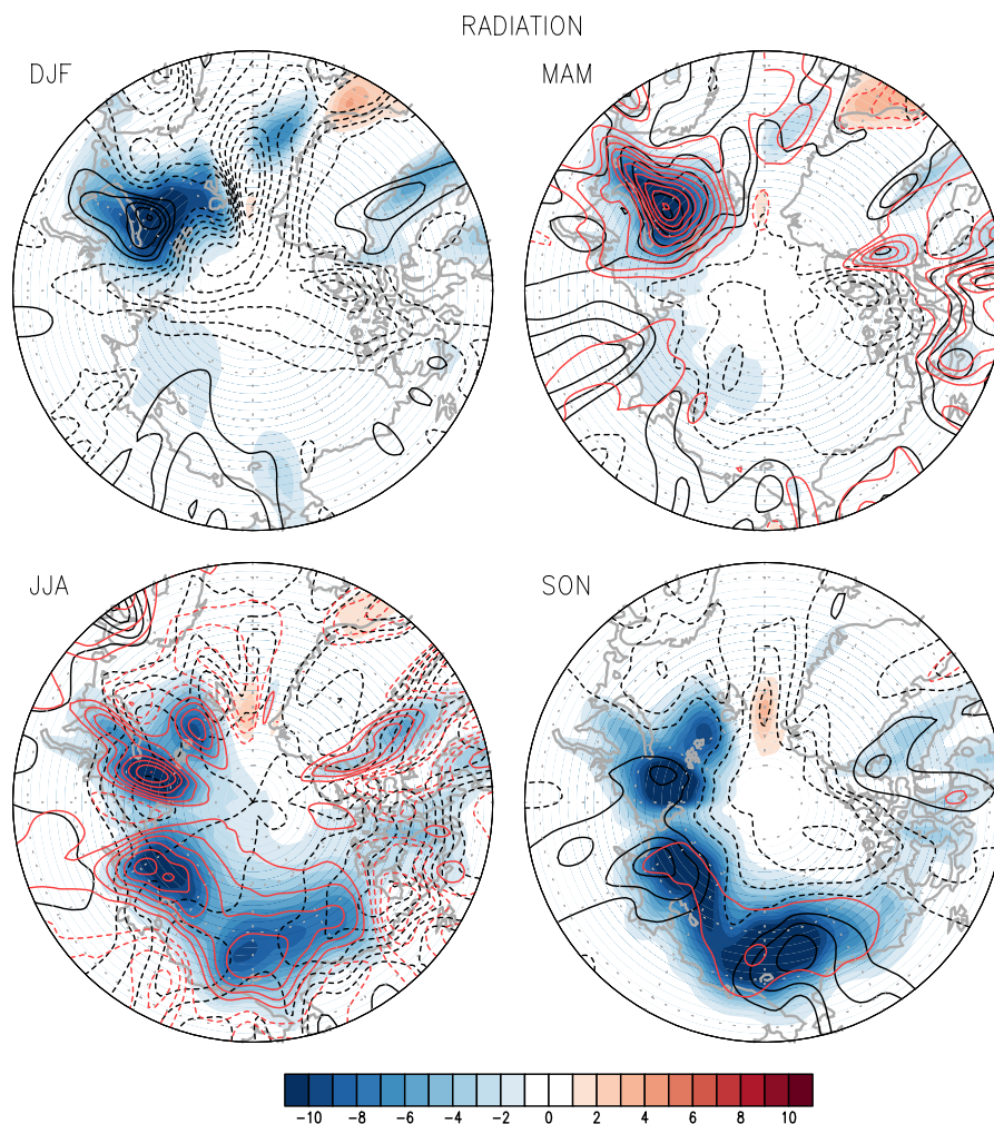
Figure 3. The regressed seasonal patterns of sea ice concentration (shading; 1 %), net shortwave radiation (red contours; 1 \text{W m}^{-2} ), and net longwave radiation (black contours; 0.5 \text{W m}^{-2} ) in the Arctic region (64.5°-90° N). Net upward longwave radiation and net downward shortwave radiation are defined as positive. Solid contours represent positive values and dotted contours represent negative values.
