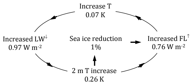
Figure 9. Sea ice melting mechanism in the Barents and Kara Seas. The numbers represent the magnitude of change at each step for a 1 % reduction in sea ice concentration and are based on the January-March averaged loading vector of the warming mode.
