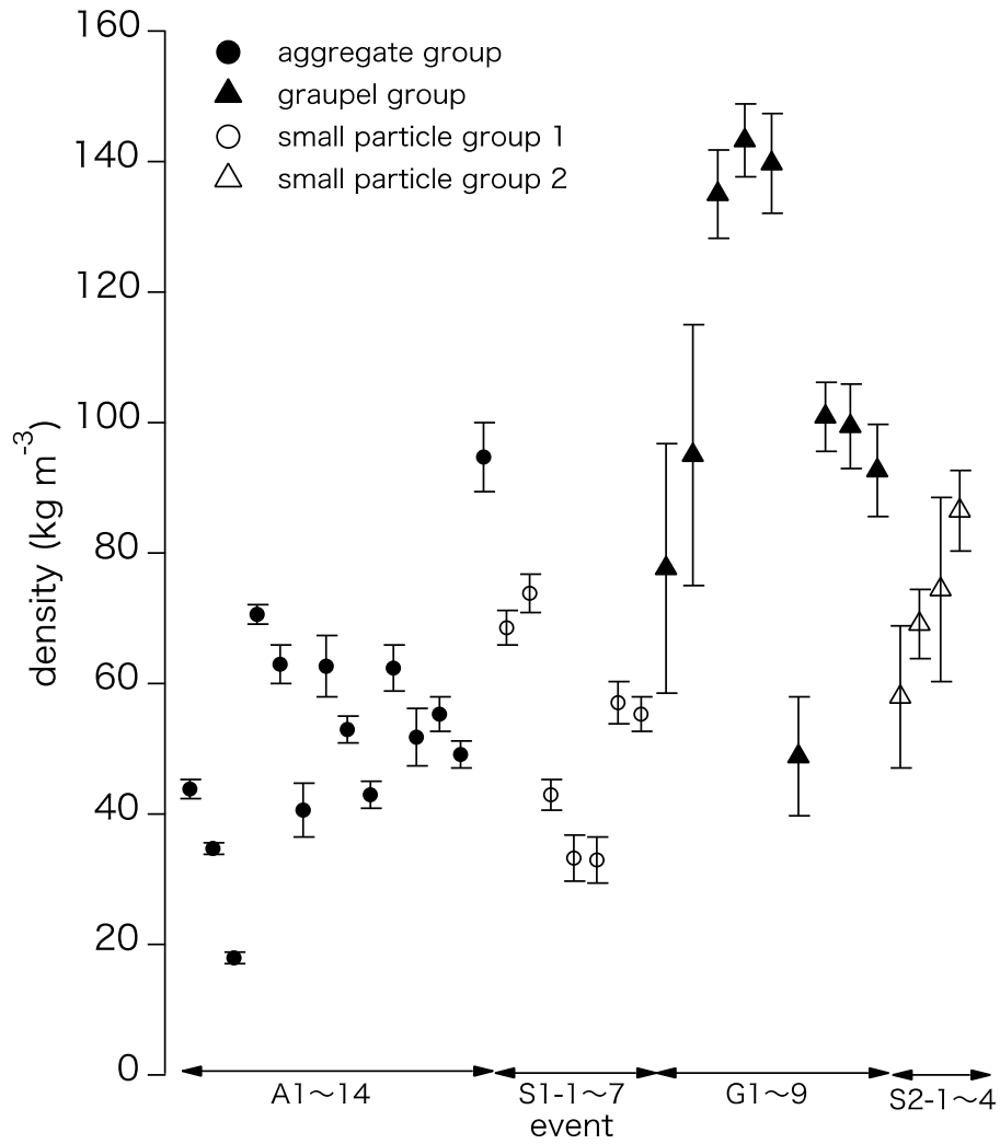
5 Figure 5: Measured snowfall density of events in each classified group: aggregate (A) group (filled circles); graupel (G) group (filled triangles); small particle group 1 (S1) (empty circle); small particle group 2 (S2) (empty triangle). The error bars indicate reading errors.
