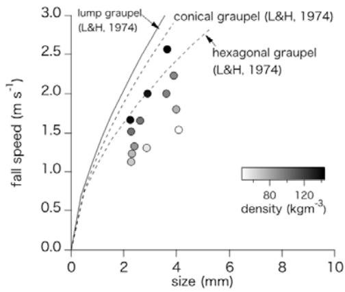
Figure 7: CMF (grey circles) and measured snowfall density of events in the graupel group and small group 2. Density is expressed by grey-scale shading in the circles. The three curves represent size-fall speed relationships for lump, conical and hexagonal types graupel (from Locatelli and Hobbs, 1974, denoted as L&H, 1974 on the graph).
