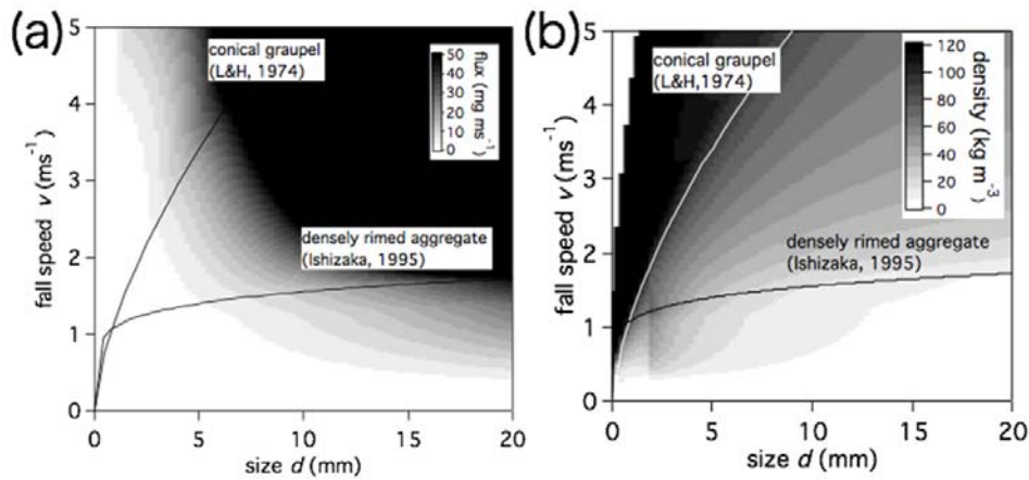
5 Figure 9: (a) Mass flux chart - a graphical expression of the mass flux table which indexes the mass flux calculated in advance for each bin of a given size and fall speed. (b) Density chart - a graphical expression of the density table that indexes density, calculated by dividing the mass deduced from the mass flux table by the volume of sphere of diameter equal to the bin size. The two curves represent relationships for conical graupel (from Locatelli and Hobbs, 1974, denoted as L&H 1974 on the graph), and densely rimed aggregate (from Ishizaka, 1995).
