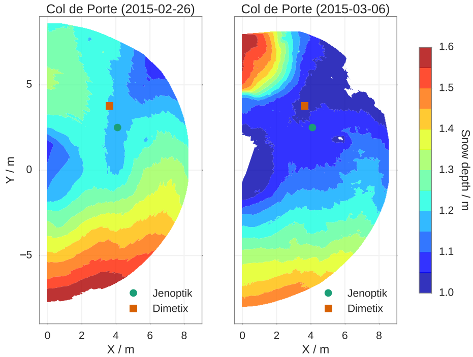
Figure 8. Two snow depth maps acquired at Col de Porte 26 February 2015 when the snow depth reaches its maximum and 6 March 2015 after a windslab wind slab appeared in the North corner (x,y) \approx (0,6\text{ m}) ( x=0, y=6\text{ m} ). The North is approximately in the y-axis direction. The square and round symbols represent the footprint of the SPICE sensors at the beginning of the season.
