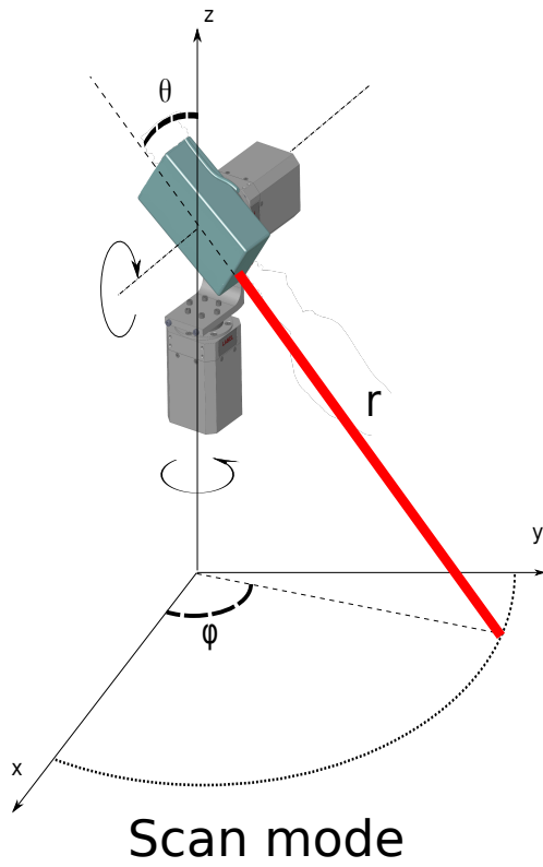
Figure 1. Principle of the scan mode and spot mode of the Rugged Laser Scan (RLS). The zenith angle \theta and azimuth angle \phi determines the orientation of the lasermeter which measures the range r .
