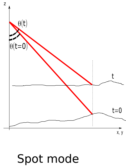
Figure 1. Principle of the scan mode and spot mode of the Rugged Laser Scan (RLS). The zenith angle \theta and azimuth angle \phi determines the orientation of the lasermeter which measures the range r .
