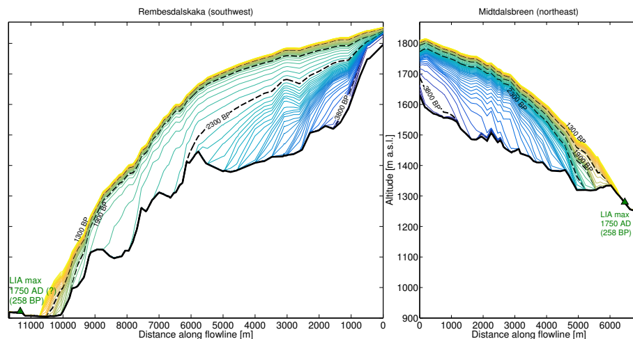
Figure 6. Modelled surfaces from 4000 BP to 1600 AD, starting with no ice cap, shown every 50 years from older (dark blue) to younger (yellow). BP ages are relative to 2008 AD. Note that the top of Rembesdalskåka (Hardangerjøkulen's summit) does not coincide with the top of Midtdalsbreen's flowline (see Fig. 9d).
