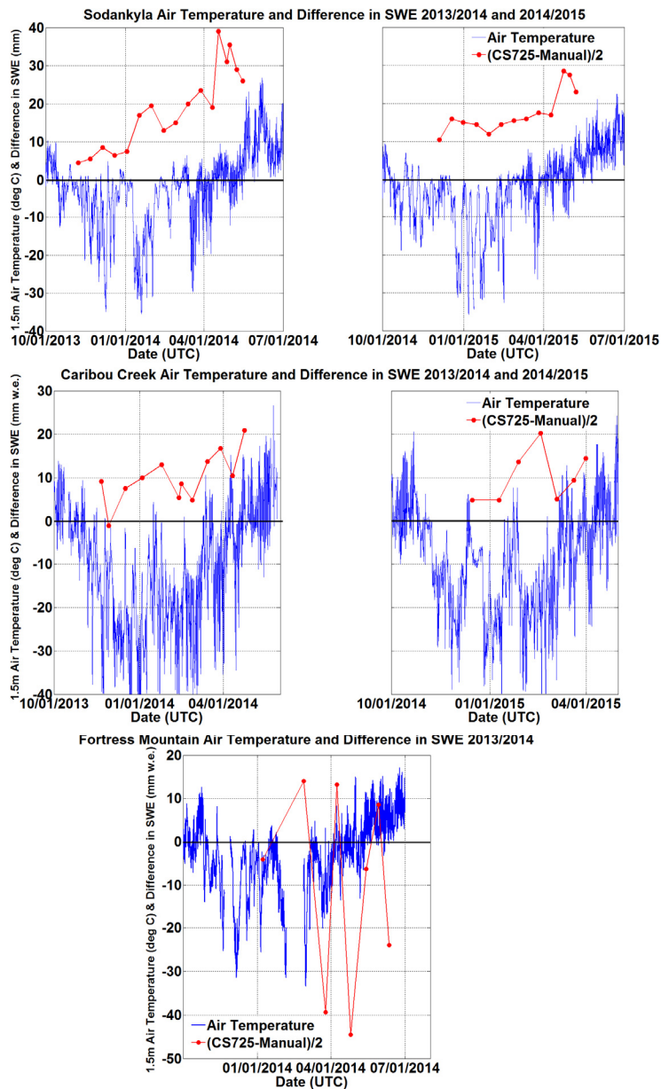
Figure 5: Time series of air temperature (blue) and difference between CS725 and manual measurements (divided by 2, red) at Sodankylä (top) and Caribou Creek (middle) for the 2013/2014 (left) and 2014/2015 (right) seasons, and at Fortress Mountain (bottom) for the 2013/2014 season.
