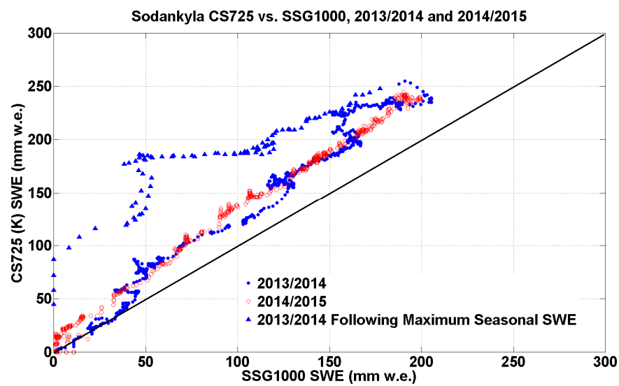
3 | Figure 9: CS725 vs SSG1000 for the 2013/2014 (blue dots/blue triangles magenta ) and 2014/2015 (red) seasons 4 | at Sodankylä. Black line is 1:1.
