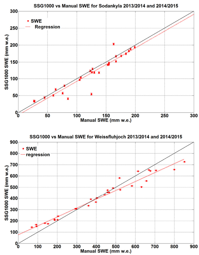
Figure-67: SSG1000 vs Manual SWE at Sodankylä (top) and Weissfluhjoch (bottom) for the 2013/2014 and 2014/2015 seasons. Black line is 1:1. Error bars represent manufacturer’s stated sensor accuracy.
