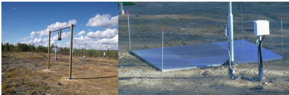
5 6 Figure 2: The Campbell Scientific CS725 (left) installed at Caribou Creek and the Sommer Messtechnik SSG1000 7 (right) installed at Sodankylä.
