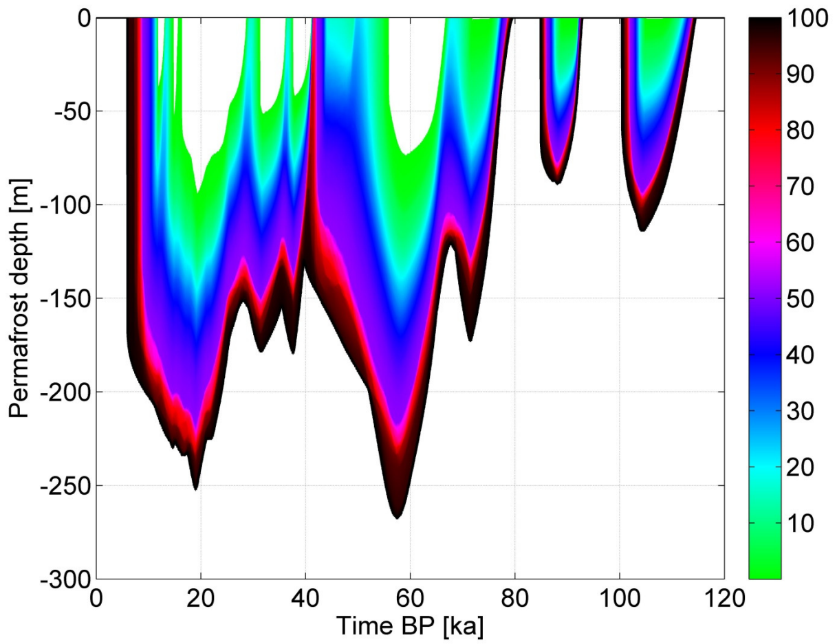
Figure 8: All percentiles of permafrost front penetration depth during a stochastic nation-wide simulation of the Weichselian 5 glaciation.
