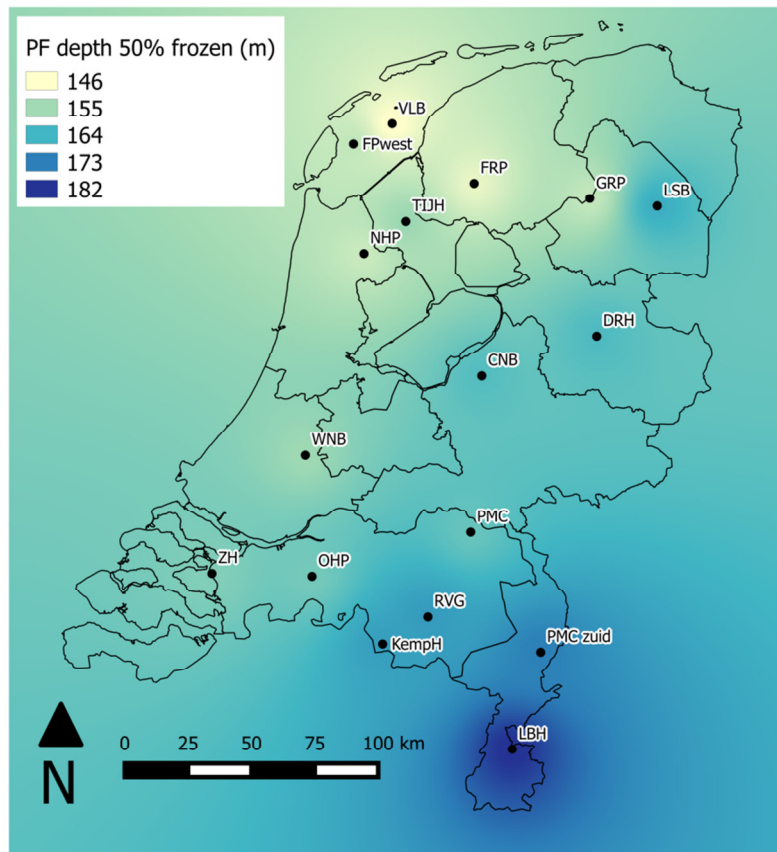
Figure 6 – Interpolated best estimate maximum permafrost depth map for the -0.25^{\circ}\text{C} isotherm. Fifty percent of the pore water along this contour map is in the liquid phase.
