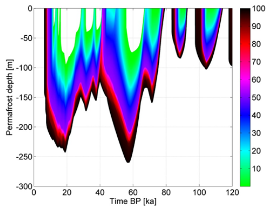
Fig. 1. Results of the uncertainty analysis. Top: previous version (freezing interval 0.5^{\circ}\text{C} to -0.5^{\circ} ), bottom: after first revision (freezing interval 0^{\circ}\text{C} to -0.5^{\circ} ). Differences on the extreme percentiles are
