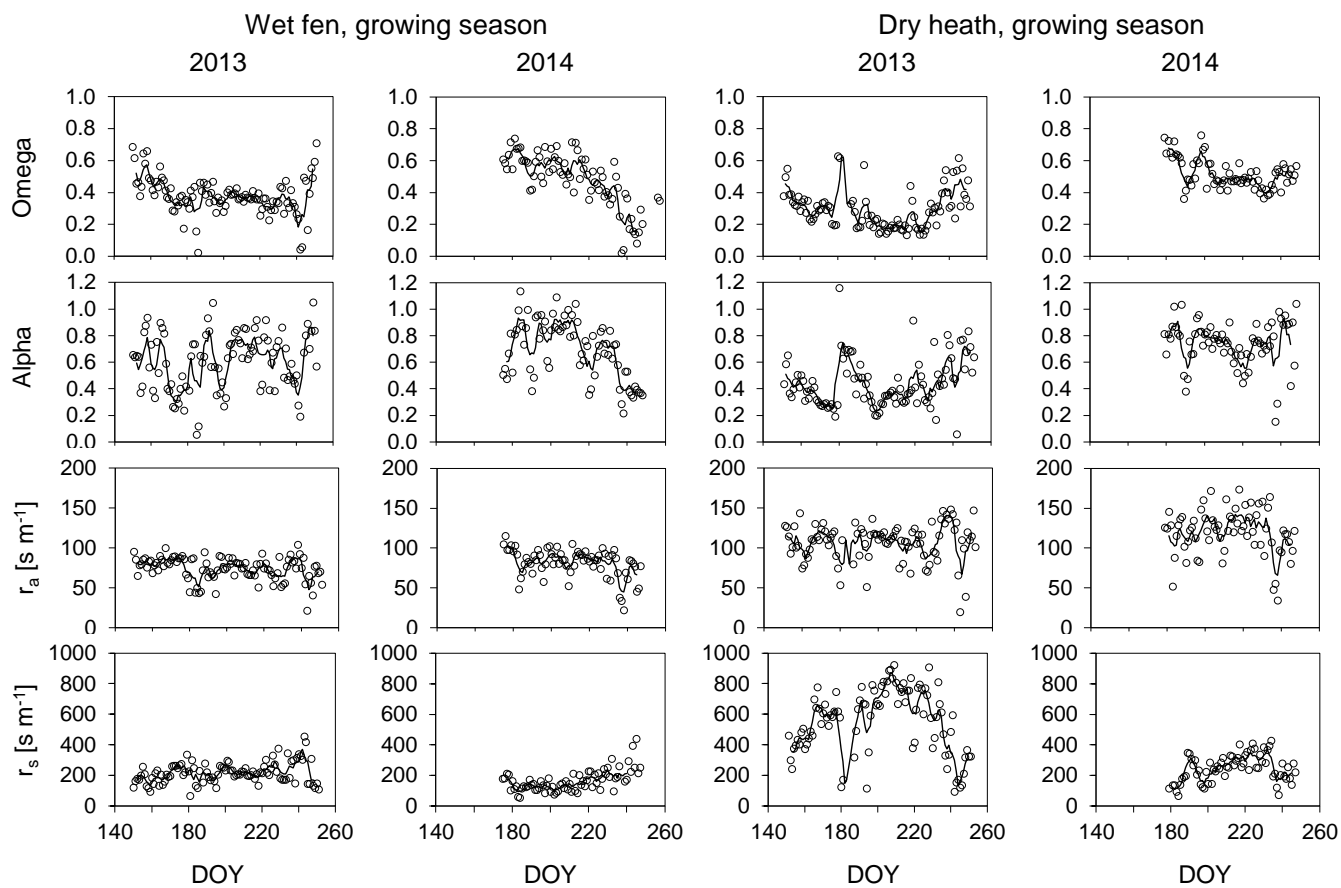
Figure 9: Omega, alpha, aerodynamic resistance and surface resistance.
