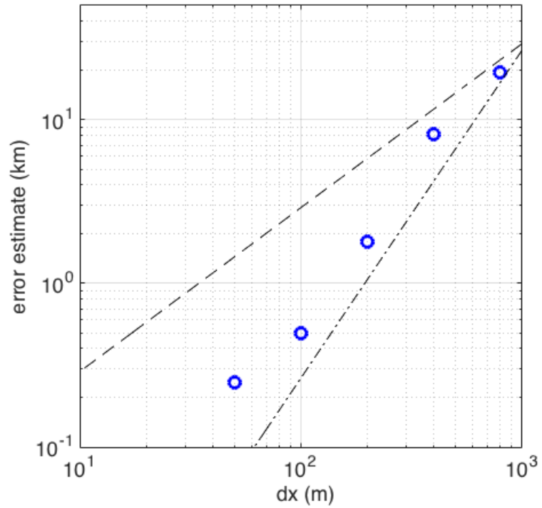
Figure 5. Convergence of the Stnd experiment as a function of along-flow grid resolution (circles), as discussed in Section 5.2. Error estimate for grounding line position are based on Richardson error estimation. Black-dashed and dash-dot lines show perfect linear and quadratic convergence rates (respectively).
