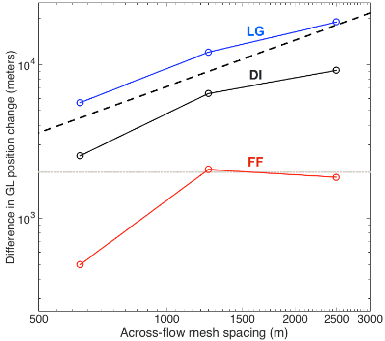
Figure 9. Difference in FELIX-S and Elmer/Ice GL position changes ( \Delta GL_{Elmer} - \Delta GL_{FELIX} ) at the centerline for the P75S experiment as a function of increasing across-flow ( y ) resolution (resolution increases from 2500-625 m as N_y increases from 20-80). Lines representing the differences relative to the LG, DI, and FF implementations in Elmer/Ice are labeled. Black-dashed line shows the slope for a theoretical first-order convergence rate. Grey-dashed line shows the estimated Elmer/Ice truncation error of \sim 2 km, from Durand et al. (2009a) and Gagliardini et al. (2016).
