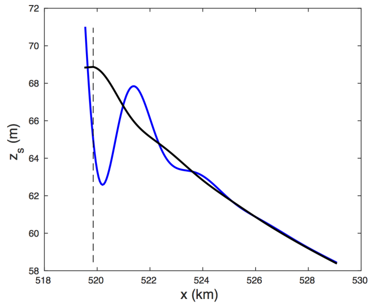
Figure 4. Grounding line position versus local floatation. The vertical black-dashed line marks the equilibrium GL position for the Stnd experiment and the heavy blue and black lines denote the modeled ice sheet surface near the GL (blue) versus that determined by the floatation condition (black) (Compare with the inset in Figure 2b from Durand et al. (2009a)).
