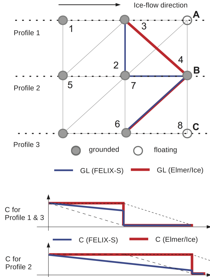
Figure 1. A schematic of the different basal boundary masking schemes used by FELIX-S and Elmer/Ice and their impact on the definition of the MISMIP3d basal friction coefficient ( C(x, y) is assumed uniform beneath grounded ice for illustrative purposes. For floating ice, C(x, y) = 0 ). Circles denote the nodes at the ice-bed interface, defining the basal finite element faces (triangular and quadrilateral for FELIX-S and Elmer/Ice, respectively); open circles denote floating nodes for which z(x, y, t) > b(x, y) and solid circles denote grounded nodes for which z(x, y, t) = b(x, y) and -\sigma_{nn} > P_w . Numbers 1-8 identify triangular element faces of FELIX-S and letters A-C identify specific nodes common to both models. As discussed in Section 6, the different masking schemes lead to the different grounding line positions and also to the different nodal values of C along profiles 1-3. The C profiles based on DI for Elmer/Ice (heavy red line) and FELIX-S profiles (heavy blue line) are shown, as are the corresponding Elmer/Ice FF (black dashed) and LG (black dotted) profiles.
