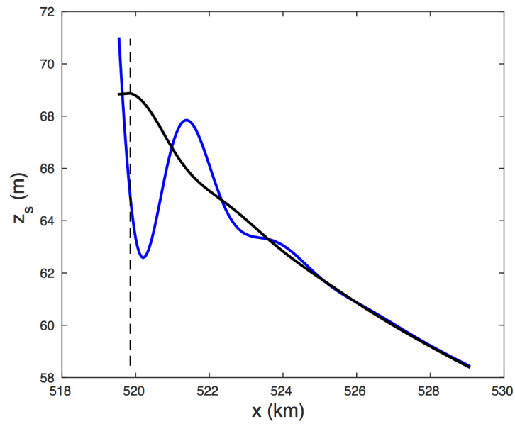
Figure 4. Grounding line position versus local flotation. The vertical black-dashed line marks the equilibrium GL position for the Stnd experiment and the heavy blue and black lines denote the modeled ice sheet surface near the GL (blue) versus that determined by the flotation condition (black) (Compare with the inset in Figure 2b from Durand et al. (2009a)).
