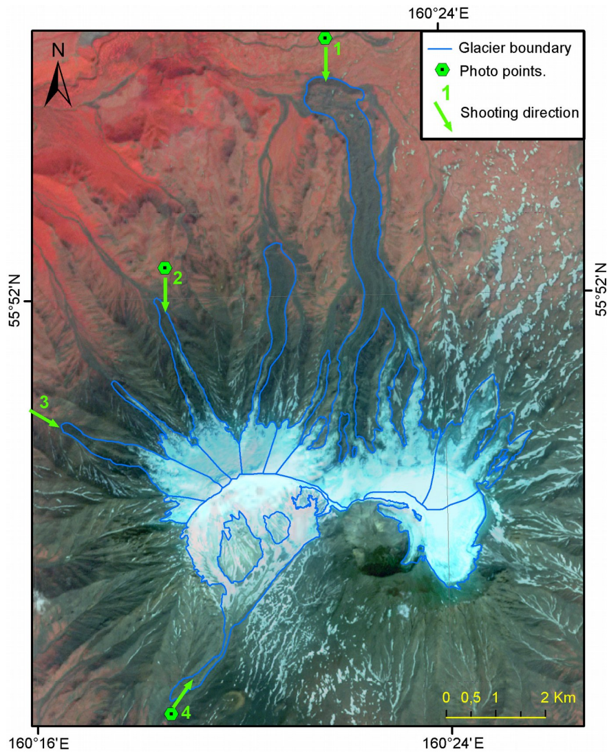
Scheme 1. Tolbachik volcano glaciation. In the substrate ASTER (19.07.2012) satellite image.
