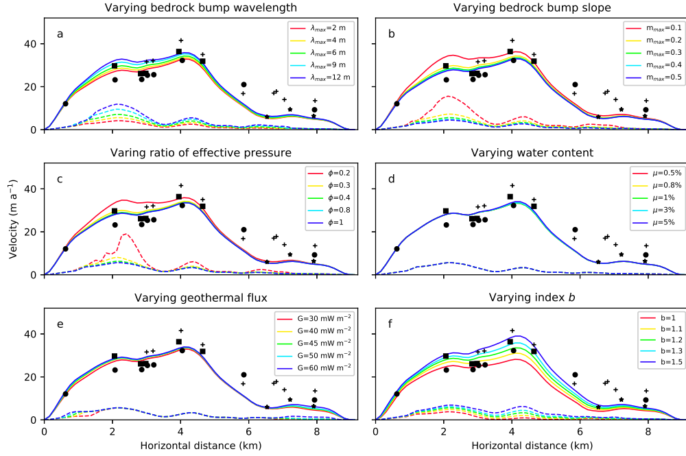
Figure 5. Sensitivity of modeled ice flow speeds to parameters along the CL. The solid and dashed lines indicate the modeled surface and basal sliding velocities, respectively. Markers indicate the measured ice surface velocities same as those shown in Fig. 3.
