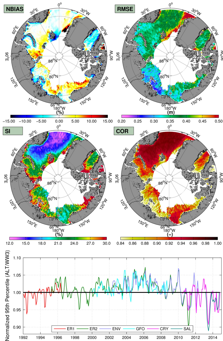
Figure 3. Top four panels display the normalized bias (NBIAS), root mean squared error (RMSE), scatter index (SI), and correlation coefficient (COR) for collocated H_s for the CFSR wave hindcast and the merged altimeters 1992-2014. The bottom panel displays the normalized monthly H_s 95th percentile for each satellite platform: European Remote Sensing Satellites 1 and 2 (ER1, ER2), Environmental Satellite ENVISAT (ENV), Geosat Follow-On (GFO), CRYOSAT2 (CRY), and Altika SARAL (SAL).
