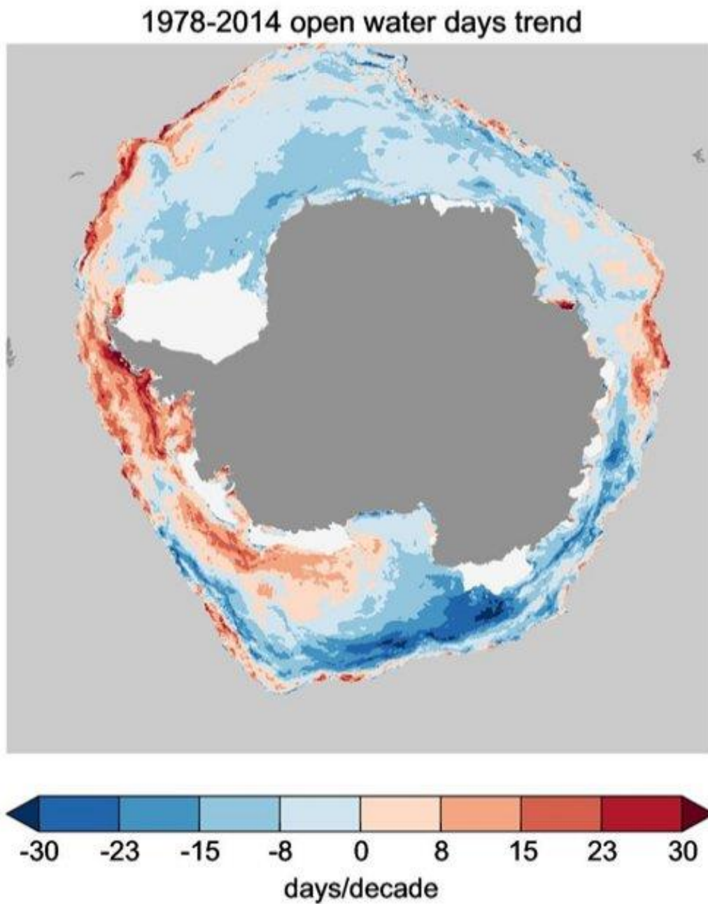
1 2 Figure 14. Show the linear trend in open water days in the Antarctic (1978-2014). 3
