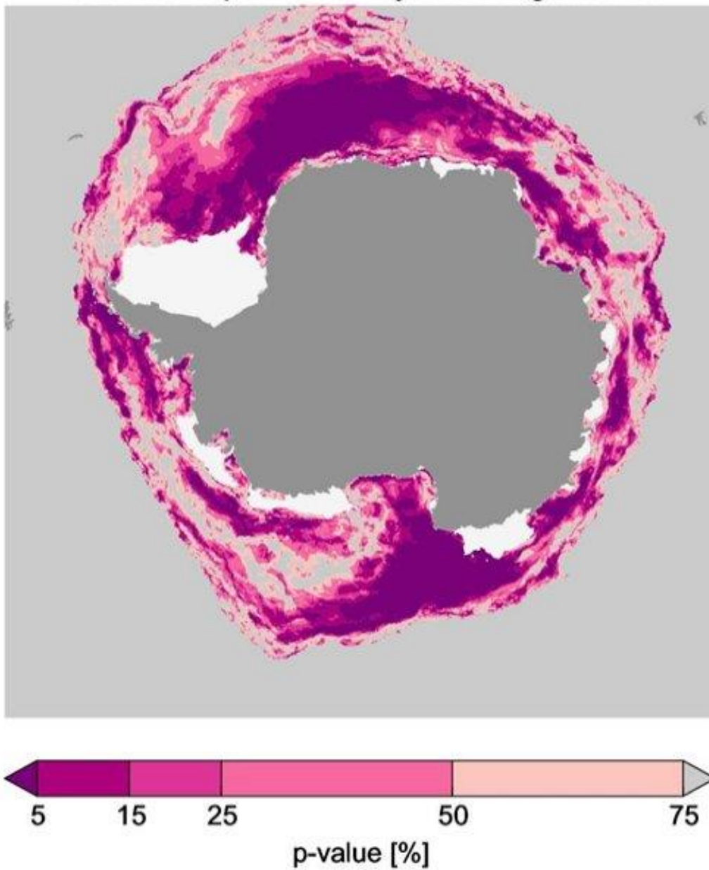
1 2 Figure 15. The probability that the trend in Figure 14 is not significant (test of the null-hypothesis). A 3 low value (< 5 %) indicates that the trend is in fact significant.
