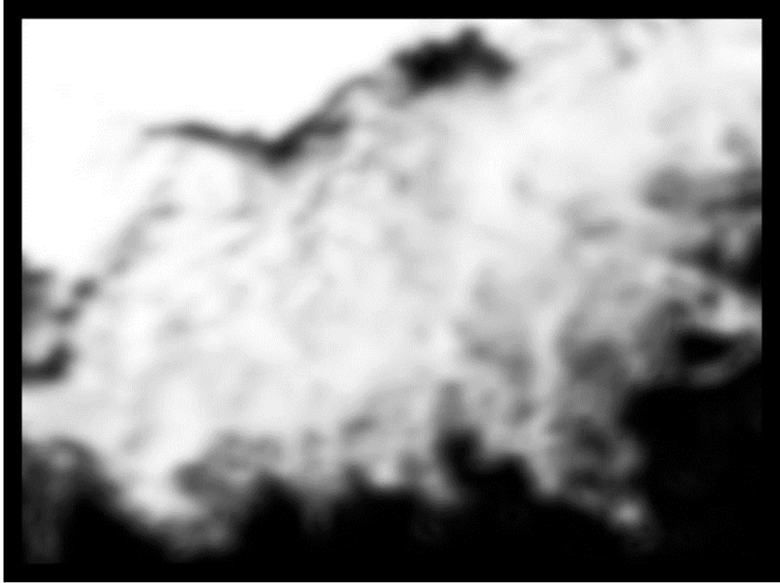
Figure 2. The simulated ice concentrations using the SSM/I sensor specifications and the OSISAF hybrid ice concentration algorithm and the data in Figure 1 as input. Ice concentrations between 0 % (black) and 100 % (white).
