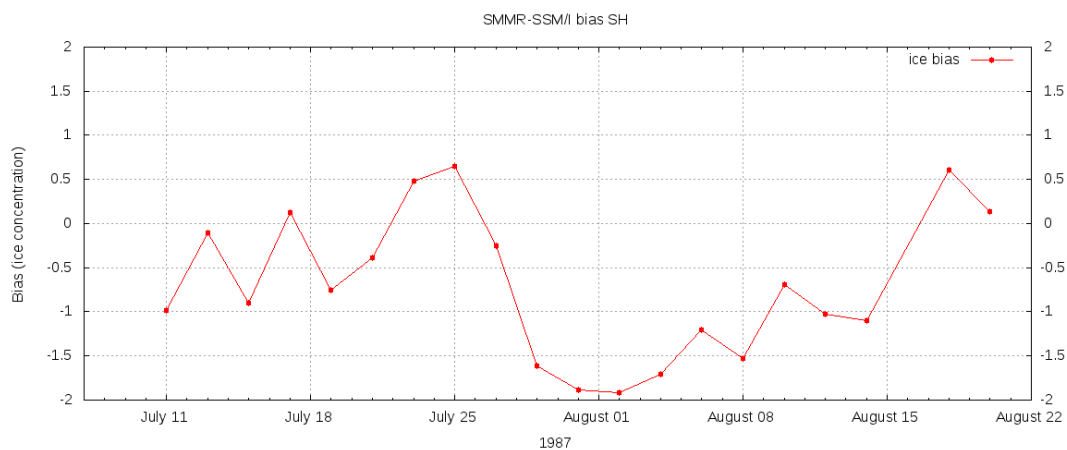
Figure 9. The overlapping SMMR - SSM/I difference around Antarctica during austral winter. The red curve is showing the ice bias.
