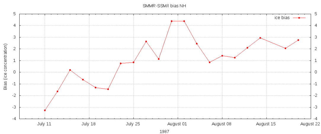
Figure 8. The overlapping SMMR - SSM/I difference in the Arctic during summer melt. The red curve is showing the ice bias.
