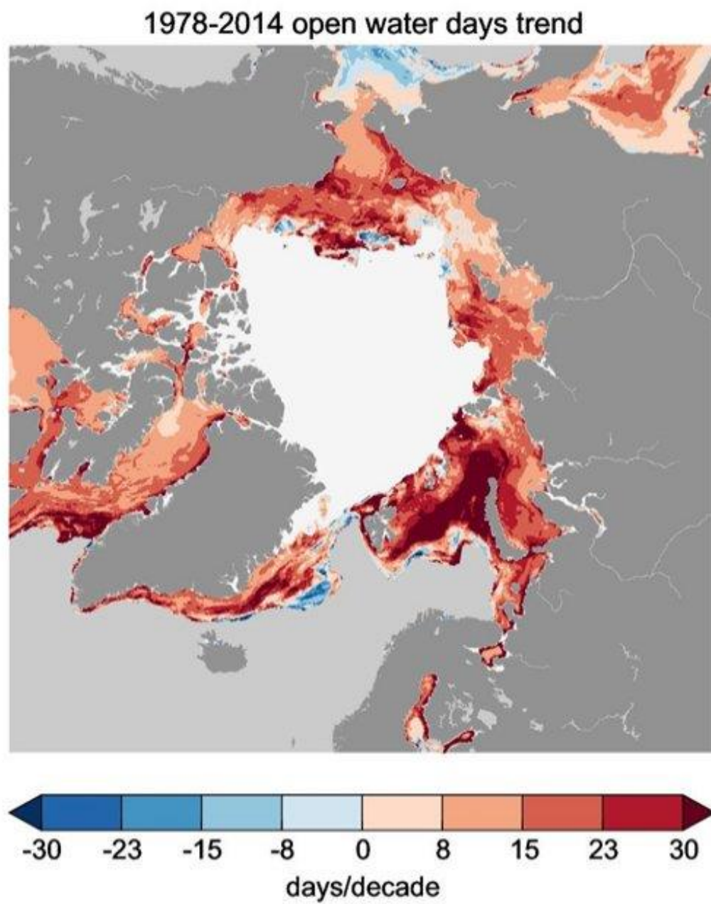
1 2 Figure 12. Show the linear trend in open water days in the Arctic (1978-2014). 3
