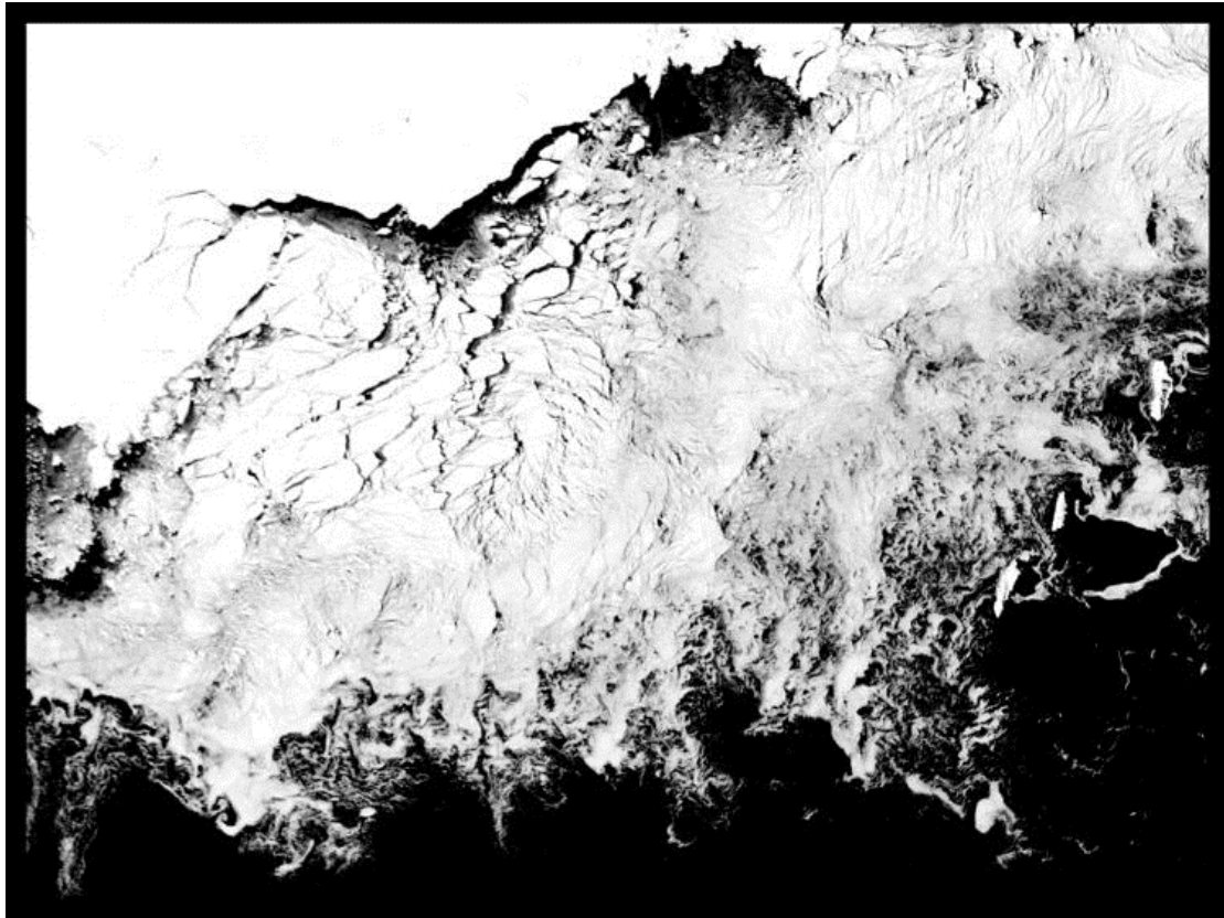
4 5 Figure 1. The 1 km cloud free MODIS image 3000 x 2200 km. The scene is situated north of McMurdo 6 Station and east of the Ross Sea, Antarctica. Ice concentrations between 0 % (black) and 100 % 7 (white). The scene is recorded at 03.30 UTC 2008/02/24 by the Aqua satellite. The scene centre is at 8 69.5°S, 165°W. 9
