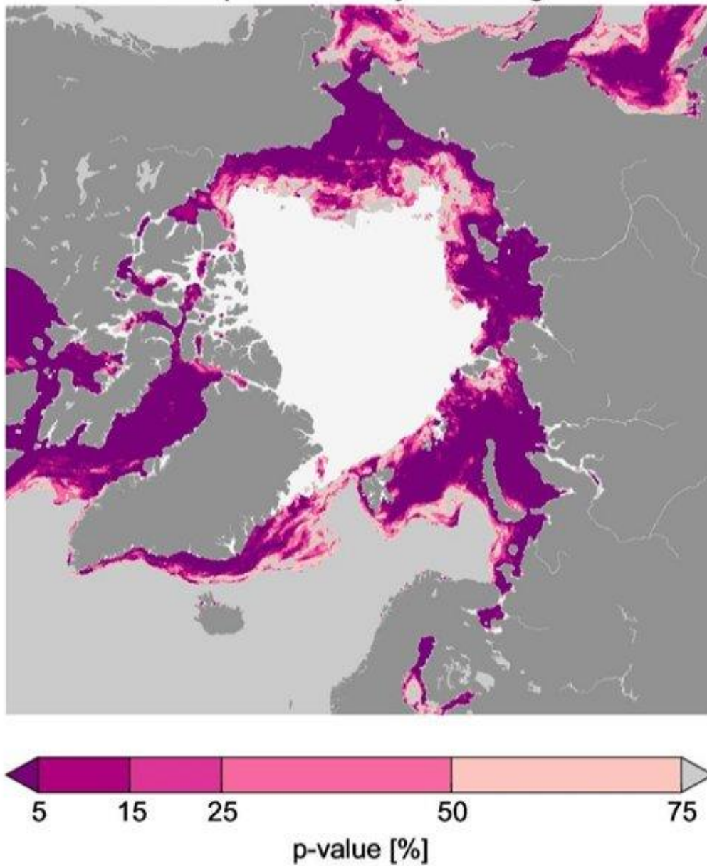
Figure 13. The probability that the trend in Figure 12 is not significant (test of the null-hypothesis). A low value (< 5 %) indicates that the trend is significant.
