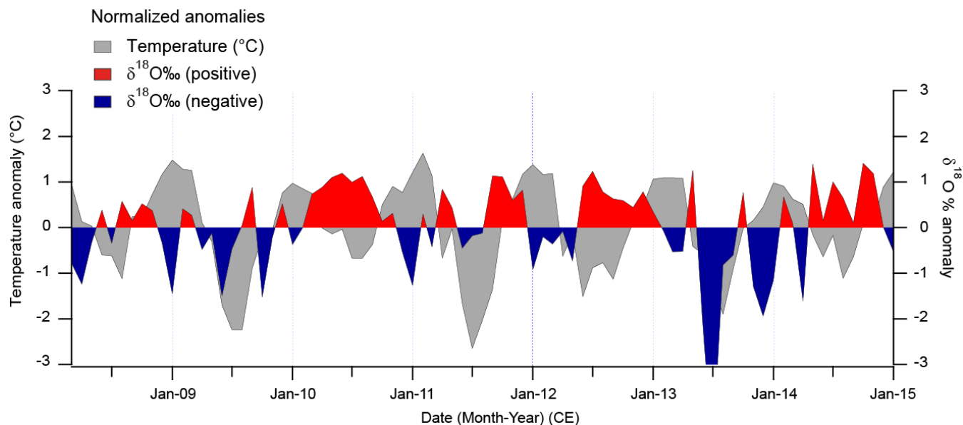
Figure 10: Standardized anomalies for air temperatures (solid grey colours) registered at Bellingshausen Station (BE) on King George Island and a composite \delta^{18}\text{O} time series derived from firm cores OH-6, OH-9 and OH-10 from Laclavere Plateau (LCL). Both time series were detrended prior to constructing the time series of anomalies.
