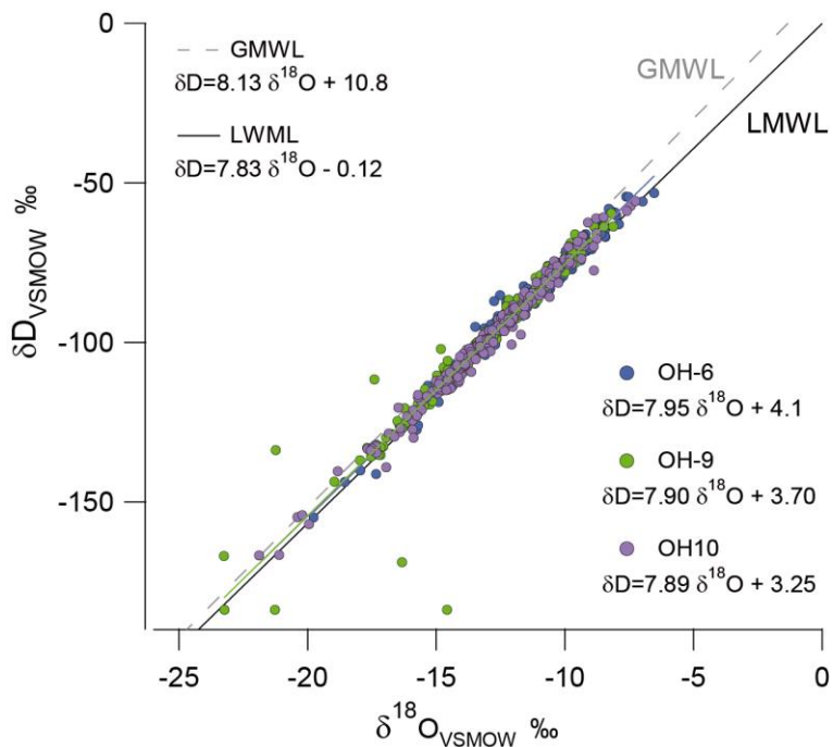
5 Figure 9: Co-isotopic relationship of firm cores OH-6 (solid blue dots), OH-9 (solid green dots) and OH-10 (solid purple dots). All slopes and intercepts are very close to each other as well as to the global and local meteoric water line (GMWL – grey dashed line, and LMWL – black solid line, respectively). Stable water isotope analysis for each firm core was made at 5cm resolution, representing 630 samples in total.
