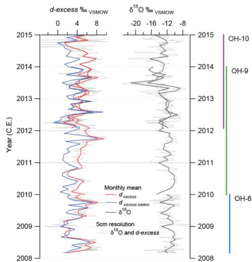
Figure 3: Time series for firn cores OH-6 (light blue line right), OH-9 (green line right) and OH-10 (purple line right) derived for \delta^{18}\text{O} (black line right) and d_{\text{excess}} (red line left) records using a theoretical d_{\text{excess}} ( d_{\text{excess meteo}} ) value (blue line left). The d_{\text{excess meteo}} is calculated from Sea surface temperature (SST) and Relative Humidity ( rh ) according to Uemura et al. (2008). All three cores are located at the same location within the GPS navigator horizontal error ( <10\text{m} ).
