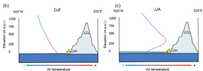
Figure 144: (a) Schematic chart showing the orographic barrier effect of the AP on the stable water isotope depletion and accumulation rate at different altitudes, firn core locations (OH-4, OH-5 and OH-6) and distances from the coast (OH); (b) temperature gradient (adiabatic cooling) during DJF (summer) and sea-ice-free conditions; (c) inversion layer in the lower troposphere during sea-ice-covered conditions in JJA (winter).
