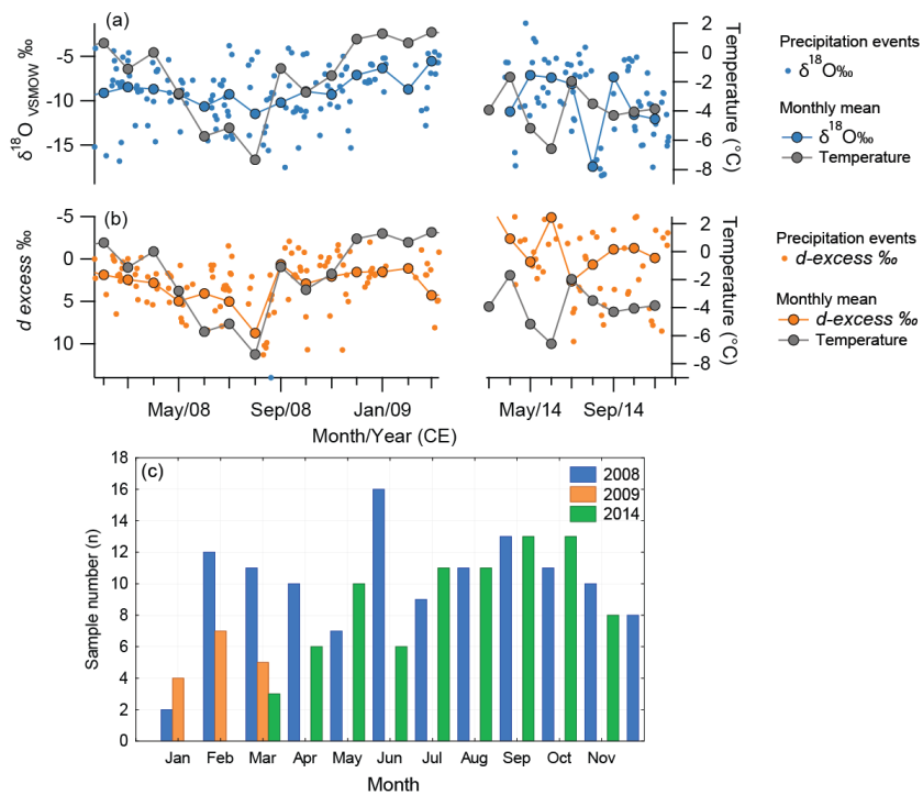
Figure 46: Stable water isotope composition of precipitation events and air temperature at O'Higgins Station. (a) shows the \delta^{18}\text{O} composition of precipitation of single daily events (small solid blue dots) and monthly means (big solid blue dots and line) and (b) deuterium excess ( d_{\text{excess}} ) of single daily events (small orange dots) and monthly means (big orange dots and line). In both (a) and (b) monthly mean air temperature is also shown (grey solid dots and line). (c) Histogram showing the monthly distribution of precipitation samples (n) collected at O'Higgins Station in 2008, 2009 and 2014
