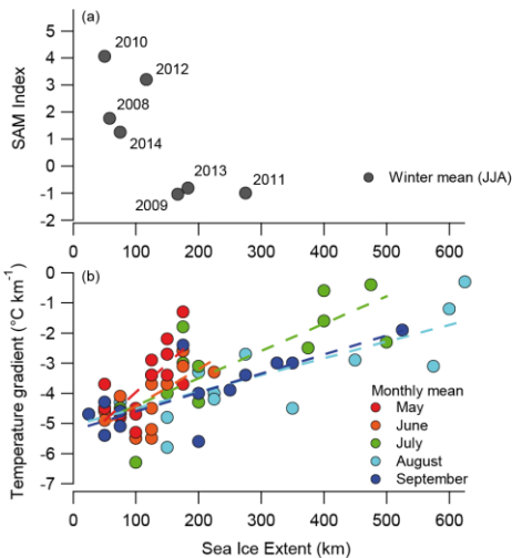
Figure 1143: Sea ice extent (SIE) from O'Higgins Station (OH) and its relationship to (a) the Southern Annular Mode and (b) to the temperature gradient between sea level and 1100 m a.s.l. at the Laclavere Plateau (LCL). SIE data is from the National Snow & Ice Data Center data set (NSIDC). Sea ice extent, defined as the extension of the sea region covered for at least 15% of ice, exhibits a negative relationship to the Southern Annular Mode between 2008 and 2014. The relationship to the temperature gradient is positive. A decreasing seasonal pattern of the temperature gradient can be observed from May to September (1979 – 1996).
