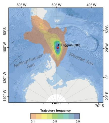
Figure 57: Frequency distribution map of the main transport paths of air masses approaching the northern Antarctic Peninsula (AP). Translucent red colours represent the lowest frequency and blue colours the higher frequency. In general most of the air masses arriving at the AP are coming from the Bellingshausen Sea and the South Pacific Ocean.
