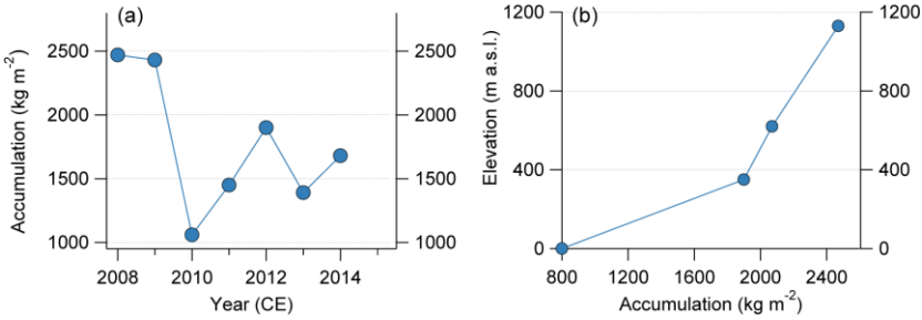
Figure 1345: (a) Accumulation rates for Plateau Laclavere during 2008 – 2014 estimated from the stable water isotope composition of fim cores OH-6, OH-9 and OH-10 and their respective density profiles. (b) Accumulation variability for the west flank of the northern Antarctic Peninsula from the coast to Laclavere Plateau. Accumulation rates were derived from precipitation at O'Higgins Station at sea level and fim cores (OH-4, OH-5 and OH-6) for higher altitudes.
