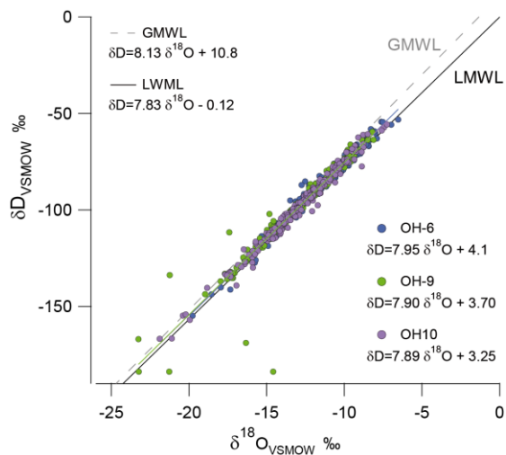
Figure 810: Co-isotopic relationship of firn cores OH-6 (solid blue dots), OH-9 (solid green dots) and OH-10 (solid purple dots). All slopes and intercepts are very close to each other as well as to the global and local meteoric water line (GMWL – grey dashed line, and LMWL – black solid line, respectively). Stable water isotope analysis for each firn core was made at 5cm resolution, representing 630 samples in total.
