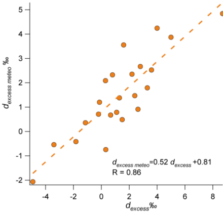
Figure 79: Correlation between monthly mean deuterium excess values ( d_{excess} ) from precipitation samples and theoretical deuterium excess values calculated from meteorological parameters of the moisture source region ( d_{excess\ meteo} ) according to Uemura et al. (2008).
