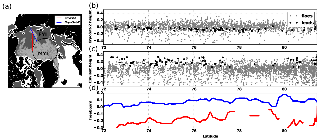
Figure 3. (a) Map of the Envisat (red) and CryoSat-2 (blue) tracks (both monitored on the 24 February 2011) selected for the along-track analysis of the radar freeboard. The light shading shows MYI regions (defined as sea ice with a MYI fraction above 0.7) and the dark gray shading shows FYI regions (defined as sea ice with a MYI below 0.7). (b) CryoSat-2 and (c) Envisat leads (gray dots) and ice floes (black dots) surface elevation corresponding to the tracks shown in (a). (d) Envisat (red) and CryoSat-2 (blue) freeboard corresponding to the tracks shown in (a).
