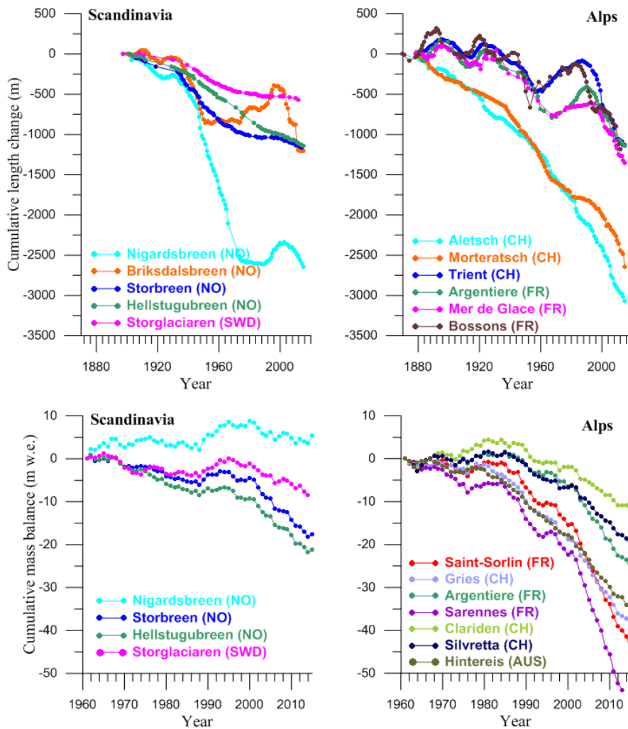
Figure 2: Length and surface mass balance changes documented with in-situ measurements for glaciers in Scandinavia and in the European Alps. Sources: WGMS (2015) and earlier in-situ with updates (Andreassen et al., 2016).
