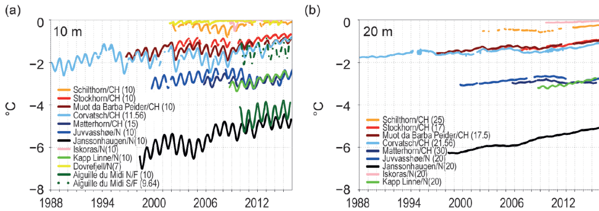
Figure 3: Temperature evolution of mountain permafrost in Norway (N), France (F), and Switzerland (CH) measured in boreholes at (a) 10 m and (b) 20 m depth (exact depth given in parenthesis). Figure adapted from Noetzli et al. (2016).
