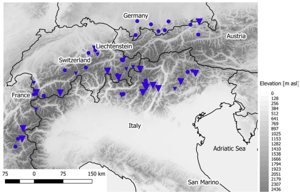
5 Figure 1: Geographical distribution of the 45 year trend (1968-2012) for April 1 th SWE in the Alps. All stations show a negative trend. Large triangles indicate significant trends ( p = 0.05 ) and small triangles indicate weakly significant trends ( p = 0.2 ). Circles represent stations with no significant trend ( p = 0.2 ). The elevation is given in gray. (Adapted from Marty et al. 2017b)
