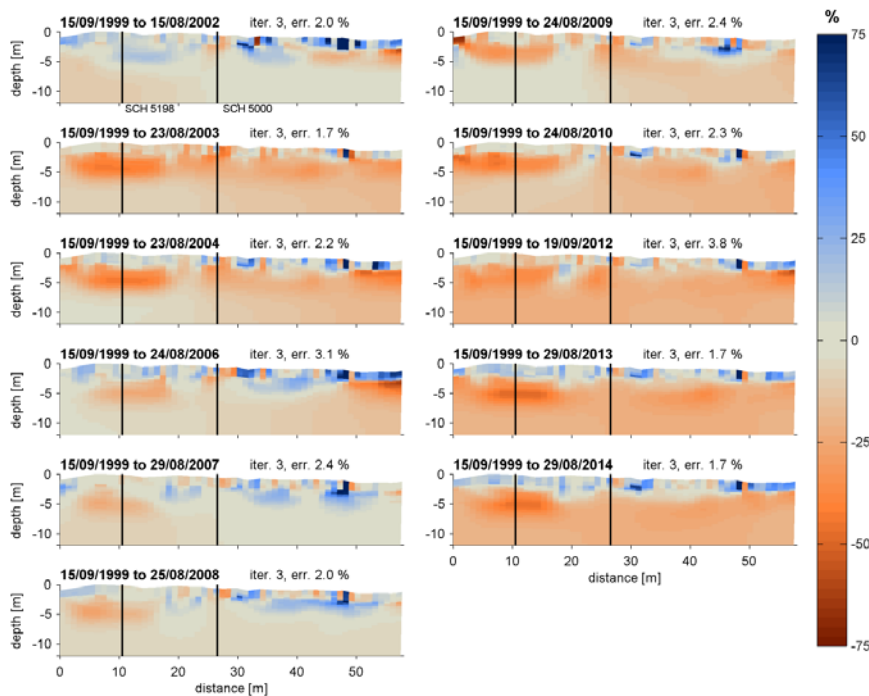
Figure 4: 15-year change in specific electrical resistivity (given as % specific resistivity change) along a 2-dimensional Electrical Resistivity Tomography (ERT) profile at Schilthorn, Swiss Alps (2900 m a.s.l.). Red colors denote a resistivity decrease corresponding to loss of ground ice with respect to the initial measurement in 1999 (see Hilbich et al. 2008a, 2011 for more details on ERT monitoring in permafrost). The black vertical lines denote borehole locations. (modified after Permos, 2016)
