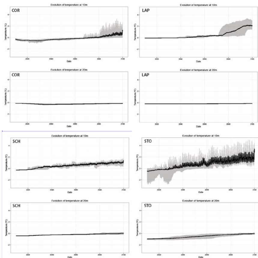
Figure 5: Modelled long-term evolution of ground temperatures at 10 m and 20 m at four different permafrost sites in the Swiss Alps (COR: Murtèl-Corvatsch, LAP: Lapires, SCH: Schilthorn, STO: Stockhorn), as simulated with the COUP model (Marmy et al., 2016). The black lines represent the median scenario and the grey zone the range of the 13 GCM/RCM chains which were used to drive the simulations. Modified after Marmy et al. (2016).
