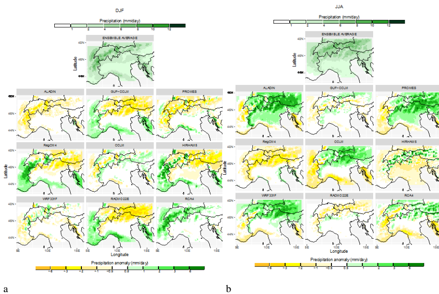
Figure 10: DJF (a) and JJA (b) precipitation as derived from 9 regional climate models. The average of the model ensemble is 5 shown in the top panel at the center.
