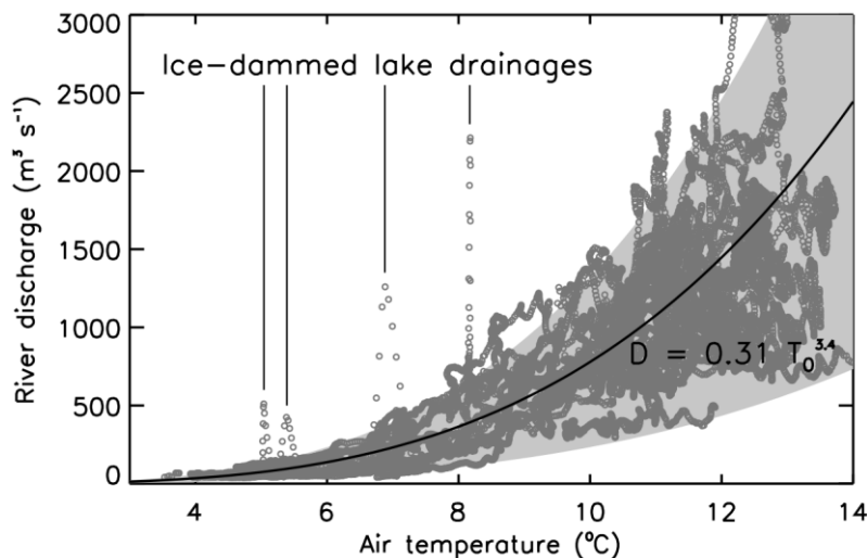
Figure 4: Hourly values of river discharge versus air temperature in Kangerlussuaq for July-September data 2008-2015 (dark grey). The solid line denotes a power-function fit to the data, with the light grey area the 70% uncertainty range. Ice-dammed lake drainages (“jökulhlaups”) stand out as spikes.
