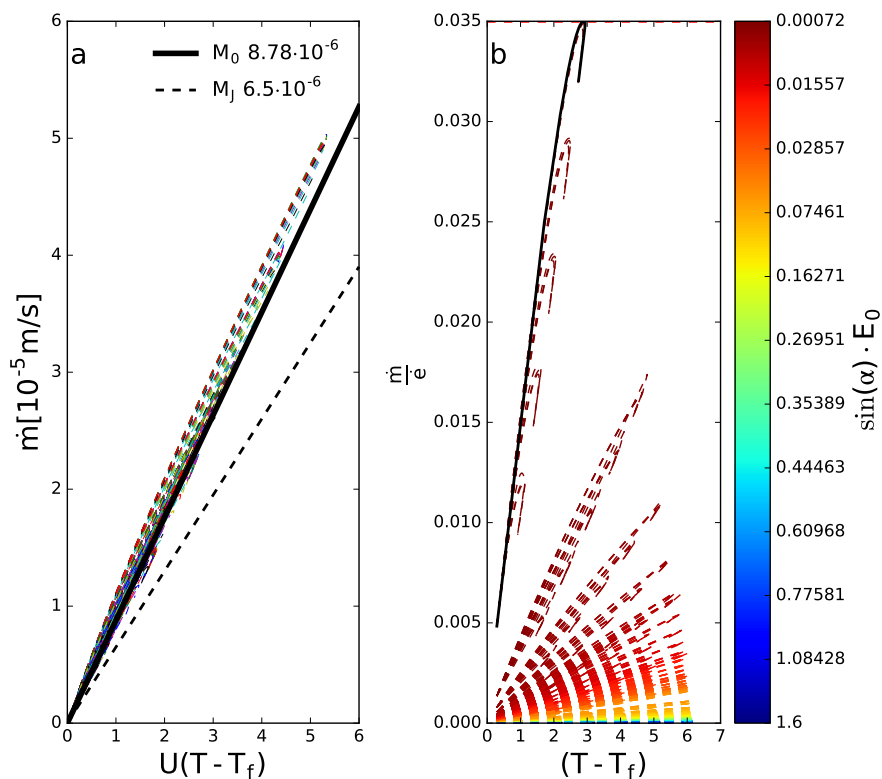
Figure 1.20. Investigation of melting proportion in the plume equations for different LP experiments. The plume model was run in a well mixed environment for different parameter settings: E_0[0.036 - 0.16] , \sin(\alpha)[0.02 - 1] , q_{sq}[10^{-5} - 0.1 \frac{\text{m}^2}{\text{s}}] , T_a[0 - 4]^\circ\text{C} . Panel a) shows the melt rate as a function of plume velocity U and plume temperature T and its freezing temperature T_f ( \dot{m} = M_0(T - T_f)U ). The second panel illustrates that \dot{m} \ll \dot{e} in this parameter range, but being biggest for long floating tongues.
