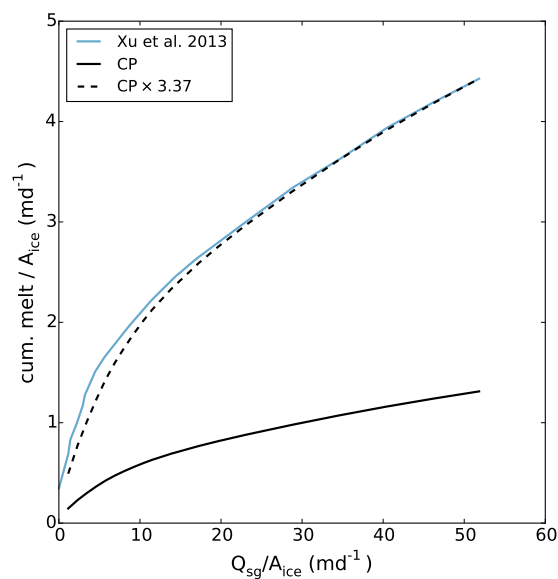
Figure 14. Average melt rate over a 150 m wide and 500 m deep glacier part as a function of discharge localized in one channel. Following Xu et al. (2013), for the x-axis, the discharge Q_{sg} was divided by the area of the ice face A_{ice} = 150 * 500 \text{ m}^2 so that q_{sg} = 50 \text{ md}^{-1} corresponds Q_{sg} = 43.4 \text{ m}^3 \text{ s}^{-1} . The numerical results of Xu et al. (2013) are displayed with the blue line. Taking the same conditions ( T_a , S_a , Q_{sg} ) and an entrainment factor of E_0 = 0.1 the CP model gives the solid black line. To match the experiment a scaling factor of 3.40 is needed (black, dashed line).
