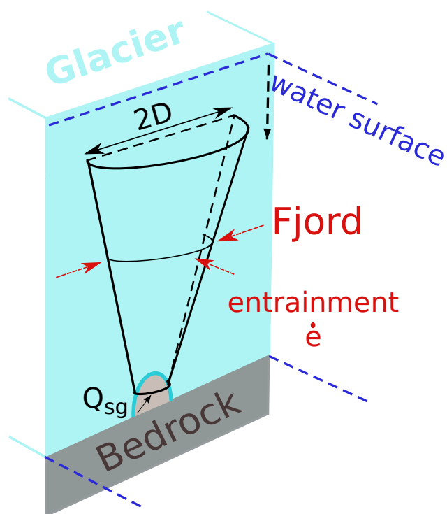
Figure 2. Conceptual scheme of two-dimensional CP model modified after Jenkins (1991) and Cowton et al. (2015). Subglacial discharge enters the fjord localized, via a channel. The plume geometry is described as a half cone and the entrainment occurs around the arc. The subglacial discharge is Q_{sg} = \frac{D_0^2 U_0 \pi}{2} where D_0 is the initial radius and U_0 is the initial velocity.
