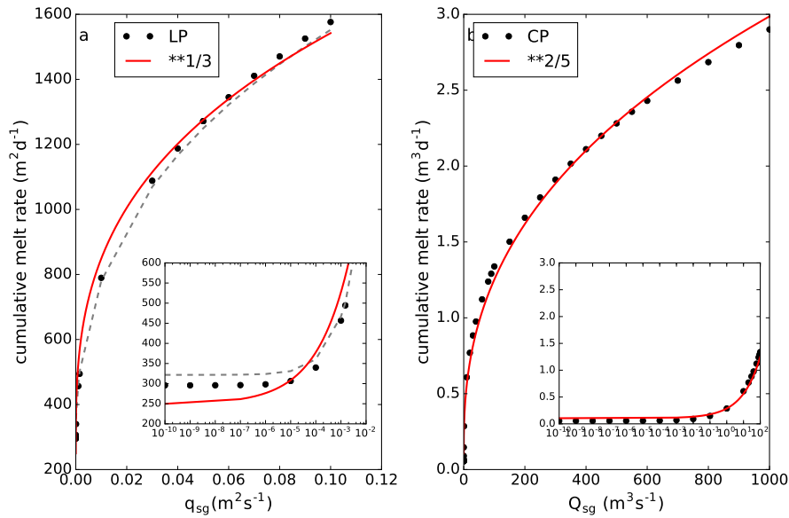
Figure 9. Cumulative melt rate of the LP model (a) and CP model (b) for E_0 = 0.1 with different discharge values for a well-mixed environment with T_a = 4^\circ\text{C} and S_a = 34.65 psu. For the LP (a) red line corresponds \dot{m} = 6.6 \cdot 10^{-5} \cdot Q_{sg}^{\frac{1}{3}} + 6.0 \cdot 10^{-6} . For the CP (b) the red line corresponds to \dot{m} = 0.19 \cdot Q_{sg}^{\frac{2}{5}} + 0.09 . The inset presents the melt rate for small discharges on logarithmic scale. The grey dashed line (a) is our analytical solution for the cumulative melt rate of the LP model (Eq. A20)
