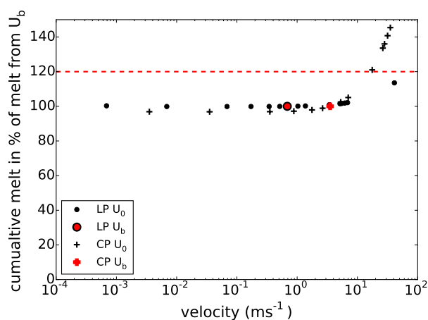
Figure 4. Sensitivity of cumulative melt rate to different initial velocities, for both plume models. Melt rate (black) is in percent of the cumulative melt achieved with initial balance velocity U_b (red). Red dashed line shows 120 % mark. Only very high initial velocities can for the CP model appreciably increase the cumulative melt rate.
