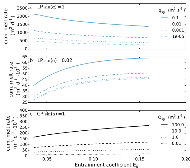
Figure 6. Cumulative melt rates of the different plume models as a function of the entrainment rate factor E_0 for four different discharge values. The cumulative melt rate is depicted for a) LP of a tidewater glacier ( \sin(\alpha) = 1 ), b) LP of a long floating tongue and c) CP of a tidewater glacier. For the LP model for \sin(\alpha) = 1 a higher E_0 leads to lower cumulative melting opposite to the other two cases.
