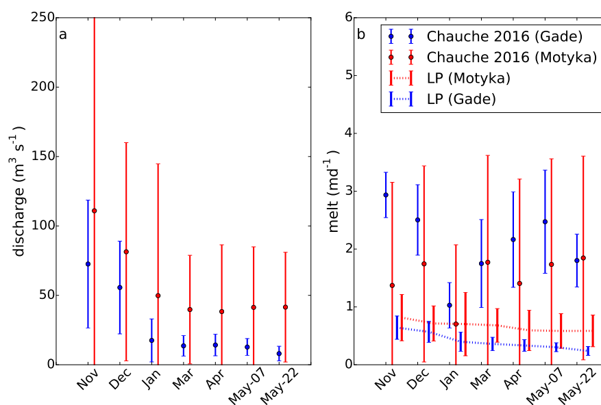
Figure 19. a) Estimated subglacial discharge of Store Glacier for winter 2012/2013 in from (Chauche, 2016). Red ranges give subglacial discharge estimates by the Motyka model and blue ranges by the Gade model and b) the corresponding melt rate profiles. Simulated melt rates by the LP model with E_0=0.036 are depicted in the red dotted (subglacial discharge from Moytka model) and blue dotted (subglacial discharge from Gade model.)
