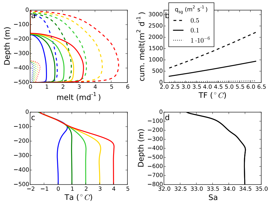
Figure 11. Influence of stratification and discharge on the melt rate profile of the LP (a). The three different discharge values ( q_{sg} = 0.5, 0.1, 10^{-6} \text{ m}^2 \text{ s}^{-1} , dashed, solid, dotted) in a stratified environment for a fixed salinity profile (d) and 5 different temperature profiles (c) result in 15 different melt rate profiles. The melt rate of the corresponding temperature profile is displayed in the same color as well as in the same style (dashed, dotted or solid) for the corresponding discharge. Note that a very high discharge ( q_{sg} = 0.5 \text{ m}^2 \text{ s}^{-1} ) is needed for the plume to reach the surface. For each discharge value the corresponding cumulative melt rate is depicted (b) as a function of the thermal forcing ( TF = T_a - T_b , eq. 7) at the grounding line. For \dot{m} \sim TF^{\beta} we found \beta values of 1.2 for ( q_{sg} = 0.5 \text{ m}^2 \text{ s}^{-1} ), 1.2 for ( q_{sg} = 0.1 \text{ m}^2 \text{ s}^{-1} ) and 1.4 for ( q_{sg} = 10^{-6} \text{ m}^2 \text{ s}^{-1} ).
