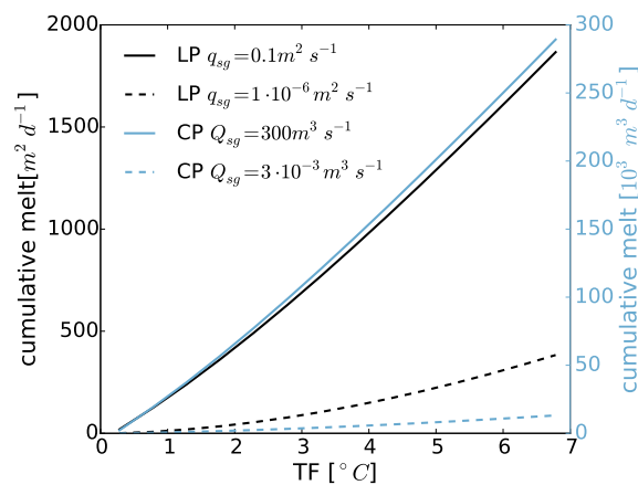
Figure 10. Cumulative melt rate for the LP model (black) and CP (blue) model as a function of the ambient temperature T_a for high (solid lines) and low (dashed lines) discharge values. The experiment is for a well-mixed, 500m deep tidewater glacier ( \sin(\alpha) = 1 ), with S_a = 34 psu and E_0 = 0.1 .
