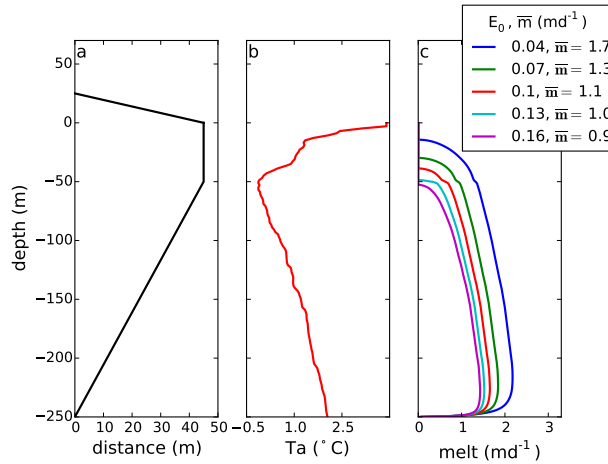
Figure 17. Kangerlussuup Sermia average undercut profile at the terminus (a) with the assumed temperature profile (b) give different melt rate profiles (c) simulated for different E_0 and same Q_{sg} = 208 \text{ m}^3 \text{ s}^{-1} . All average melt rates are below the determined 2 \text{ md}^{-1} by Fried et al. (2015).
