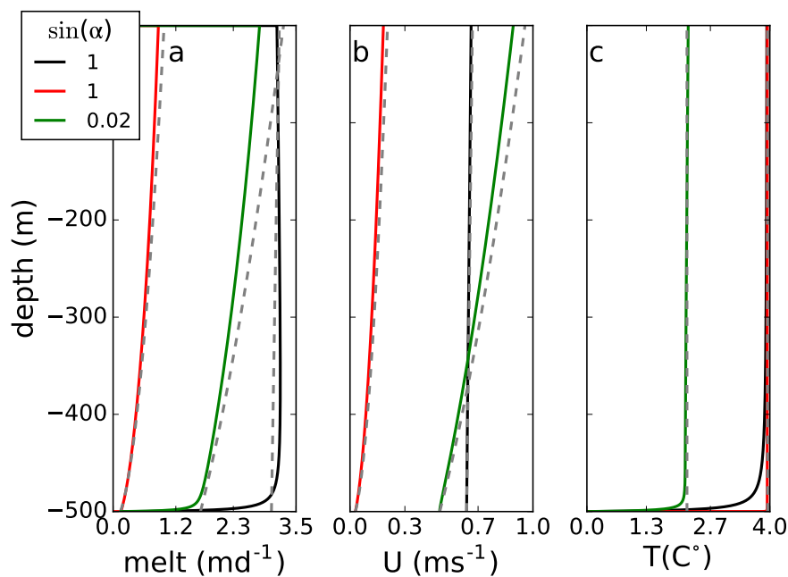
Figure 1.23. Evolution of m (a), U (b) and T (c) along Z for the tidewater glaciers with high discharge ( q_{sg} = 0.1 \frac{m^2}{s} , black line), low discharge ( q_{sg} = 10^{-5} \frac{m^2}{s} , red line) and a floating tongue glacier ( q_{sg} = 0.1 \frac{m^2}{s} , green line). The corresponding approximations of m_* = M_0 U_* \Delta T_* , U_* (A13), T_* (A9) (grey, dashed line) show high similarities.
