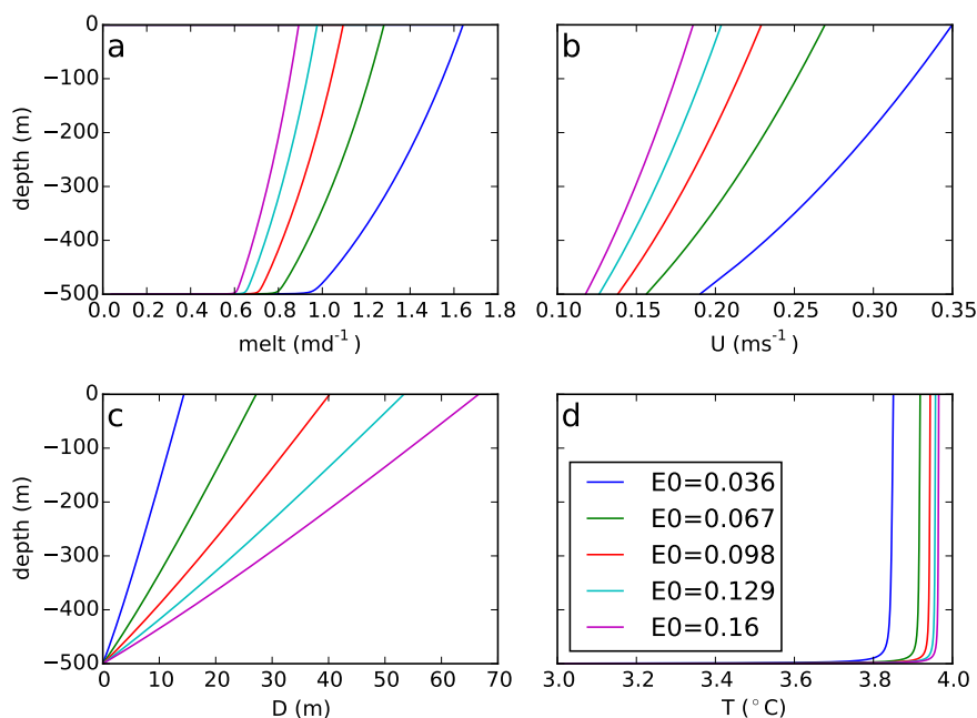
Figure 7. a) melt rate profile of a plume and its b) velocity, c) thickness and d) temperature computed with the LP model with a discharge q_{sg} = 10^{-3} \text{ m}^2 \text{ s}^{-1} for different E_0 . Higher E_0 leads to lower melting and slower velocity (b) but thicker (c) and warmer (d) plumes.
