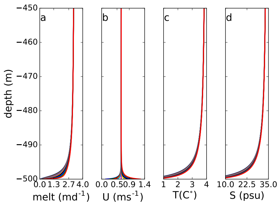
Figure 1.21. Convergence of melt rate (a), velocity (b), temperature (c) and salinity (d) within the first 50 meter of the LP.
