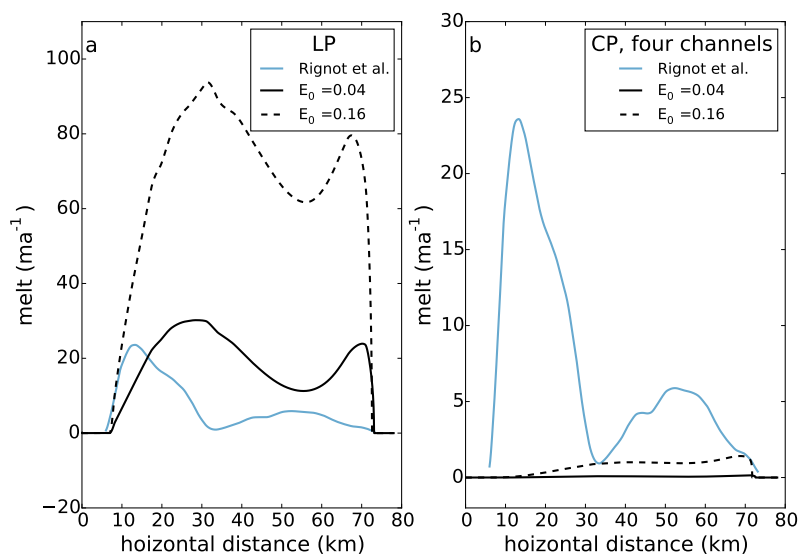
Figure 16. Melt rate of a) LP model simulated over the long floating tongue of Petermann glacier with a minimal discharge of Q_{min} = 10^{-5} \text{ m}^2 \text{ s}^{-1} for the minimal ( E_0 = 0.036 ) and maximal ( E_0 = 0.16 ) value (black lines) of the entrainment parameter. In panel b) we used the maximum discharge Q_{sg} = 296 \text{ m}^3 \text{ s}^{-1} (total runoff assumed only in summer) distributed over four channels to compute the melt rate with the CP model. As forcing variables we used the fjord's temperature and salinity profile in front of the floating tongue for the year 2003 summarized by Johnson et al. (2011a) and from Morlighem et al. (2014) we determined the glacier thickness and depth of the floating tongue (see 5.1 for details). For both E_0 the melt rate is highly overestimated with the LP model and underestimated with the CP model. The empirical melt rate estimated by Rignot and Steffen (2008) is displayed with the blue line. Note the different vertical scale on the panels.
