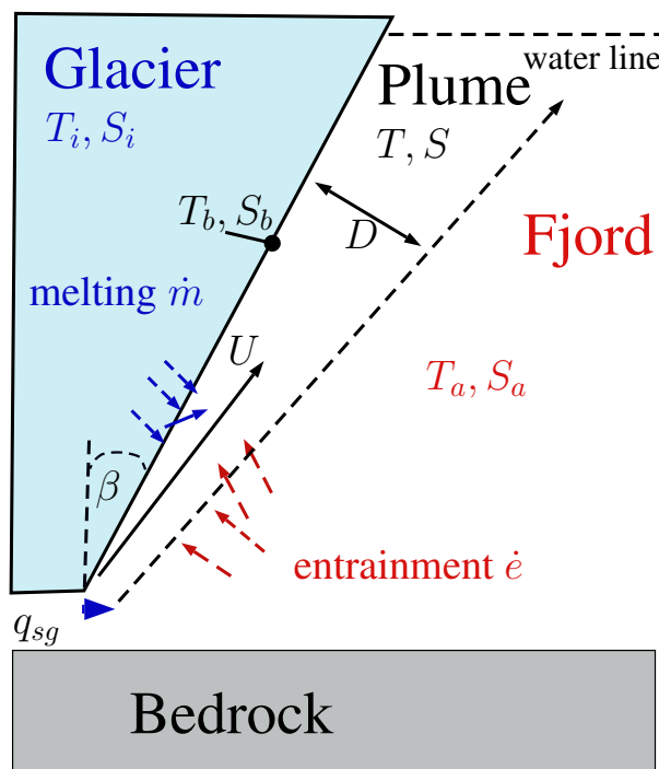
Figure 1. Conceptual scheme of 1D plume model after Jenkins (2011). Uniformly distributed along the grounding line subglacial freshwater flux q_{sg} , enters the fjord and forms a plume that rises up due to buoyancy. The plume is described explicitly with its temperature T , salinity S , thickness D and velocity U . The plume rises along the ice shelf an slope \alpha = 90^\circ - \beta until it either reaches the water surface or has zero velocity due to the loss its buoyancy. The ambient water with salinity S_a and temperature T_a entrains into the plume with an entrainment rate \dot{e} . Melting \dot{m} occurs on the glacier front and adds to the plume buoyancy with water of the temperature T_b and salinity S_b .
