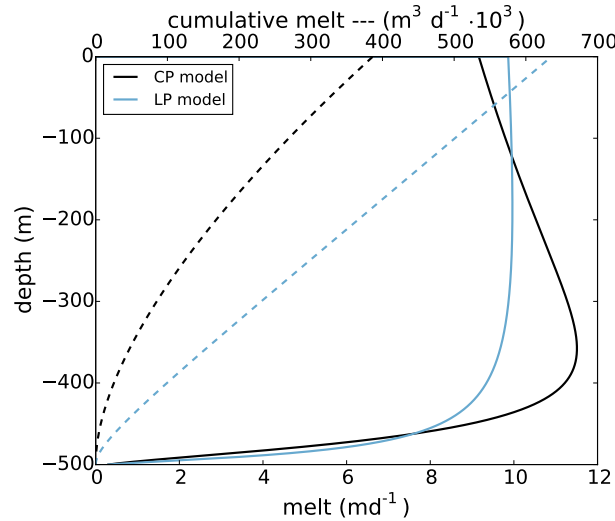
Figure 5. Melt rate profiles in a well-mixed fjord simulated by the CP model (black) and LP model (blue) for a width W = 150 m and the total discharge of Q_{sg} = 500 \text{ m}^3 \text{ s}^{-1} . In the case of the CP model the total discharge occur through one channel in the center of the glacier, in the case of LP model the discharge is uniformly distributed with the rate q_{sg} = \frac{Q_{sg}}{W} = 3.6 \text{ m}^2 \text{ s}^{-1} . Both plumes start with a velocity of U_0 = 1 \frac{\text{m}}{\text{s}} . Solid lines show melt rate averaged acrosss the plume in the case of CP model and over entire glacier in the case of LP model. The dashed lines shows the corresponding cumulative melt rate for the entire glacier.
