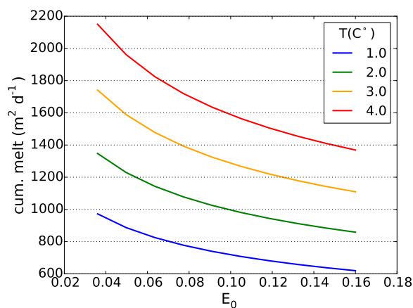
Figure 8. cumulative melt rate in dependence of the entrainment E_0 for q_{sg} = 10^{-3} \text{ m}^2 \text{ s}^{-1} in four different well mixed ambient Temperatures ( T_a )
